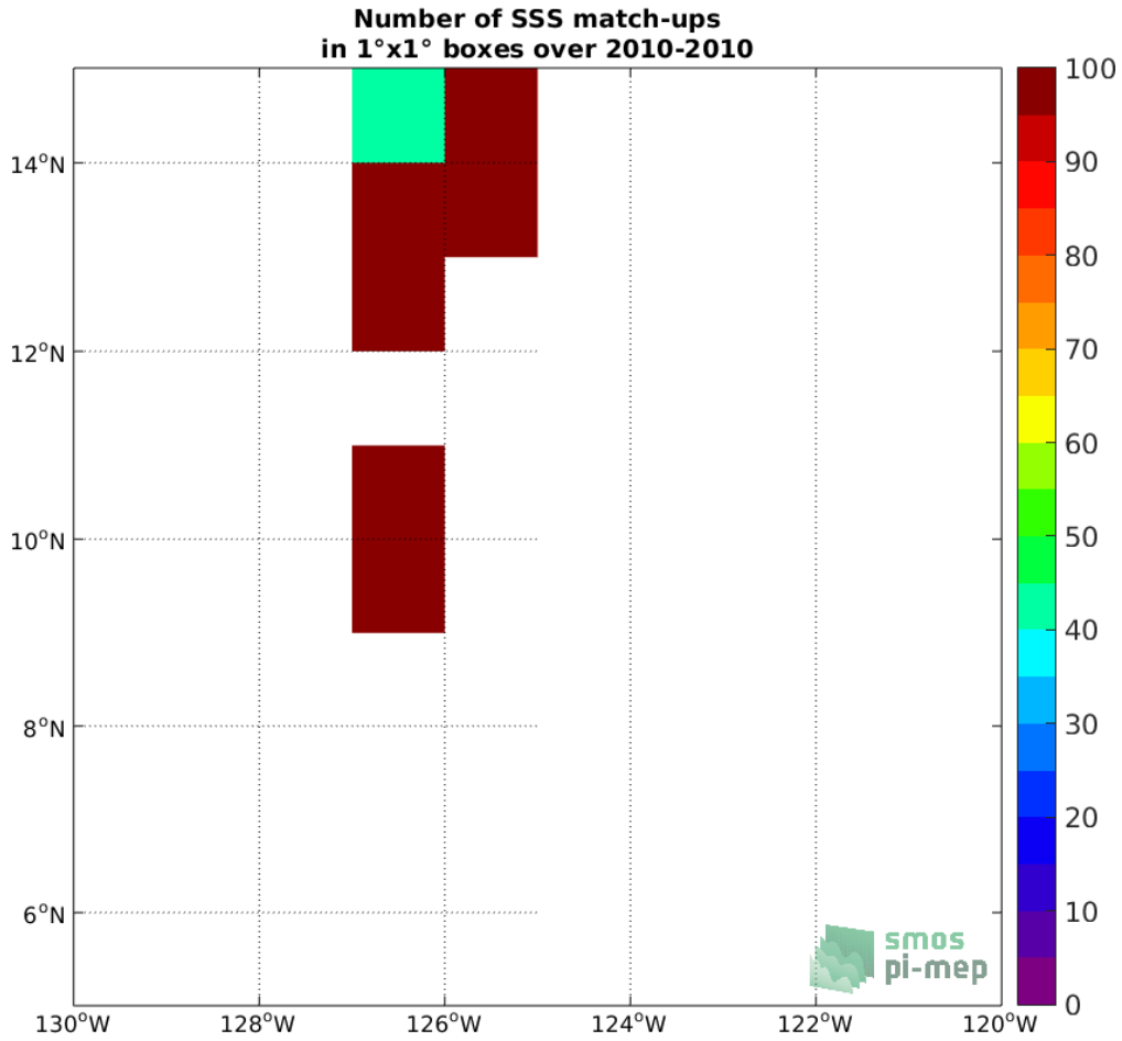
Figure 4: Number of SSS match-ups between TSG (GOSUD-Sailing-ship) SSS and the SMOS SSS L2 v700 (ESA) SSS product for the SPURS 2 Pi-MEP region over 1^\circ \times 1^\circ boxes and for the full satellite product period.
