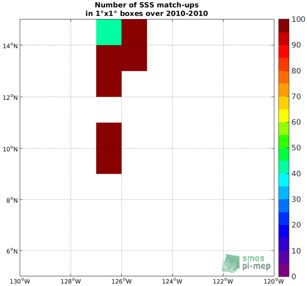
Figure 4: Number of SSS match-ups between TSG (GOSUD-Sailing-ship) SSS and the SMOS SSS L2 v700 (ESA) SSS product for the SPURS 2 Pi-MEP region over 1°x1° boxes and for the full satellite product period.
