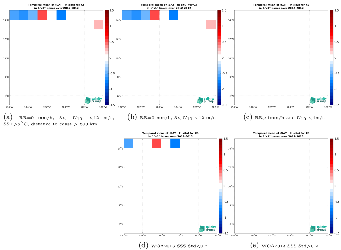
Figure 14: Temporal mean gridded over spatial boxes of size 1^\circ \times 1^\circ of \Delta\text{SSS} (SMOS SSS L2 v700 (ESA) - TSG (GOSUD-Research-vessel)) for 5 different subdatasets corresponding to:RR=0 mm/h, 3 < U_{10} < 12 m/s, SST > 5°C, distance to coast > 800 km (a), RR=0 mm/h, 3 < U_{10} < 12 m/s (b), RR > 1mm/h and U_{10} < 4 m/s (c), WOA2013 SSS Std < 0.2 (d), WOA2013 SSS Std > 0.2 (e).
