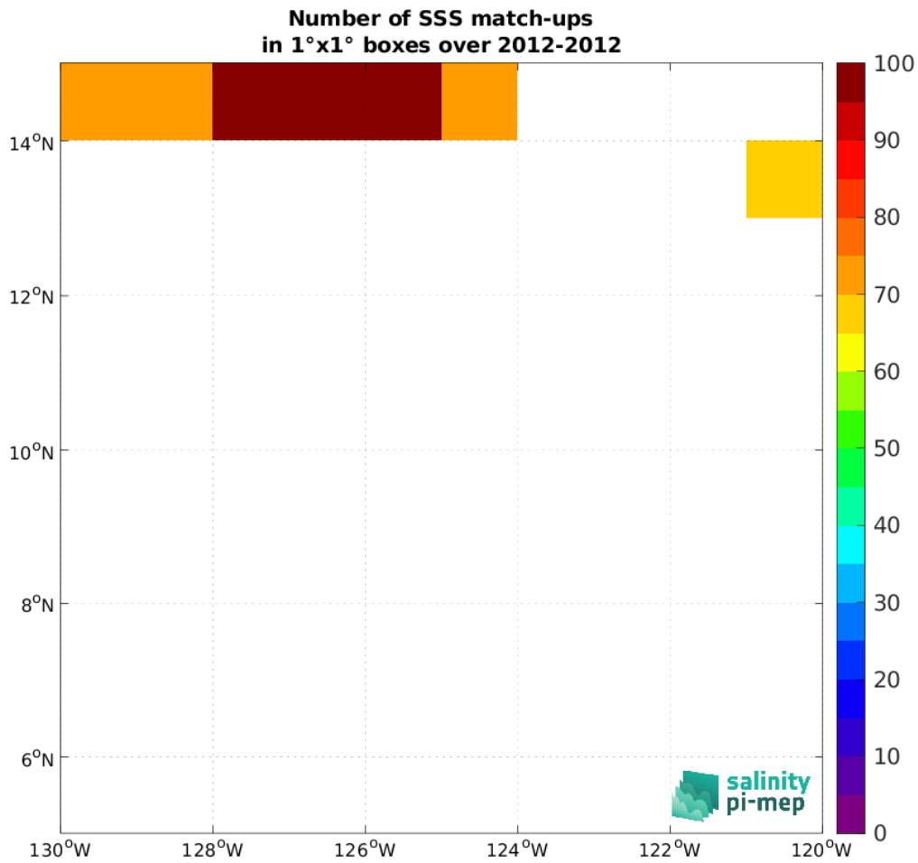
Figure 4: Number of SSS match-ups between TSG (GOSUD-Research-vessel) SSS and the SMOS SSS L2 v700 (ESA) SSS product for the SPURS 2 Pi-MEP region over 1^{\circ} \times 1^{\circ} boxes and for the full satellite product period.
