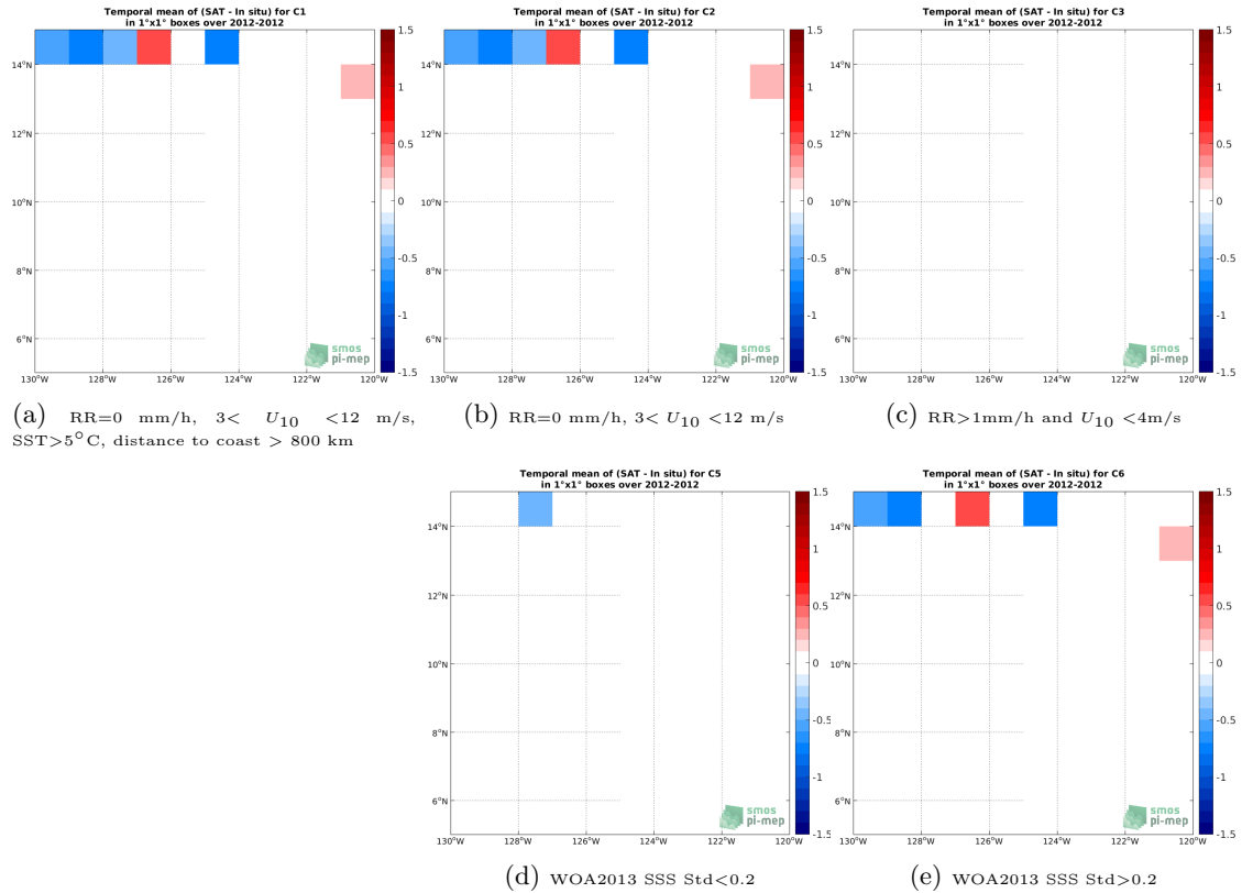
Figure 12: Temporal mean gridded over spatial boxes of size 1^\circ \times 1^\circ of \Delta\text{SSS} (SMOS SSS L2 v700 (ESA) - TSG (GOSUD-Research-vessel)) for 5 different subdatasets corresponding to:RR=0 mm/h, 3 < U_{10} < 12 m/s, SST>5°C, distance to coast > 800 km (a), RR=0 mm/h, 3 < U_{10} < 12 m/s (b), RR>1mm/h and U_{10} < 4 m/s (c), WOA2013 SSS Std<0.2 (d), WOA2013 SSS Std>0.2 (e).
