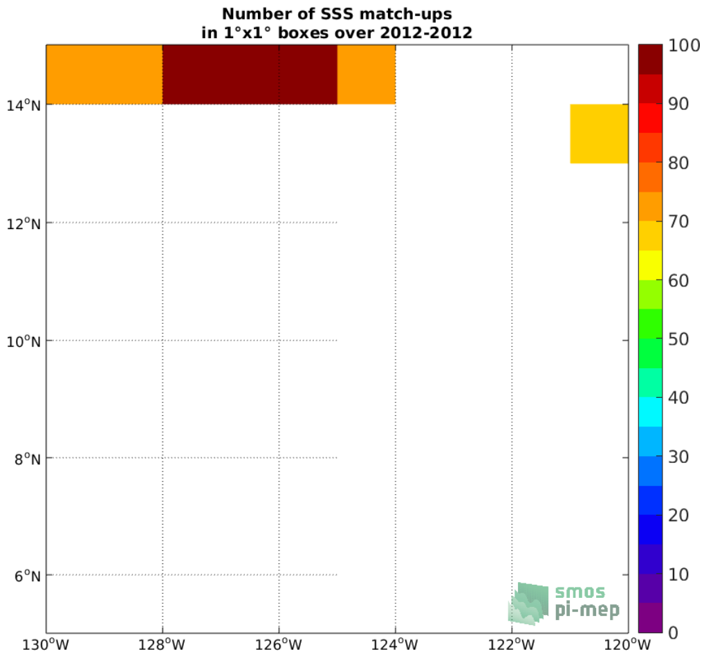
Figure 4: Number of SSS match-ups between TSG (GOSUD-Research-vessel) SSS and the SMOS SSS L2 v700 (ESA) SSS product for the SPURS 2 Pi-MEP region over 1^\circ \times 1^\circ boxes and for the full satellite product period.
