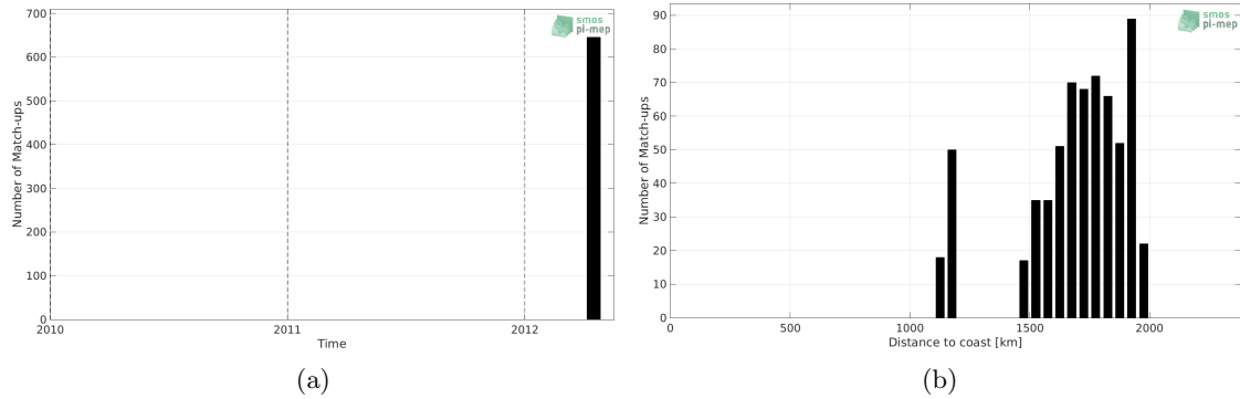
Figure 1: Number of match-ups between TSG (GOSUD-Research-vessel) and SMOS SSS L2 v700 (ESA) SSS as a function of time (a) and as function of the distance to coast (b) over the SPURS 2 Pi-MEP region and for the full satellite product period.
