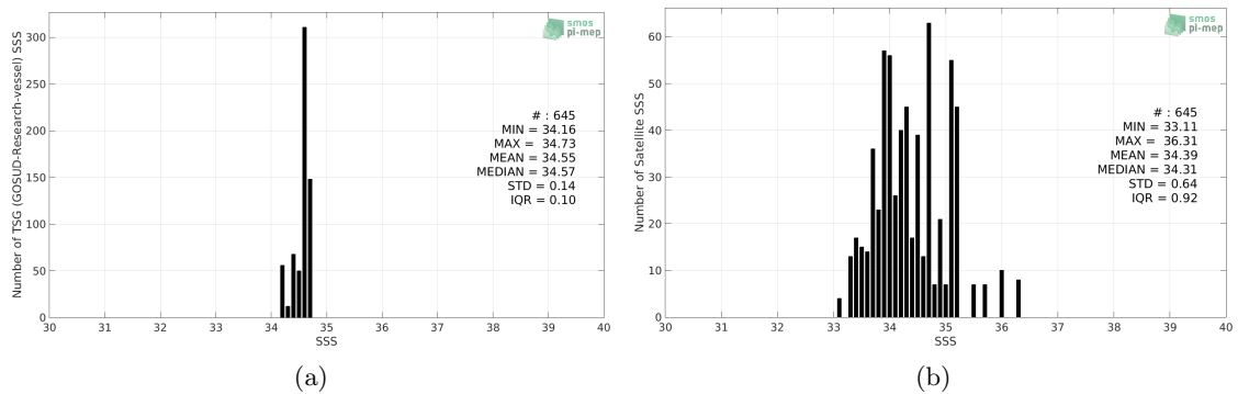
Figure 2: Histograms of SSS from TSG (GOSUD-Research-vessel) (a) and SMOS SSS L2 v700 (ESA) (b) considering all match-up pairs per bins of 0.1 over the SPURS 2 Pi-MEP region and for the full satellite product period.
