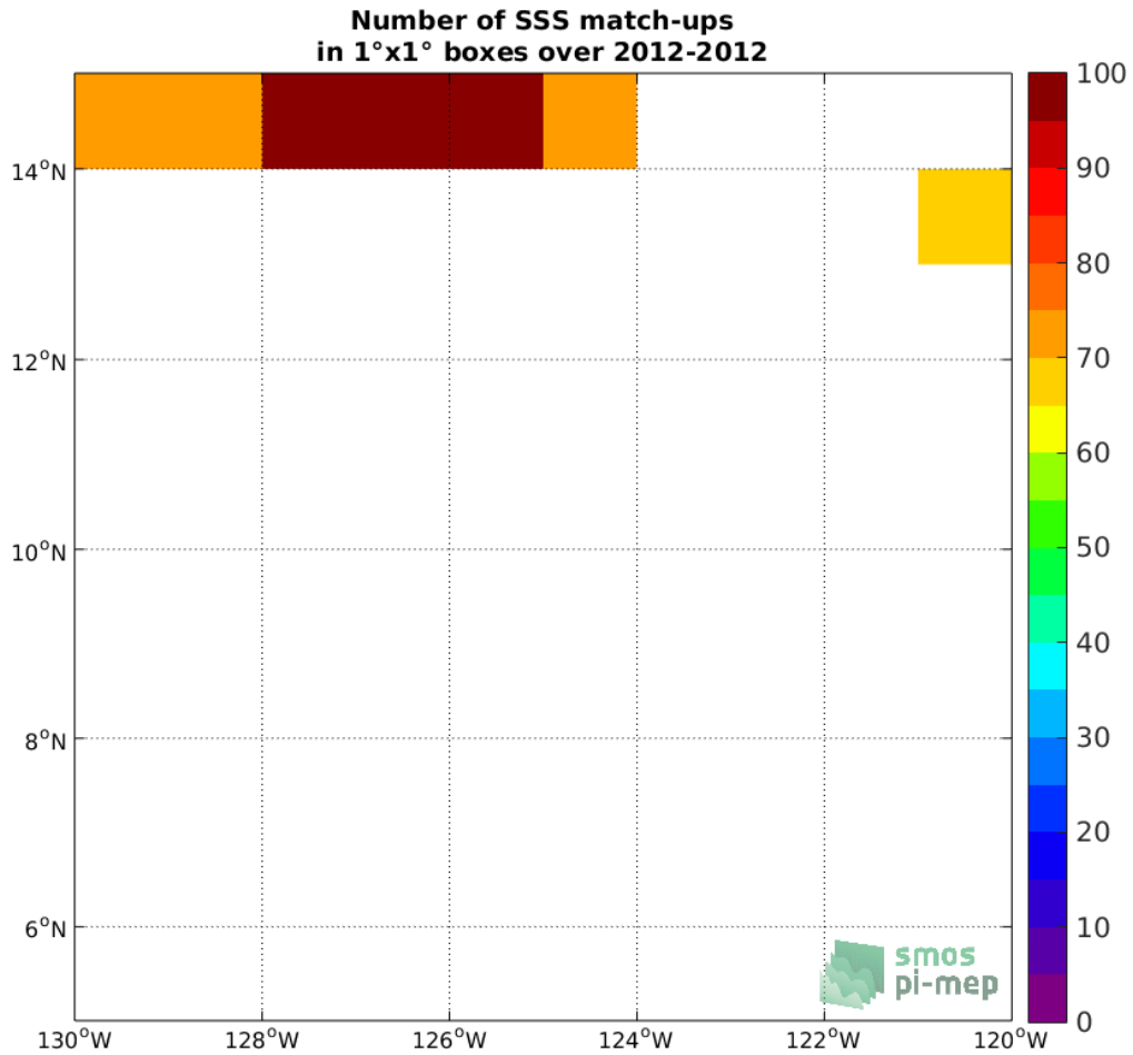
Figure 4: Number of SSS match-ups between TSG (GOSUD-Research-vessel) SSS and the SMOS SSS L2 v700 (ESA) SSS product for the SPURS 2 Pi-MEP region over 1°x1° boxes and for the full satellite product period.
