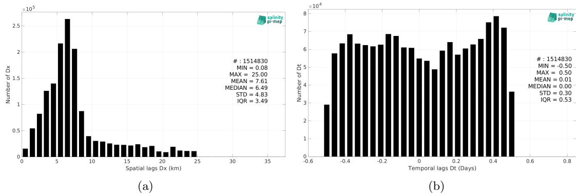
Figure 6: Histograms of the spatial (a) and temporal (b) lags between the location/time of the Salinity Snake (SPURS 2) measurement and the date of the corresponding SMOS SSS L2 v700 (ESA) SSS pixel.
