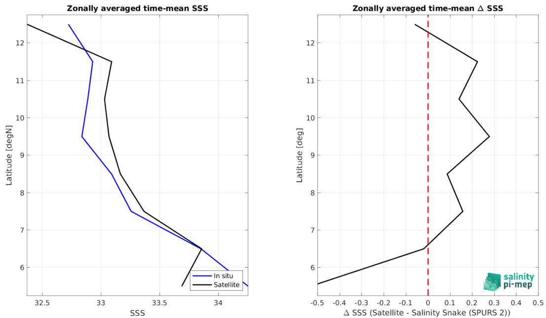
Figure 9: Left panel: Zonal mean SSS from SMOS SSS L2 v700 (ESA) satellite product (black) and from Salinity Snake (SPURS 2) (blue). Right panel: Zonal mean of \Delta SSS (Satellite - Salinity Snake (SPURS 2)) for all the collected Pi-MEP match-up pairs estimated over the full satellite product period.
