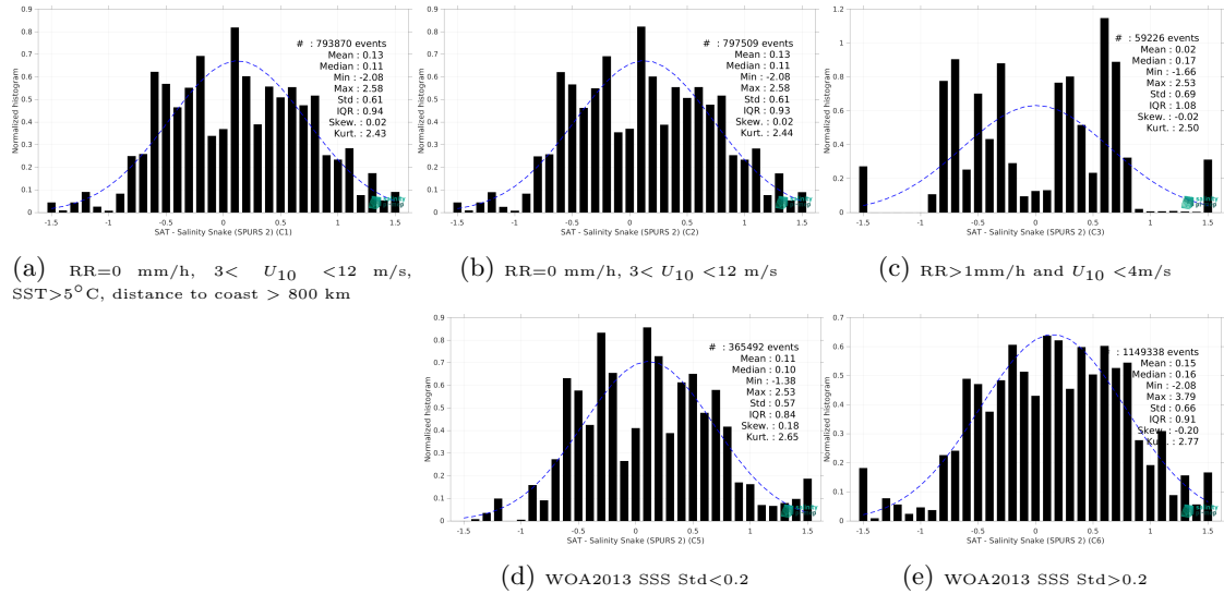
Figure 15: Normalized histogram of \Delta SSS (SMOS SSS L2 v700 (ESA) - Salinity Snake (SPURS 2)) for 5 different subdatasets corresponding to: RR=0 mm/h, 3 < U_{10} < 12 m/s, SST>5°C, distance to coast > 800 km (a), RR=0 mm/h, 3 < U_{10} < 12 m/s (b), RR>1mm/h and U_{10} < 4 m/s (c), WOA2013 SSS Std<0.2 (d), WOA2013 SSS Std>0.2 (e).
