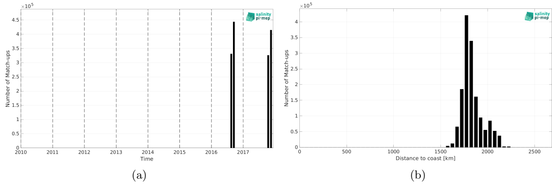
Figure 2: Number of match-ups between Salinity Snake (SPURS 2) and SMOS SSS L2 v700 (ESA) SSS as a function of time (a) and as function of the distance to coast (b) over the SPURS 2 Pi-MEP region and for the full satellite product period.
