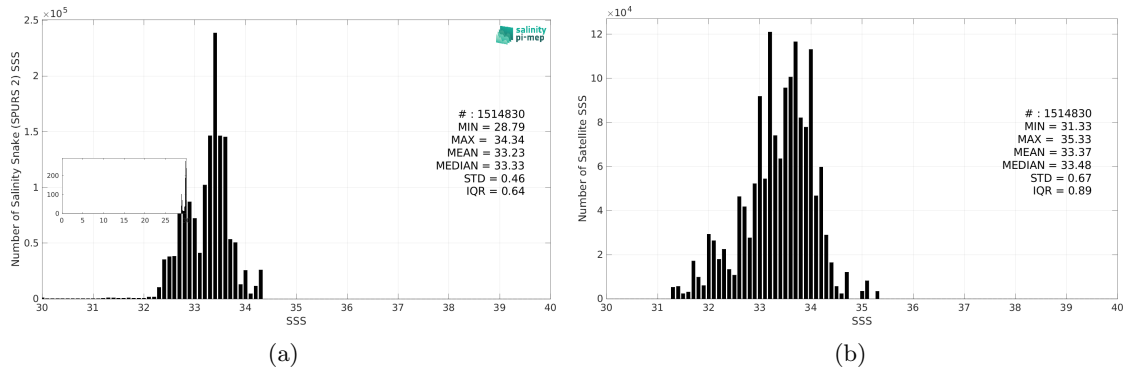
Figure 3: Histograms of SSS from Salinity Snake (SPURS 2) (a) and SMOS SSS L2 v700 (ESA) (b) considering all match-up pairs per bins of 0.1 over the SPURS 2 Pi-MEP region and for the full satellite product period.
