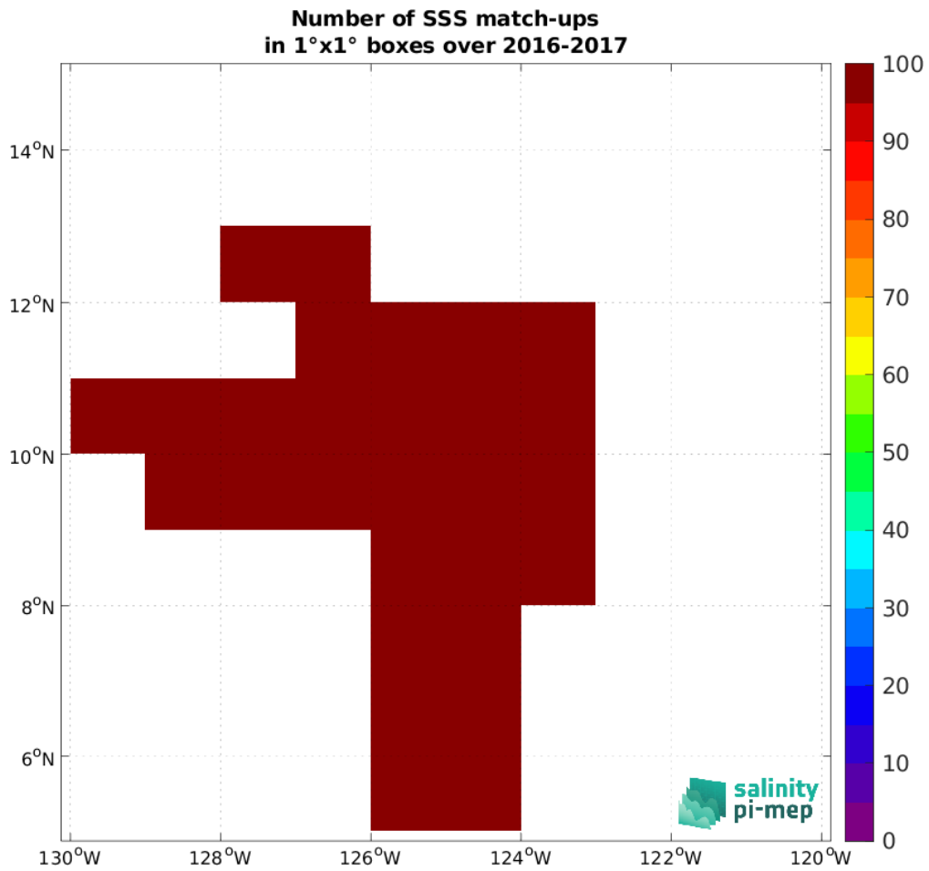
Figure 5: Number of SSS match-ups between Salinity Snake (SPURS 2) SSS and the SMOS SSS L2 v700 (ESA) SSS product for the SPURS 2 Pi-MEP region over 1^\circ \times 1^\circ boxes and for the full satellite product period.
