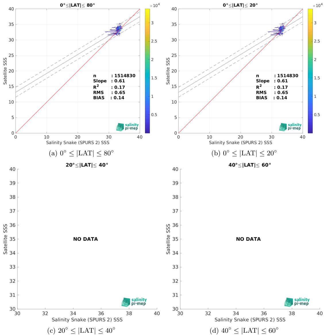
Figure 10: Contour maps of the concentration of SMOS SSS L2 v700 (ESA) SSS (y-axis) versus Salinity Snake (SPURS 2) SSS (x-axis) at match-up pairs for different latitude bands. For each plot, the red line shows x=y . The black thin and dashed lines indicate a linear fit through the data cloud and the \pm 95\% confidence levels, respectively. The number match-up pairs n , the slope and R^2 coefficient of the linear fit, the root mean square (RMS) and the mean bias between satellite and in situ data are indicated for each latitude band in each plots.
