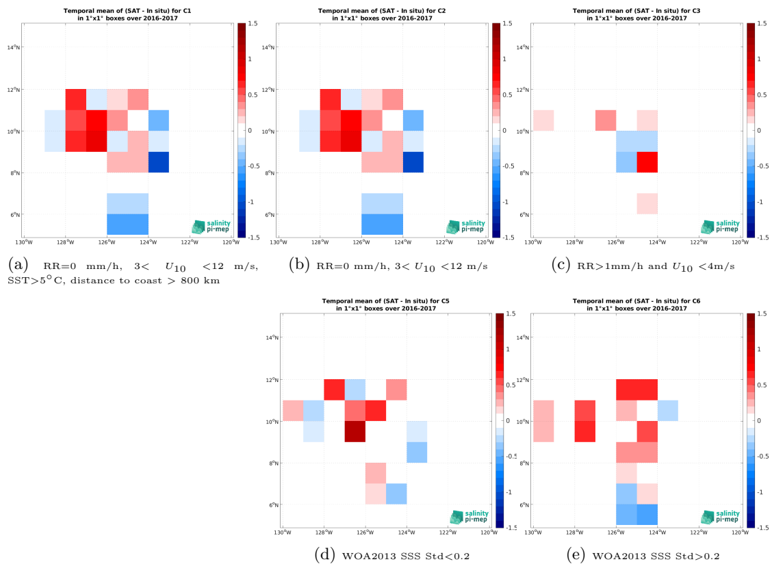
Figure 14: Temporal mean gridded over spatial boxes of size 1^\circ \times 1^\circ of \Delta\text{SSS} (SMOS SSS L2 v700 (ESA) - Salinity Snake (SPURS 2)) for 5 different subdatasets corresponding to: RR=0 mm/h, 3 < U_{10} < 12 m/s, SST > 5°C, distance to coast > 800 km (a), RR=0 mm/h, 3 < U_{10} < 12 m/s (b), RR > 1 mm/h and U_{10} < 4 m/s (c), WOA2013 SSS Std < 0.2 (d), WOA2013 SSS Std > 0.2 (e).
