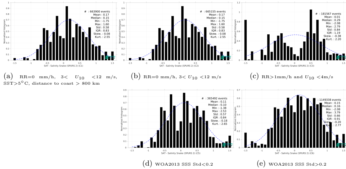
Figure 13: Normalized histogram of \Delta SSS (SMOS SSS L2 v700 (ESA) - Salinity Snake (SPURS 2)) for 5 different subdatasets corresponding to: RR=0 mm/h, 3 < U_{10} < 12 m/s, SST>5°C, distance to coast > 800 km (a), RR=0 mm/h, 3 < U_{10} < 12 m/s (b), RR>1mm/h and U_{10} < 4 m/s (c), WOA2013 SSS Std<0.2 (d), WOA2013 SSS Std>0.2 (e).
