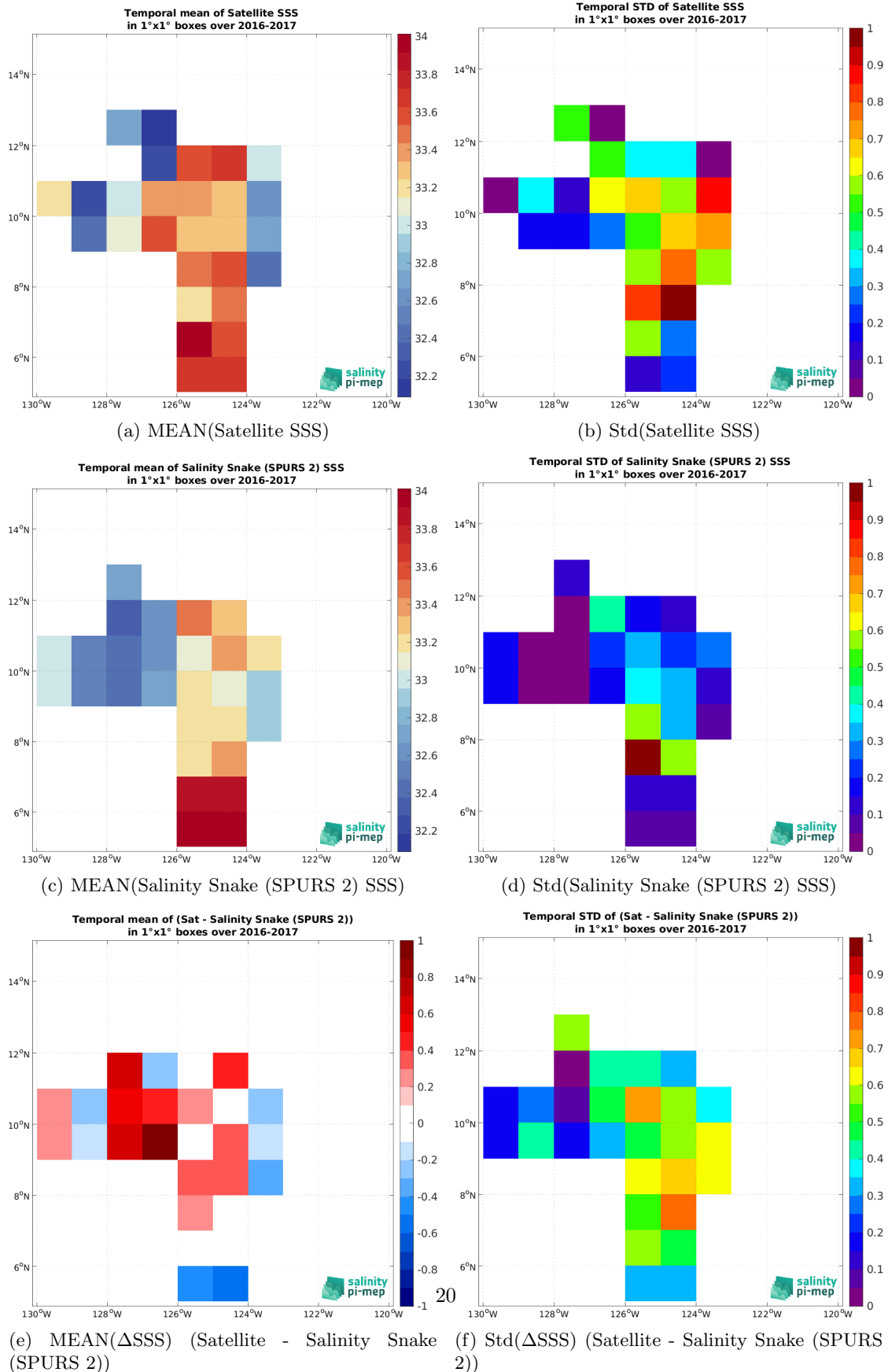
Figure 6: Temporal mean (left) and Std (right) of SSS from SMOS SSS L2 v700 (ESA) (top), Salinity Snake (SPURS 2) (middle), and of \Delta SSS (Satellite - Salinity Snake (SPURS 2)). Only match-up pairs are used to generate these maps.
