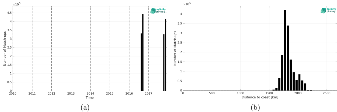
Figure 1: Number of match-ups between Salinity Snake (SPURS 2) and SMOS SSS L2 v700 (ESA) SSS as a function of time (a) and as function of the distance to coast (b) over the SPURS 2 Pi-MEP region and for the full satellite product period.
