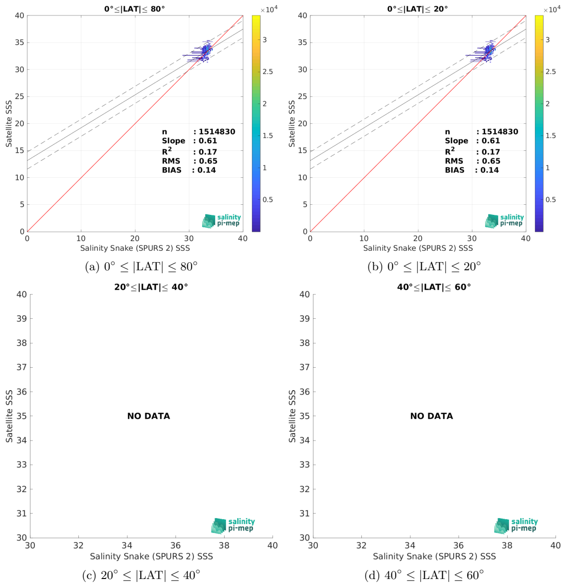
Figure 9: Contour maps of the concentration of SMOS SSS L2 v700 (ESA) SSS (y-axis) versus Salinity Snake (SPURS 2) SSS (x-axis) at match-up pairs for different latitude bands. For each plot, the red line shows x=y . The black thin and dashed lines indicate a linear fit through the data cloud and the \pm 95\% confidence levels, respectively. The number match-up pairs n , the slope and R^2 coefficient of the linear fit, the root mean square (RMS) and the mean bias between satellite and in situ data are indicated for each latitude band in each plots.
