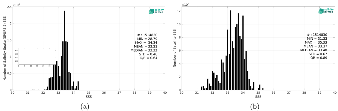
Figure 2: Histograms of SSS from Salinity Snake (SPURS 2) (a) and SMOS SSS L2 v700 (ESA) (b) considering all match-up pairs per bins of 0.1 over the SPURS 2 Pi-MEP region and for the full satellite product period.
