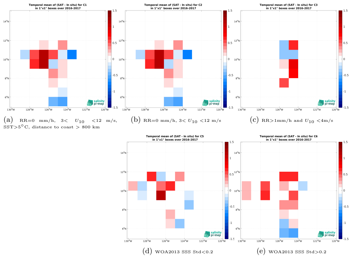
Figure 12: Temporal mean gridded over spatial boxes of size 1^\circ \times 1^\circ of \Delta\text{SSS} (SMOS SSS L2 v700 (ESA) - Salinity Snake (SPURS 2)) for 5 different subdatasets corresponding to:RR=0 mm/h, 3 < U_{10} < 12 m/s, SST>5°C, distance to coast > 800 km (a), RR=0 mm/h, 3 < U_{10} < 12 m/s (b), RR>1mm/h and U_{10} < 4 m/s (c), WOA2013 SSS Std<0.2 (d), WOA2013 SSS Std>0.2 (e).
