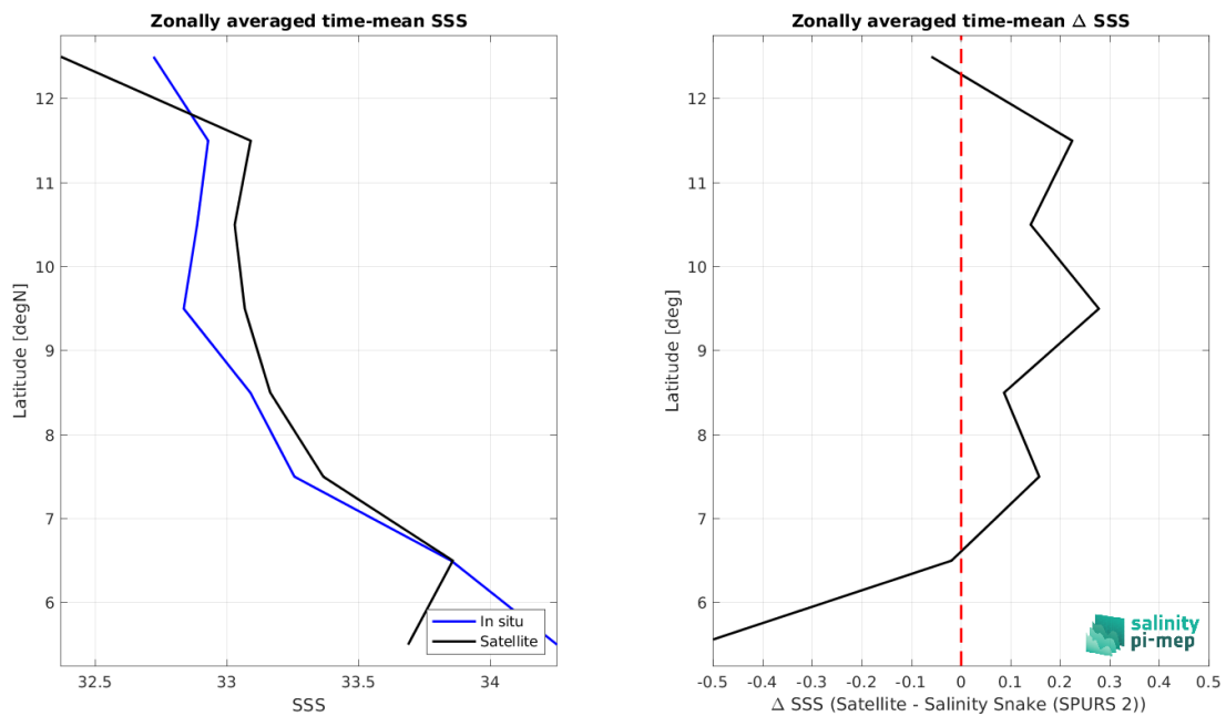
Figure 8: Left panel: Zonal mean SSS from SMOS SSS L2 v700 (ESA) satellite product (black) and from Salinity Snake (SPURS 2) (blue). Right panel: Zonal mean of \Delta SSS (Satellite - Salinity Snake (SPURS 2)) for all the collected Pi-MEP match-up pairs estimated over the full satellite product period.
