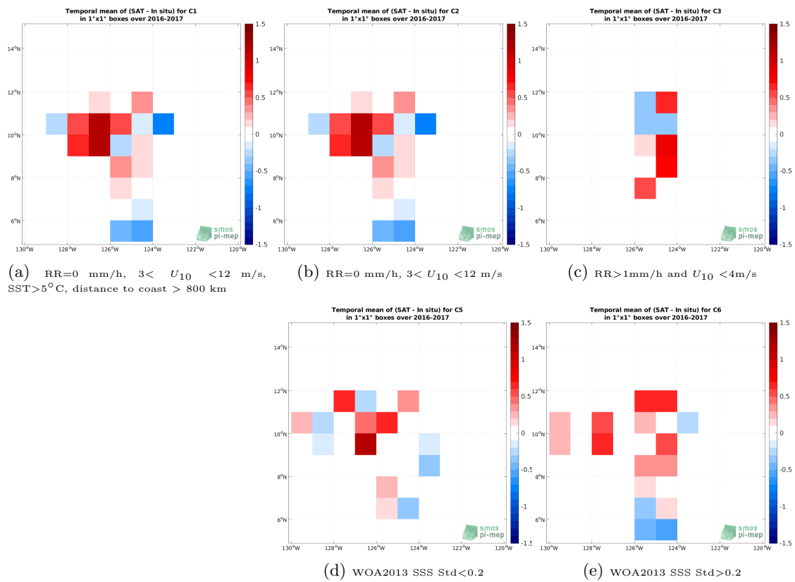
Figure 12: Temporal mean gridded over spatial boxes of size 1^\circ \times 1^\circ of \Delta SSS (SMOS SSS L2 v700 (ESA) - Salinity Snake (SPURS 2)) for 5 different subdatasets corresponding to:RR=0 mm/h, 3 < U_{10} < 12 m/s, SST >5^\circ C, distance to coast > 800 km (a), RR=0 mm/h, 3 < U_{10} < 12 m/s (b), RR >1 mm/h and U_{10} < 4 m/s (c), WOA2013 SSS Std <0.2 (d), WOA2013 SSS Std >0.2 (e).
