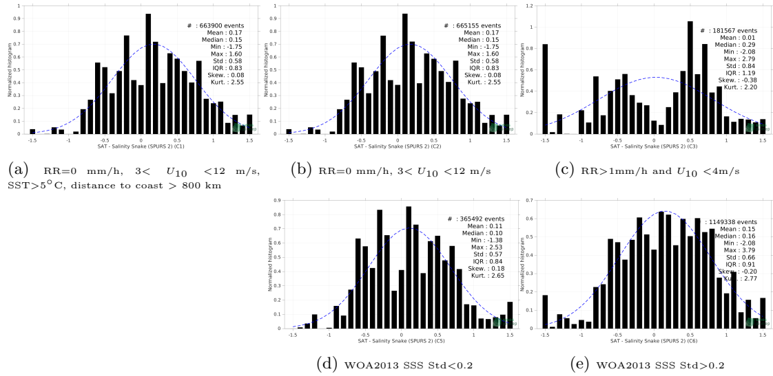
Figure 13: Normalized histogram of \Delta SSS (SMOS SSS L2 v700 (ESA) - Salinity Snake (SPURS 2)) for 5 different subdatasets corresponding to: RR=0 mm/h, 3 < U_{10} < 12 m/s, SST > 5°C, distance to coast > 800 km (a), RR=0 mm/h, 3 < U_{10} < 12 m/s (b), RR > 1mm/h and U_{10} < 4 m/s (c), WOA2013 SSS Std < 0.2 (d), WOA2013 SSS Std > 0.2 (e).
