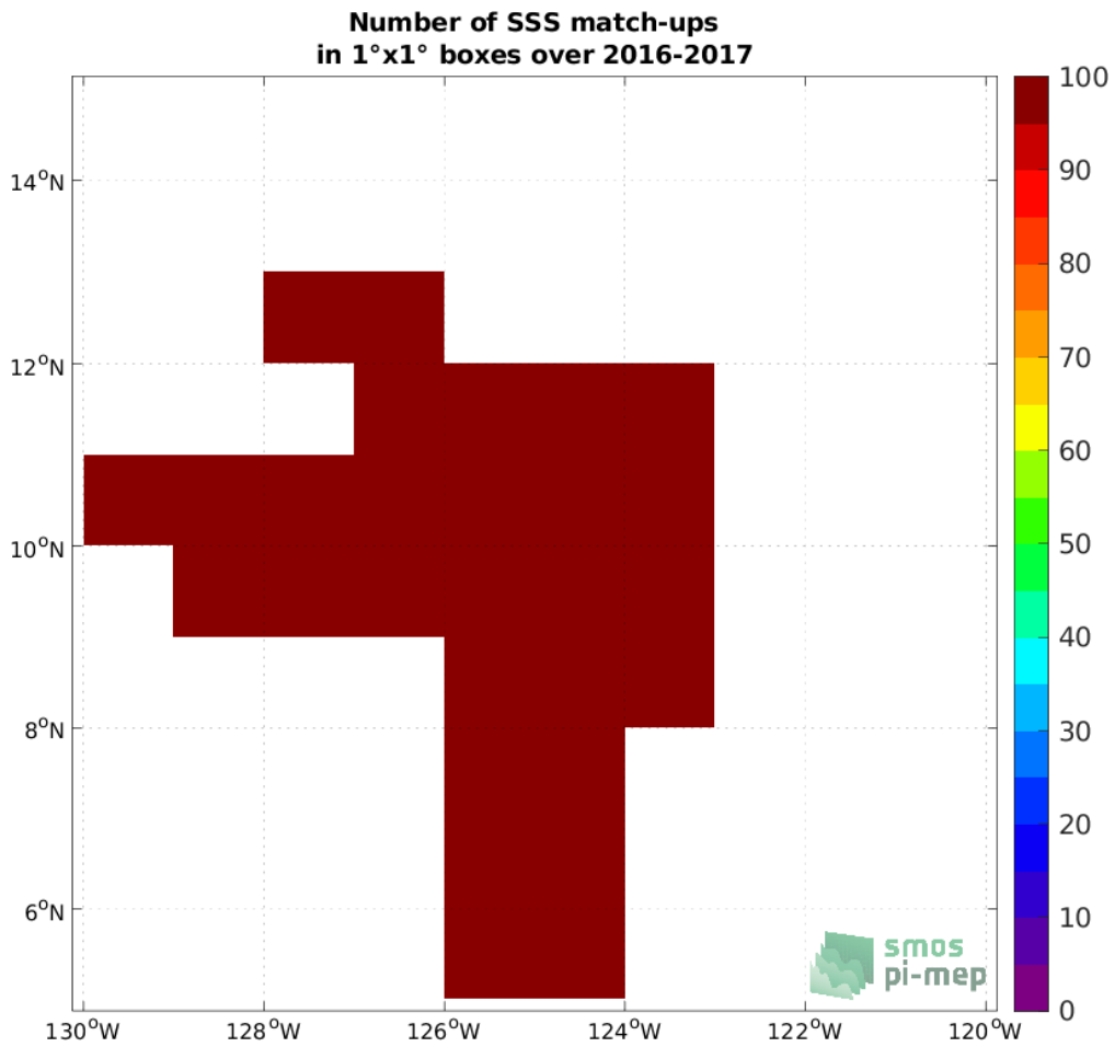
Figure 4: Number of SSS match-ups between Salinity Snake (SPURS 2) SSS and the SMOS SSS L2 v700 (ESA) SSS product for the SPURS 2 Pi-MEP region over 1°x1° boxes and for the full satellite product period.
