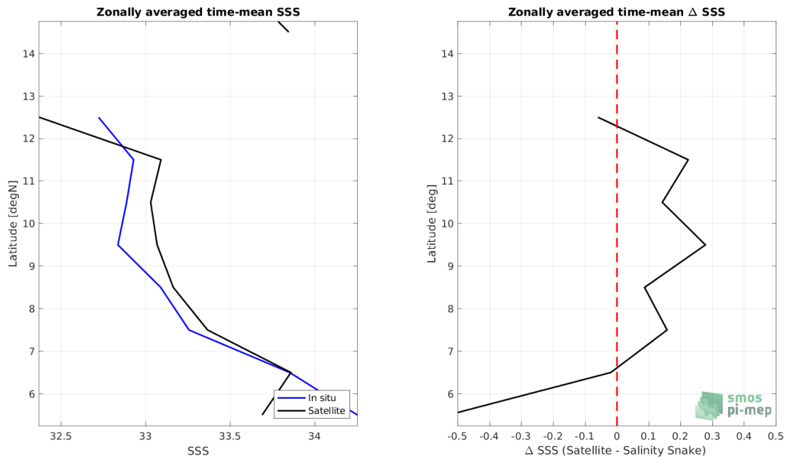
Figure 8: Left panel: Zonal mean SSS from SMOS SSS L2 v700 (ESA) satellite product (black) and from Salinity Snake (blue). Right panel: Zonal mean of \Delta SSS (Satellite - Salinity Snake) for all the collected Pi-MEP match-up pairs estimated over the full satellite product period.
