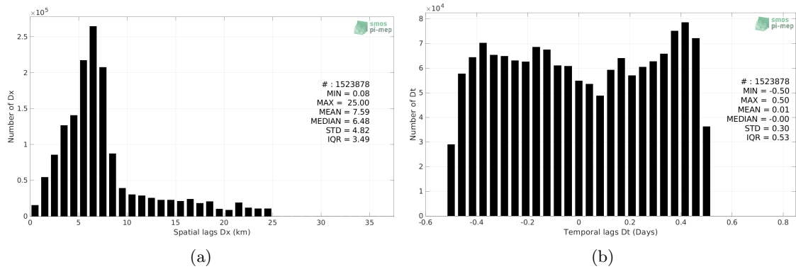
Figure 5: Histograms of the spatial (a) and temporal (b) lags between the location/time of the Salinity Snake measurement and the date of the corresponding SMOS SSS L2 v700 (ESA) SSS pixel.
