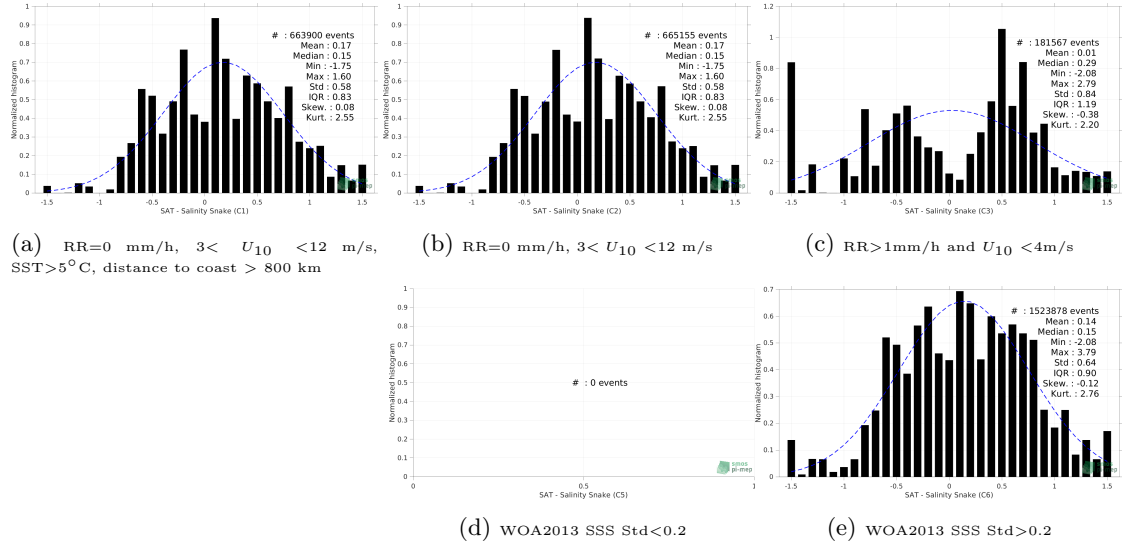
Figure 13: Normalized histogram of \Delta SSS (SMOS SSS L2 v700 (ESA) - Salinity Snake) for 5 different subdatasets corresponding to: RR=0 mm/h, 3 < U_{10} < 12 m/s, SST > 5°C, distance to coast > 800 km (a), RR=0 mm/h, 3 < U_{10} < 12 m/s (b), RR > 1mm/h and U_{10} < 4 m/s (c), WOA2013 SSS Std < 0.2 (d), WOA2013 SSS Std > 0.2 (e).
