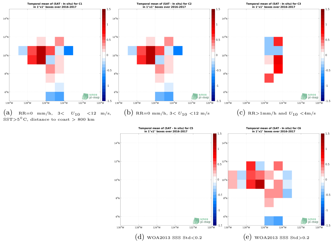
Figure 12: Temporal mean gridded over spatial boxes of size 1^\circ \times 1^\circ of \Delta SSS (SMOS SSS L2 v700 (ESA) - Salinity Snake) for 5 different subdatasets corresponding to:RR=0 mm/h, 3 < U_{10} < 12 m/s, SST >5^\circ C, distance to coast > 800 km (a), RR=0 mm/h, 3 < U_{10} < 12 m/s (b), RR >1 mm/h and U_{10} < 4 m/s (c), WOA2013 SSS Std <0.2 (d), WOA2013 SSS Std >0.2 (e).
