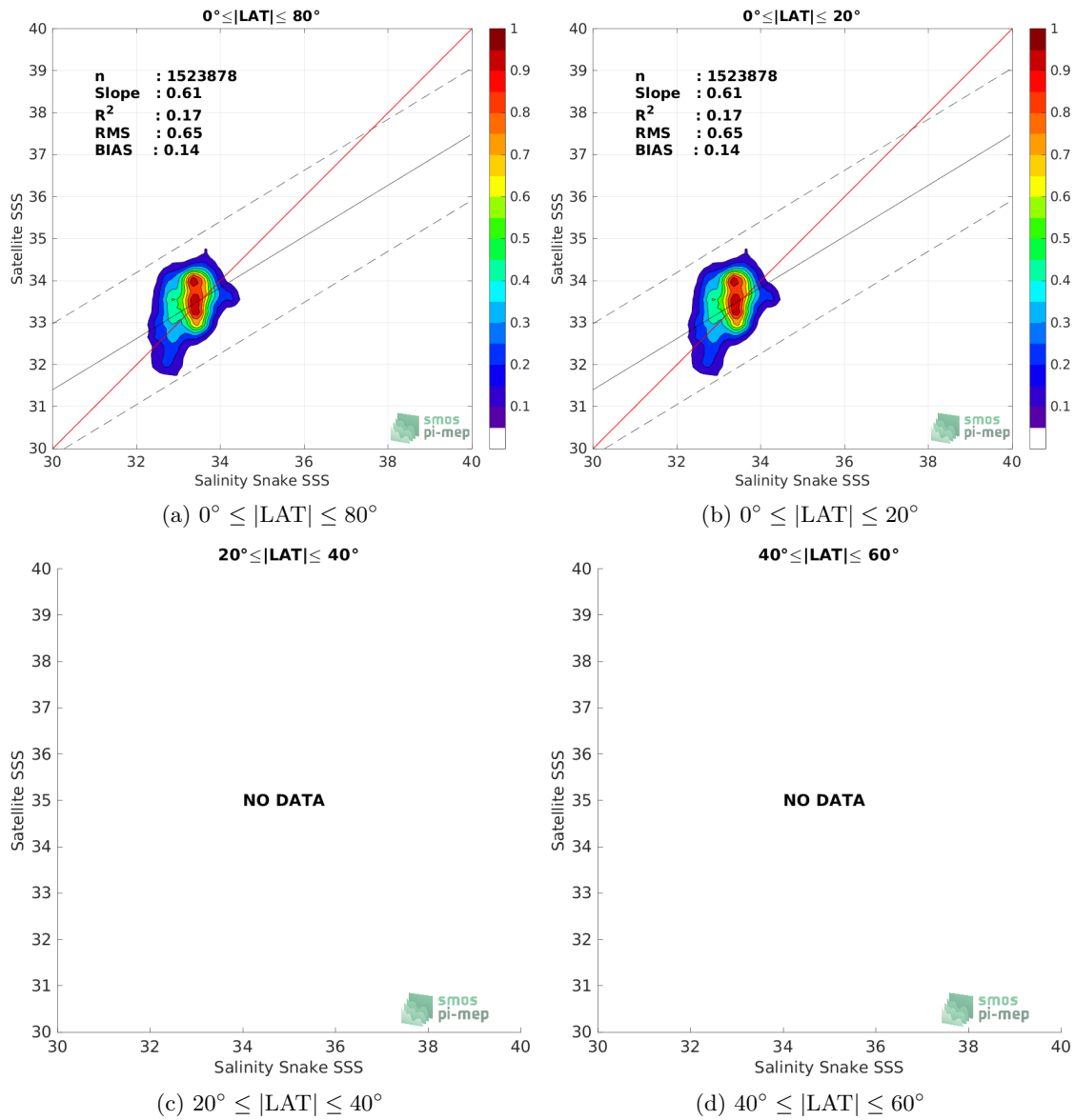
Figure 9: Contour maps of the concentration of SMOS SSS L2 v700 (ESA) SSS (y-axis) versus Salinity Snake SSS (x-axis) at match-up pairs for different latitude bands. For each plot, the red line shows x=y . The black thin and dashed lines indicate a linear fit through the data cloud and the \pm 95\% confidence levels, respectively. The number match-up pairs n , the slope and R^2 coefficient of the linear fit, the root mean square (RMS) and the mean bias between satellite and in situ data are indicated for each latitude band in each plots.
