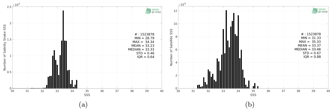
Figure 2: Histograms of SSS from Salinity Snake (a) and SMOS SSS L2 v700 (ESA) (b) considering all match-up pairs per bins of 0.1 over the SPURS 2 Pi-MEP region and for the full satellite product period.
