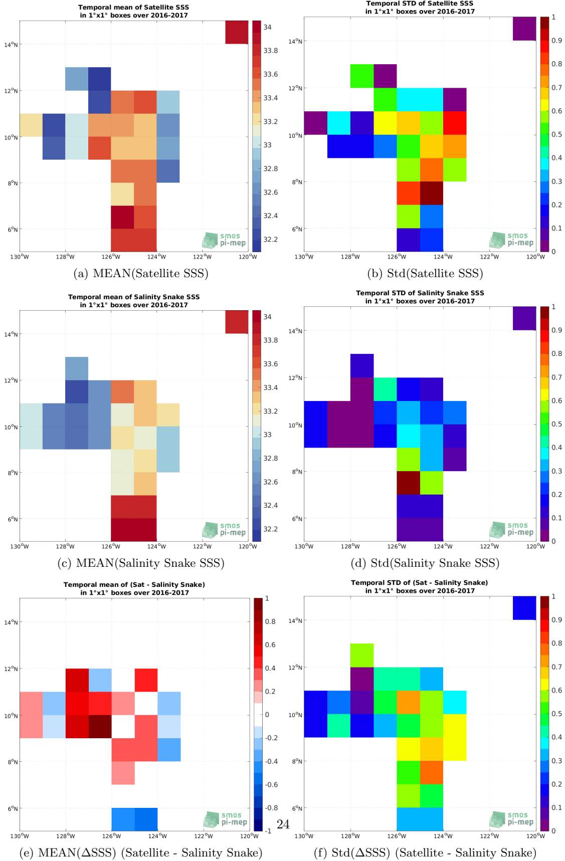
Figure 5: Temporal mean (left) and Std (right) of SSS from SMOS SSS L2 v700 (ESA) (top), Salinity Snake (middle), and of \Delta SSS (Satellite - Salinity Snake). Only match-up pairs are used to generate these maps.
