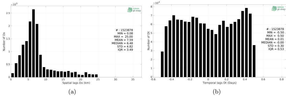
Figure 4: Histograms of the spatial (a) and temporal (b) lags between the location/time of the Salinity Snake measurement and the date of the corresponding SMOS SSS L2 v700 (ESA) SSS pixel.
