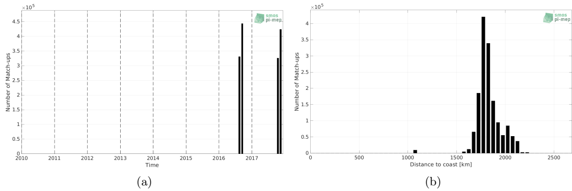
Figure 1: Number of match-ups between Salinity Snake and SMOS SSS L2 v700 (ESA) SSS as a function of time (a) and as function of the distance to coast (b) over the SPURS 2 Pi-MEP region and for the full satellite product period.
