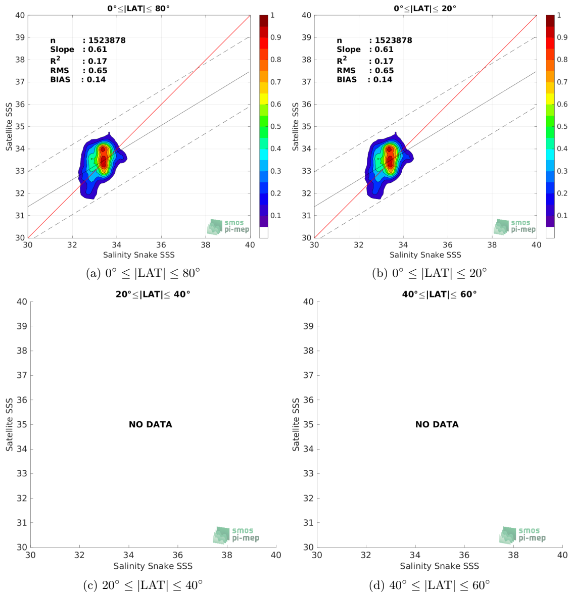
Figure 8: Contour maps of the concentration of SMOS SSS L2 v700 (ESA) SSS (y-axis) versus Salinity Snake SSS (x-axis) at match-up pairs for different latitude bands. For each plot, the red line shows x=y . The black thin and dashed lines indicate a linear fit through the data cloud and the \pm 95\% confidence levels, respectively. The number match-up pairs n , the slope and R^2 coefficient of the linear fit, the root mean square (RMS) and the mean bias between satellite and in situ data are indicated for each latitude band in each plots.
