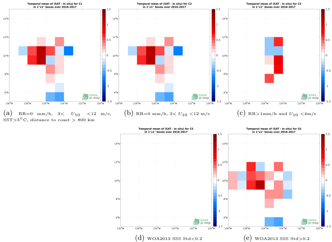
Figure 11: Temporal mean gridded over spatial boxes of size 1^\circ \times 1^\circ of \Delta SSS (SMOS SSS L2 v700 (ESA) - Salinity Snake) for 5 different subdatasets corresponding to:RR=0 mm/h, 3 < U_{10} < 12 m/s, SST >5^\circ C, distance to coast > 800 km (a), RR=0 mm/h, 3 < U_{10} < 12 m/s (b), RR >1 mm/h and U_{10} < 4 m/s (c), WOA2013 SSS Std <0.2 (d), WOA2013 SSS Std >0.2 (e).
