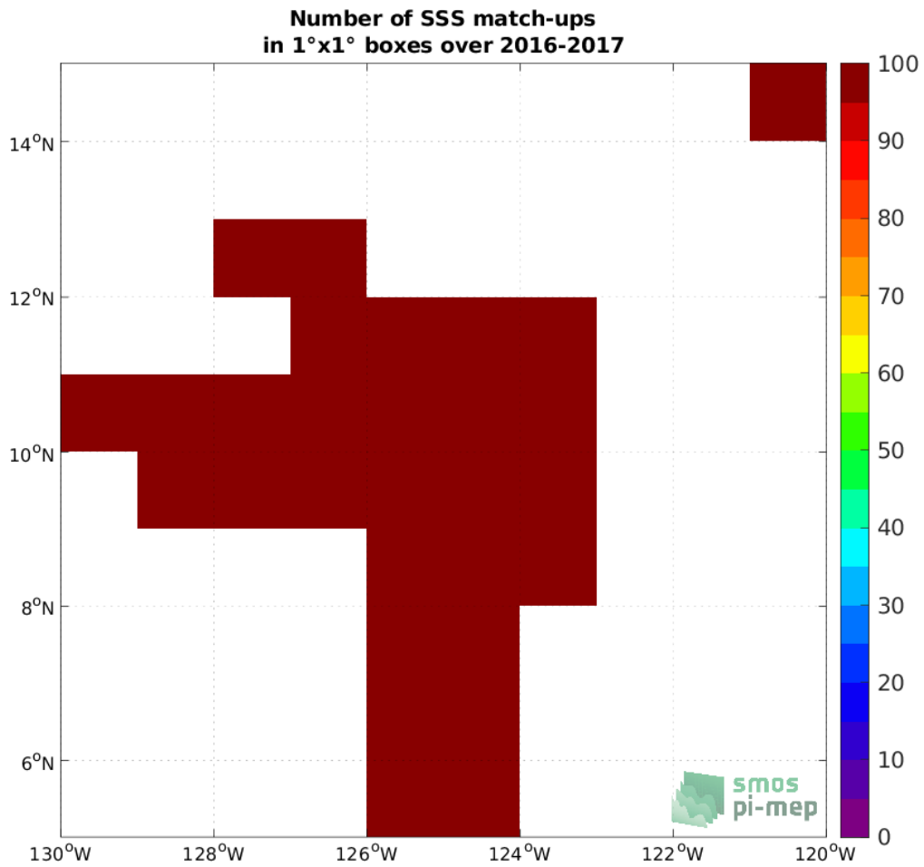
Figure 3: Number of SSS match-ups between Salinity Snake SSS and the SMOS SSS L2 v700 (ESA) SSS product for the SPURS 2 Pi-MEP region over 1°x1° boxes and for the full satellite product period.
