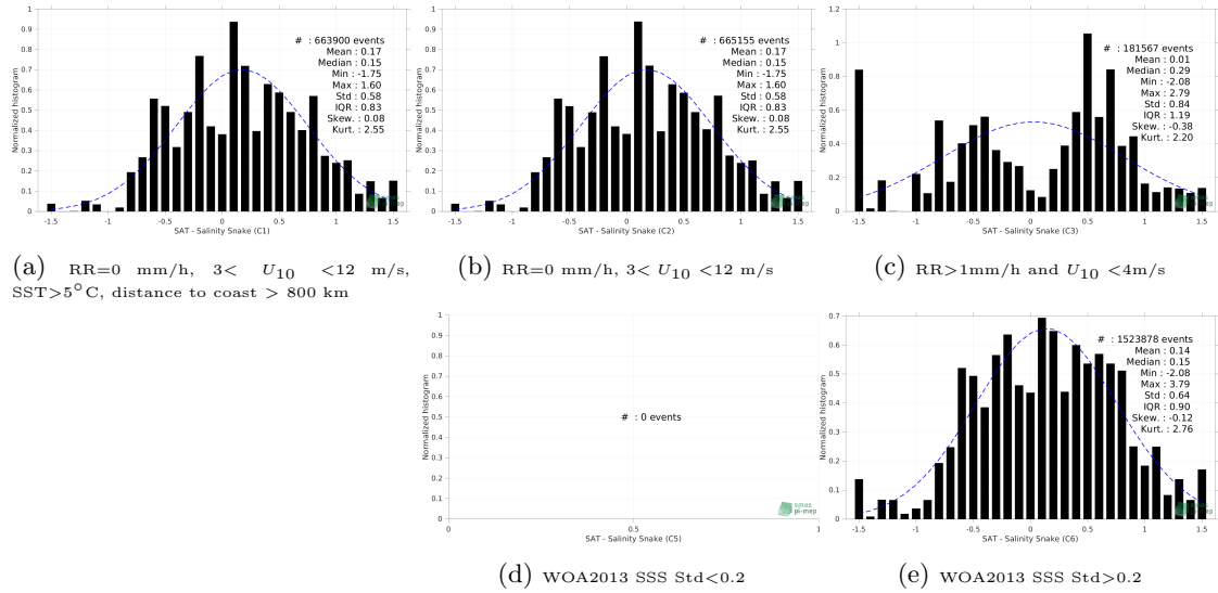
Figure 12: Normalized histogram of \Delta SSS (SMOS SSS L2 v700 (ESA) - Salinity Snake) for 5 different subdatasets corresponding to: RR=0 mm/h, 3 < U_{10} < 12 m/s, SST > 5°C, distance to coast > 800 km (a), RR=0 mm/h, 3 < U_{10} < 12 m/s (b), RR > 1mm/h and U_{10} < 4 m/s (c), WOA2013 SSS Std < 0.2 (d), WOA2013 SSS Std > 0.2 (e).
