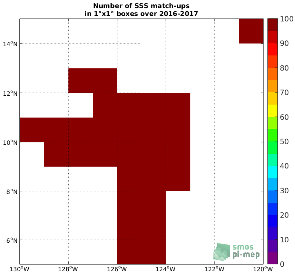
Figure 3: Number of SSS match-ups between Salinity Snake SSS and the SMOS SSS L2 v700 (ESA) SSS product for the SPURS 2 Pi-MEP region over 1°x1° boxes and for the full satellite product period.
