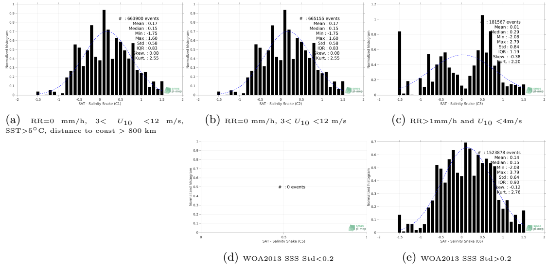
Figure 12: Normalized histogram of \Delta SSS (SMOS SSS L2 v700 (ESA) - Salinity Snake) for 5 different subdatasets corresponding to: RR=0 mm/h, 3 < U_{10} < 12 m/s, SST>5°C, distance to coast > 800 km (a), RR=0 mm/h, 3 < U_{10} < 12 m/s (b), RR>1mm/h and U_{10} < 4 m/s (c), WOA2013 SSS Std<0.2 (d), WOA2013 SSS Std>0.2 (e).
