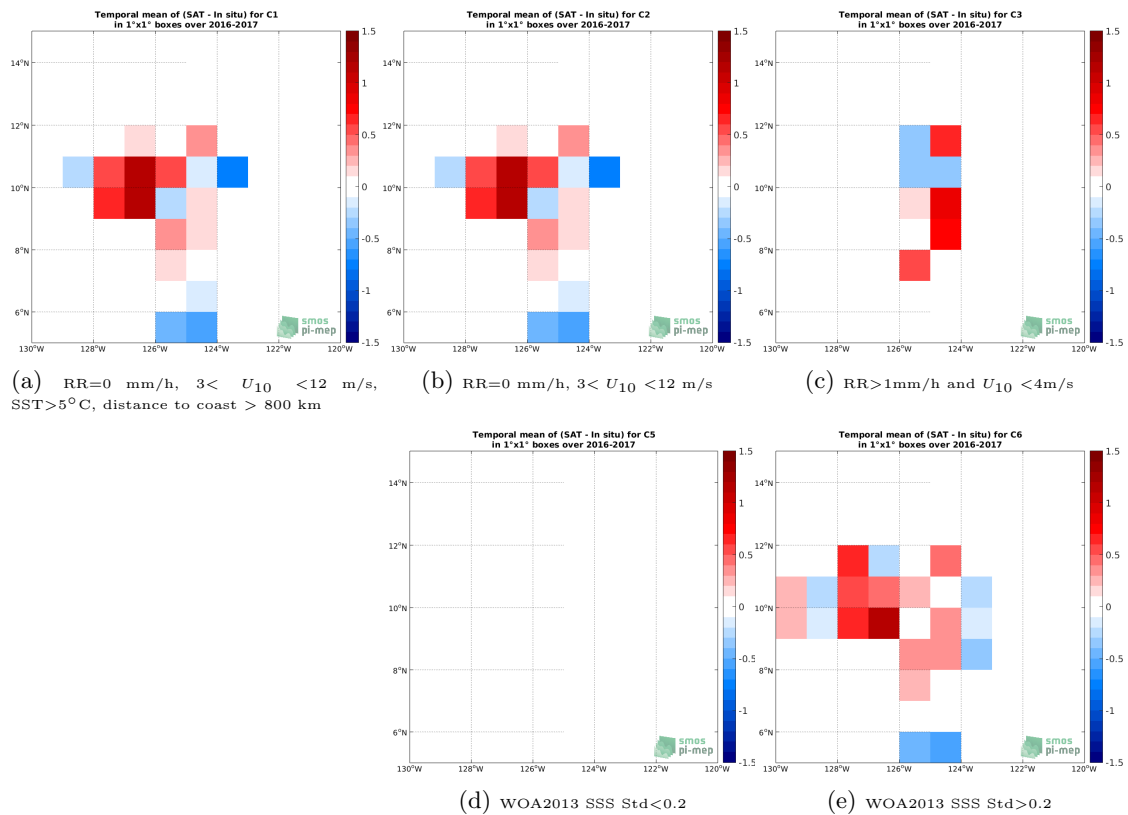
Figure 11: Temporal mean gridded over spatial boxes of size 1^\circ \times 1^\circ of \Delta SSS (SMOS SSS L2 v700 (ESA) - Salinity Snake) for 5 different subdatasets corresponding to:RR=0 mm/h, 3 < U_{10} < 12 m/s, SST>5°C, distance to coast > 800 km (a), RR=0 mm/h, 3 < U_{10} < 12 m/s (b), RR>1mm/h and U_{10} < 4 m/s (c), WOA2013 SSS Std<0.2 (d), WOA2013 SSS Std>0.2 (e).
