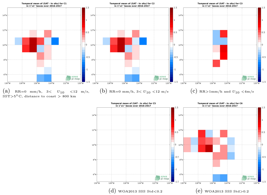
Figure 11: Temporal mean gridded over spatial boxes of size 1°x1° of \Delta SSS (SMOS SSS L2 v700 (ESA) - Salinity Snake) for 5 different subdatasets corresponding to:RR=0 mm/h, 3 < U_{10} < 12 m/s, SST>5°C, distance to coast > 800 km (a), RR=0 mm/h, 3 < U_{10} < 12 m/s (b), RR>1mm/h and U_{10} < 4m/s (c), WOA2013 SSS Std<0.2 (d), WOA2013 SSS Std>0.2 (e).
