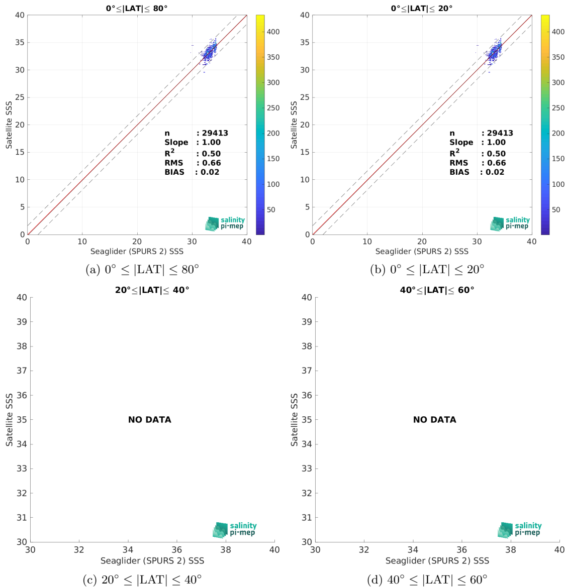
Figure 10: Contour maps of the concentration of SMOS SSS L2 v700 (ESA) SSS (y-axis) versus Seaglider (SPURS 2) SSS (x-axis) at match-up pairs for different latitude bands. For each plot, the red line shows x=y . The black thin and dashed lines indicate a linear fit through the data cloud and the \pm 95\% confidence levels, respectively. The number match-up pairs n , the slope and R^2 coefficient of the linear fit, the root mean square (RMS) and the mean bias between satellite and in situ data are indicated for each latitude band in each plots.
