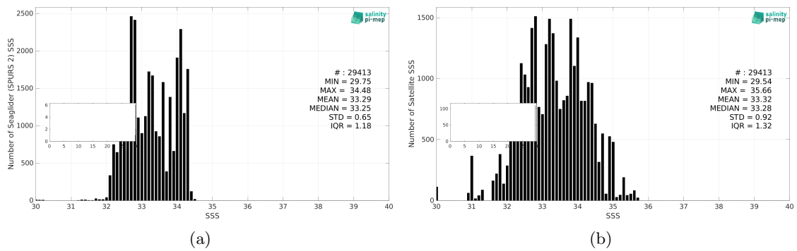
Figure 3: Histograms of SSS from Seaglider (SPURS 2) (a) and SMOS SSS L2 v700 (ESA) (b) considering all match-up pairs per bins of 0.1 over the SPURS 2 Pi-MEP region and for the full satellite product period.
