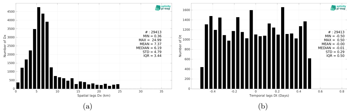
Figure 6: Histograms of the spatial (a) and temporal (b) lags between the location/time of the Seaglider (SPURS 2) measurement and the date of the corresponding SMOS SSS L2 v700 (ESA) SSS pixel.
