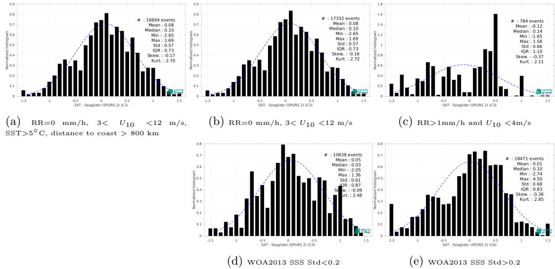
Figure 15: Normalized histogram of \Delta SSS (SMOS SSS L2 v700 (ESA) - Seaglider (SPURS 2)) for 5 different subdatasets corresponding to: RR=0 mm/h, 3 < U_{10} < 12 m/s, SST > 5°C, distance to coast > 800 km (a), RR=0 mm/h, 3 < U_{10} < 12 m/s (b), RR > 1mm/h and U_{10} < 4 m/s (c), WOA2013 SSS Std < 0.2 (d), WOA2013 SSS Std > 0.2 (e).
