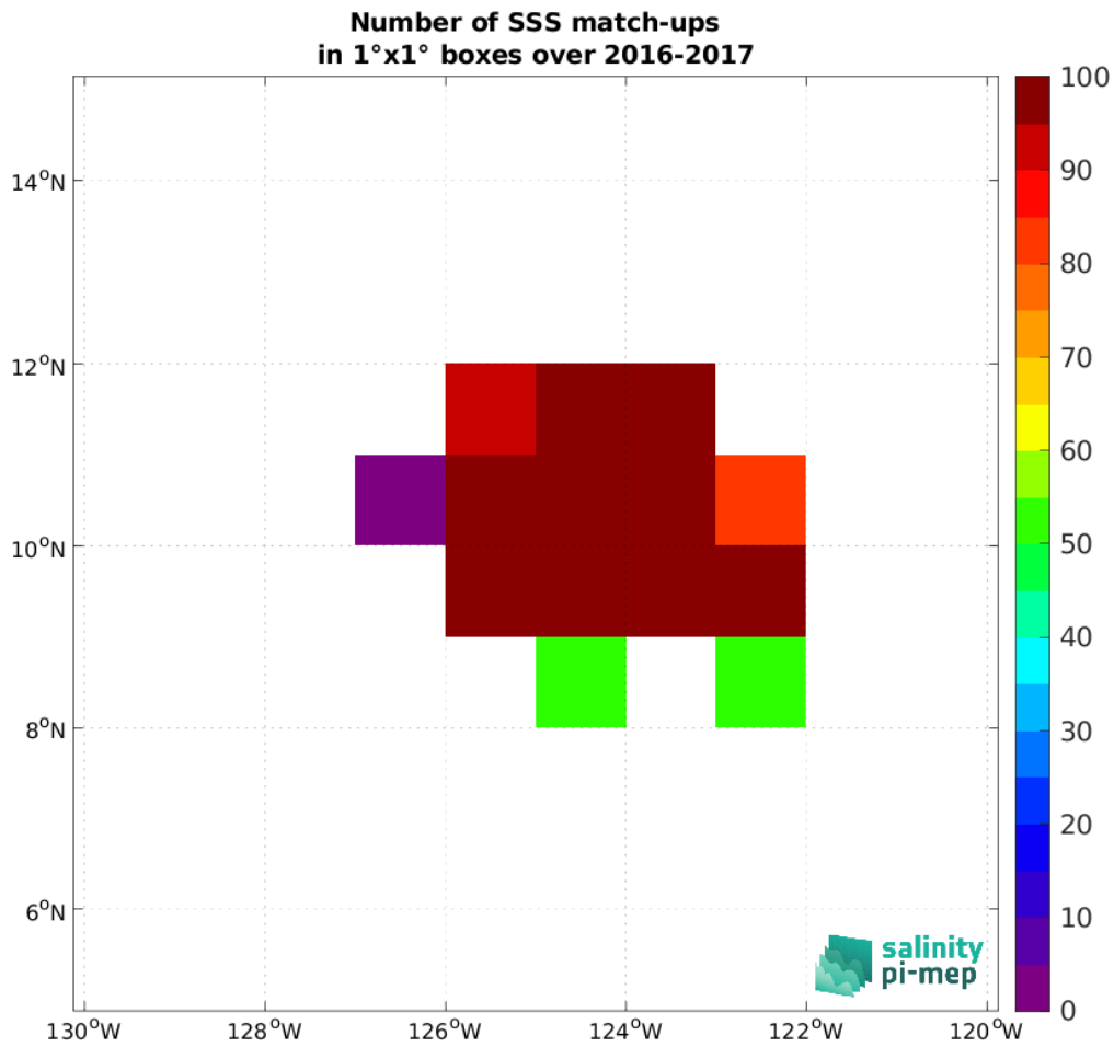
Figure 5: Number of SSS match-ups between Seagliders (SPURS 2) SSS and the SMOS SSS L2 v700 (ESA) SSS product for the SPURS 2 Pi-MEP region over 1°x1° boxes and for the full satellite product period.
