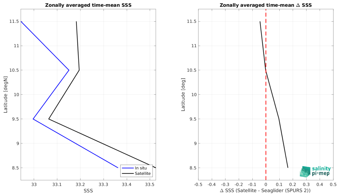
Figure 9: Left panel: Zonal mean SSS from SMOS SSS L2 v700 (ESA) satellite product (black) and from Seaglider (SPURS 2) (blue). Right panel: Zonal mean of \Delta SSS (Satellite - Seaglider (SPURS 2)) for all the collected Pi-MEP match-up pairs estimated over the full satellite product period.
