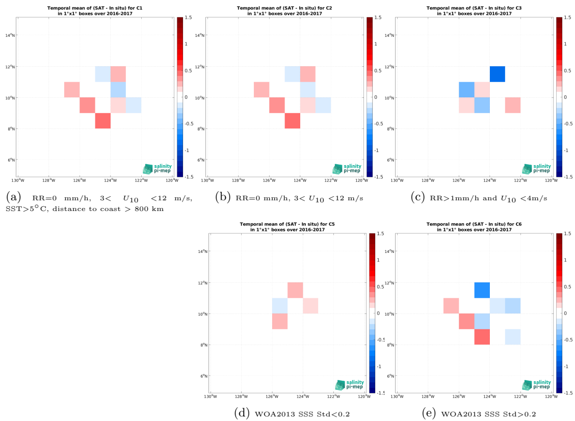
Figure 14: Temporal mean gridded over spatial boxes of size 1^\circ \times 1^\circ of \Delta SSS (SMOS SSS L2 v700 (ESA) - Seaglider (SPURS 2)) for 5 different subdatasets corresponding to: RR=0 mm/h, 3 < U_{10} < 12 m/s, SST > 5°C, distance to coast > 800 km (a), RR=0 mm/h, 3 < U_{10} < 12 m/s (b), RR > 1mm/h and U_{10} < 4 m/s (c), WOA2013 SSS Std < 0.2 (d), WOA2013 SSS Std > 0.2 (e).
