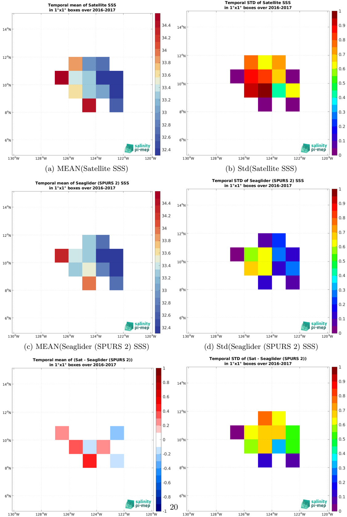
Figure 6: Temporal mean (left) and Std (right) of SSS from SMOS SSS L2 v700 (ESA) (top), Seaglider (SPURS 2) (middle), and of \Delta SSS (Satellite - Seaglider (SPURS 2)). Only match-up pairs are used to generate these maps.
