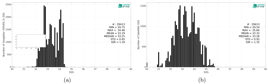
Figure 2: Histograms of SSS from Seaglider (SPURS 2) (a) and SMOS SSS L2 v700 (ESA) (b) considering all match-up pairs per bins of 0.1 over the SPURS 2 Pi-MEP region and for the full satellite product period.
