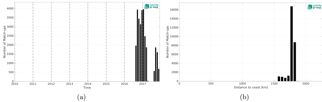
Figure 1: Number of match-ups between Seaglider (SPURS 2) and SMOS SSS L2 v700 (ESA) SSS as a function of time (a) and as function of the distance to coast (b) over the SPURS 2 Pi-MEP region and for the full satellite product period.
