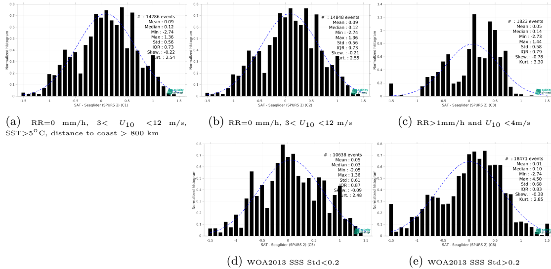
Figure 13: Normalized histogram of \Delta SSS (SMOS SSS L2 v700 (ESA) - Seaglider (SPURS 2)) for 5 different subdatasets corresponding to: RR=0 mm/h, 3 < U_{10} < 12 m/s, SST > 5°C, distance to coast > 800 km (a), RR=0 mm/h, 3 < U_{10} < 12 m/s (b), RR > 1mm/h and U_{10} < 4 m/s (c), WOA2013 SSS Std < 0.2 (d), WOA2013 SSS Std > 0.2 (e).
