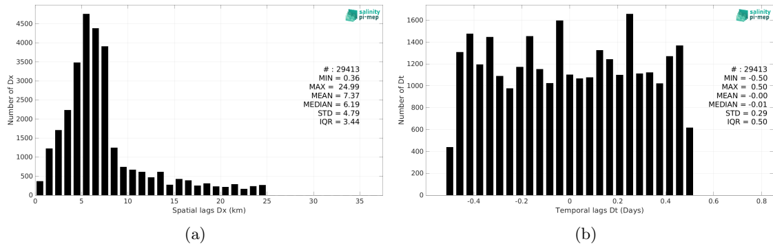
Figure 5: Histograms of the spatial (a) and temporal (b) lags between the location/time of the Seaglider (SPURS 2) measurement and the date of the corresponding SMOS SSS L2 v700 (ESA) SSS pixel.
