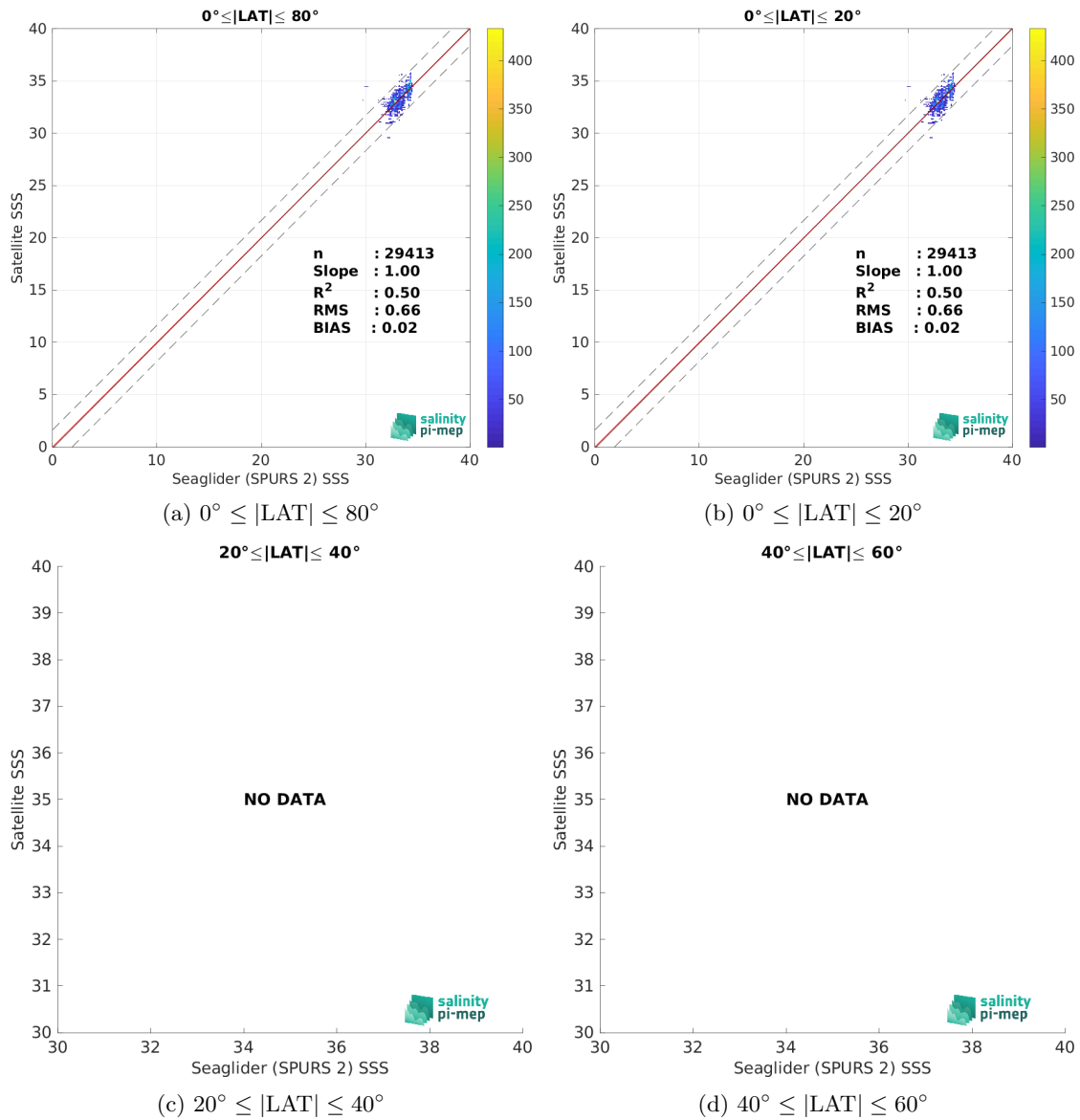
Figure 9: Contour maps of the concentration of SMOS SSS L2 v700 (ESA) SSS (y-axis) versus Seaglider (SPURS 2) SSS (x-axis) at match-up pairs for different latitude bands. For each plot, the red line shows x=y . The black thin and dashed lines indicate a linear fit through the data cloud and the \pm 95\% confidence levels, respectively. The number match-up pairs n , the slope and R^2 coefficient of the linear fit, the root mean square (RMS) and the mean bias between satellite and in situ data are indicated for each latitude band in each plots.
