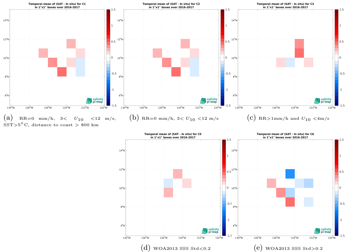
Figure 12: Temporal mean gridded over spatial boxes of size 1^\circ \times 1^\circ of \Delta SSS (SMOS SSS L2 v700 (ESA) - Seaglider (SPURS 2)) for 5 different subdatasets corresponding to:RR=0 mm/h, 3 < U_{10} < 12 m/s, SST >5^\circ\text{C} , distance to coast > 800 km (a), RR=0 mm/h, 3 < U_{10} < 12 m/s (b), RR >1 mm/h and U_{10} < 4 m/s (c), WOA2013 SSS Std <0.2 (d), WOA2013 SSS Std >0.2 (e).
