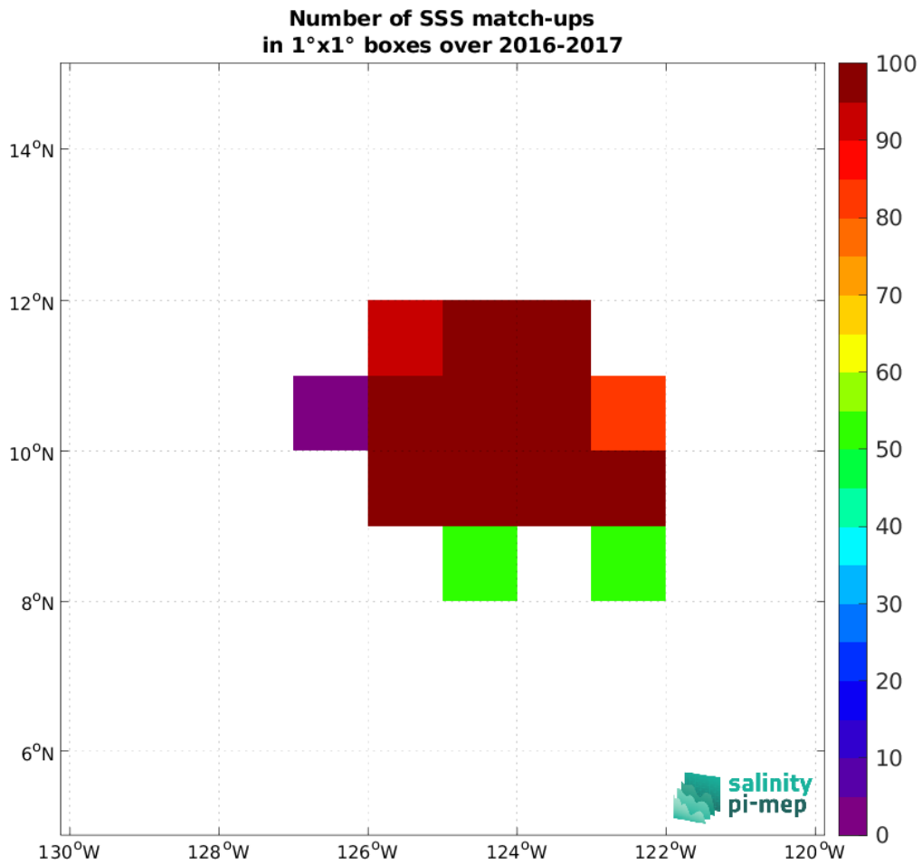
Figure 4: Number of SSS match-ups between Seagliders (SPURS 2) SSS and the SMOS SSS L2 v700 (ESA) SSS product for the SPURS 2 Pi-MEP region over 1°x1° boxes and for the full satellite product period.
