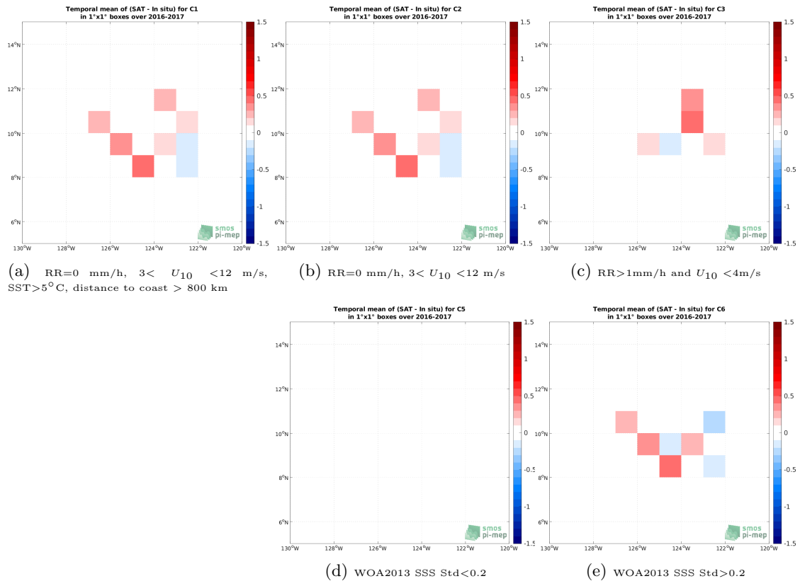
Figure 12: Temporal mean gridded over spatial boxes of size 1^\circ \times 1^\circ of \Delta SSS (SMOS SSS L2 v700 (ESA) - Seaglider) for 5 different subdatasets corresponding to:RR=0 mm/h, 3 < U_{10} < 12 m/s, SST >5^\circ C, distance to coast > 800 km (a), RR=0 mm/h, 3 < U_{10} < 12 m/s (b), RR >1 mm/h and U_{10} < 4 m/s (c), WOA2013 SSS Std <0.2 (d), WOA2013 SSS Std >0.2 (e).
