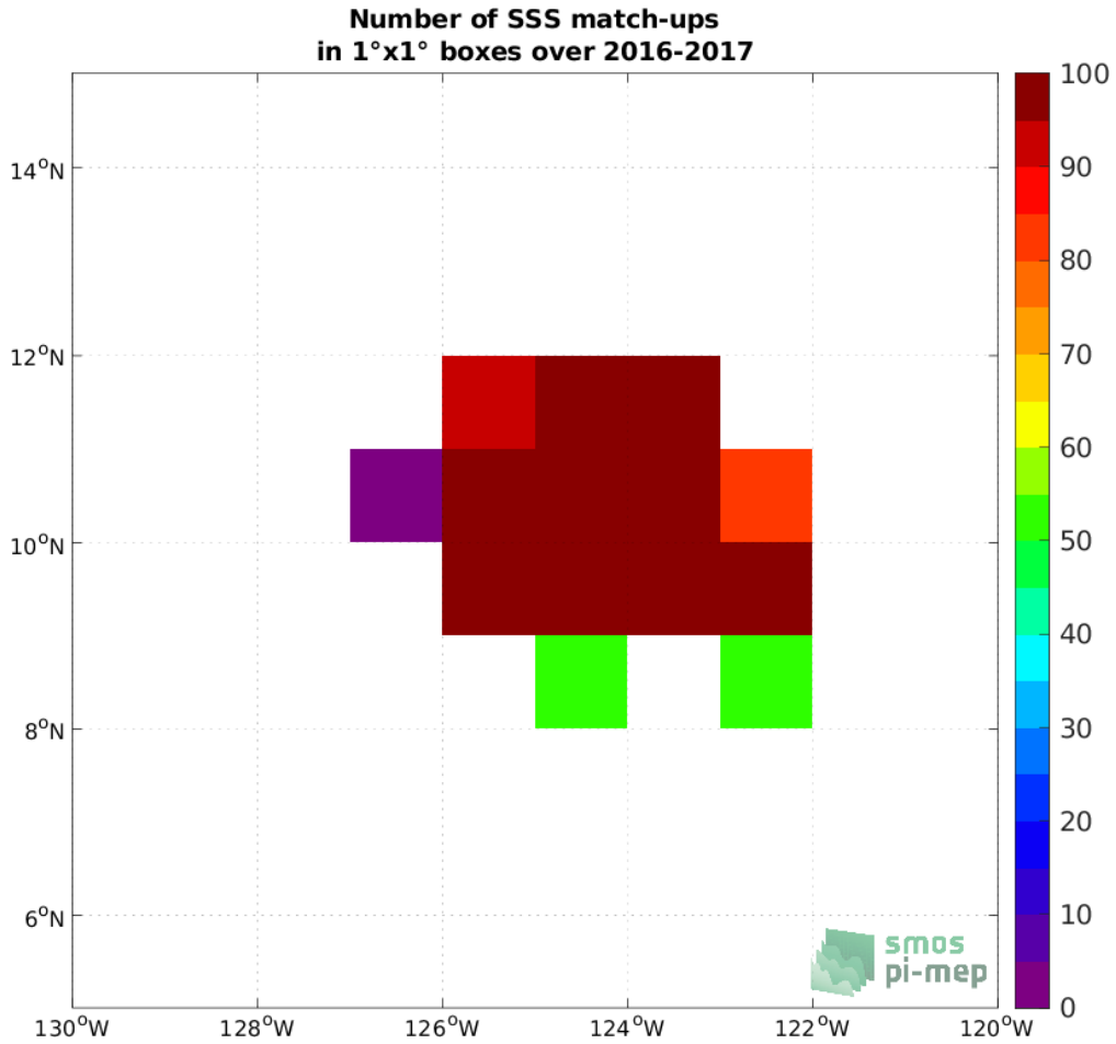
Figure 4: Number of SSS match-ups between Seaglider SSS and the SMOS SSS L2 v700 (ESA) SSS product for the SPURS 2 Pi-MEP region over 1°x1° boxes and for the full satellite product period.
