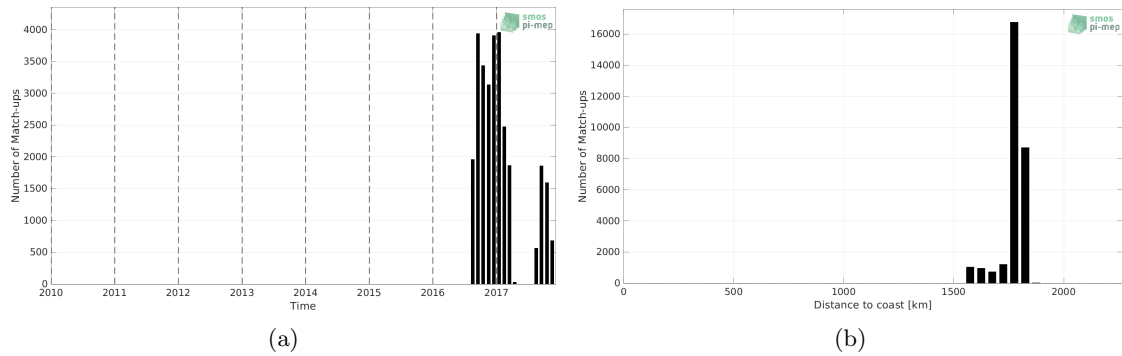
Figure 1: Number of match-ups between Seagliders and SMOS SSS L2 v700 (ESA) SSS as a function of time (a) and as function of the distance to coast (b) over the SPURS 2 Pi-MEP region and for the full satellite product period.
