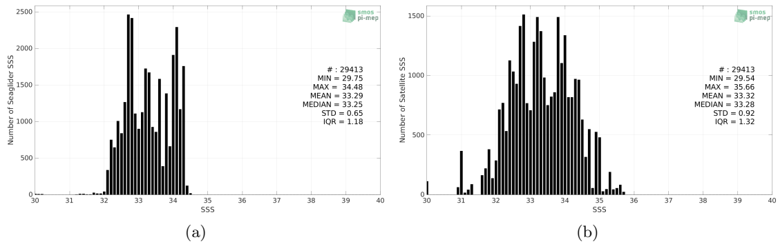
Figure 2: Histograms of SSS from Seagliders (a) and SMOS SSS L2 v700 (ESA) (b) considering all match-up pairs per bins of 0.1 over the SPURS 2 Pi-MEP region and for the full satellite product period.
