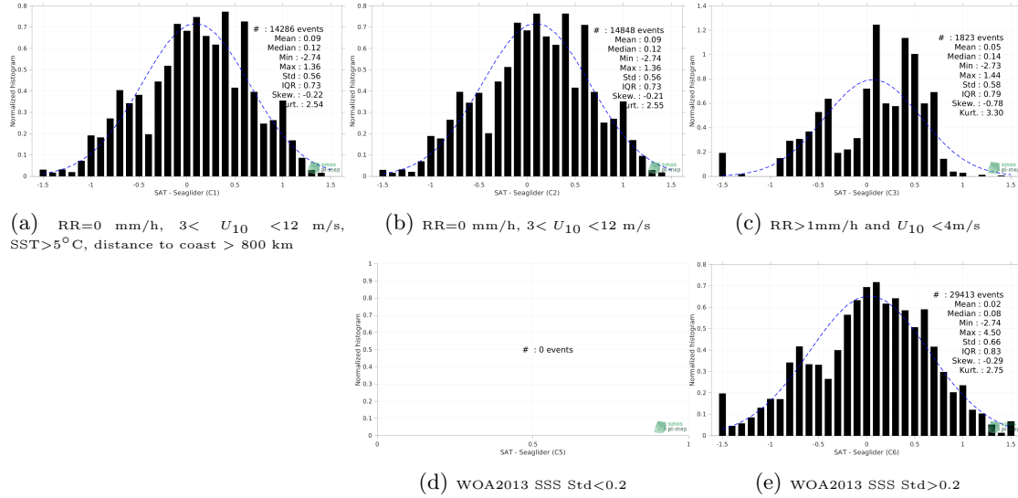
Figure 13: Normalized histogram of \Delta SSS (SMOS SSS L2 v700 (ESA) - Seaglider) for 5 different subdatasets corresponding to: RR=0 mm/h, 3 < U_{10} < 12 m/s, SST > 5°C, distance to coast > 800 km (a), RR=0 mm/h, 3 < U_{10} < 12 m/s (b), RR > 1mm/h and U_{10} < 4 m/s (c), WOA2013 SSS Std < 0.2 (d), WOA2013 SSS Std > 0.2 (e).
