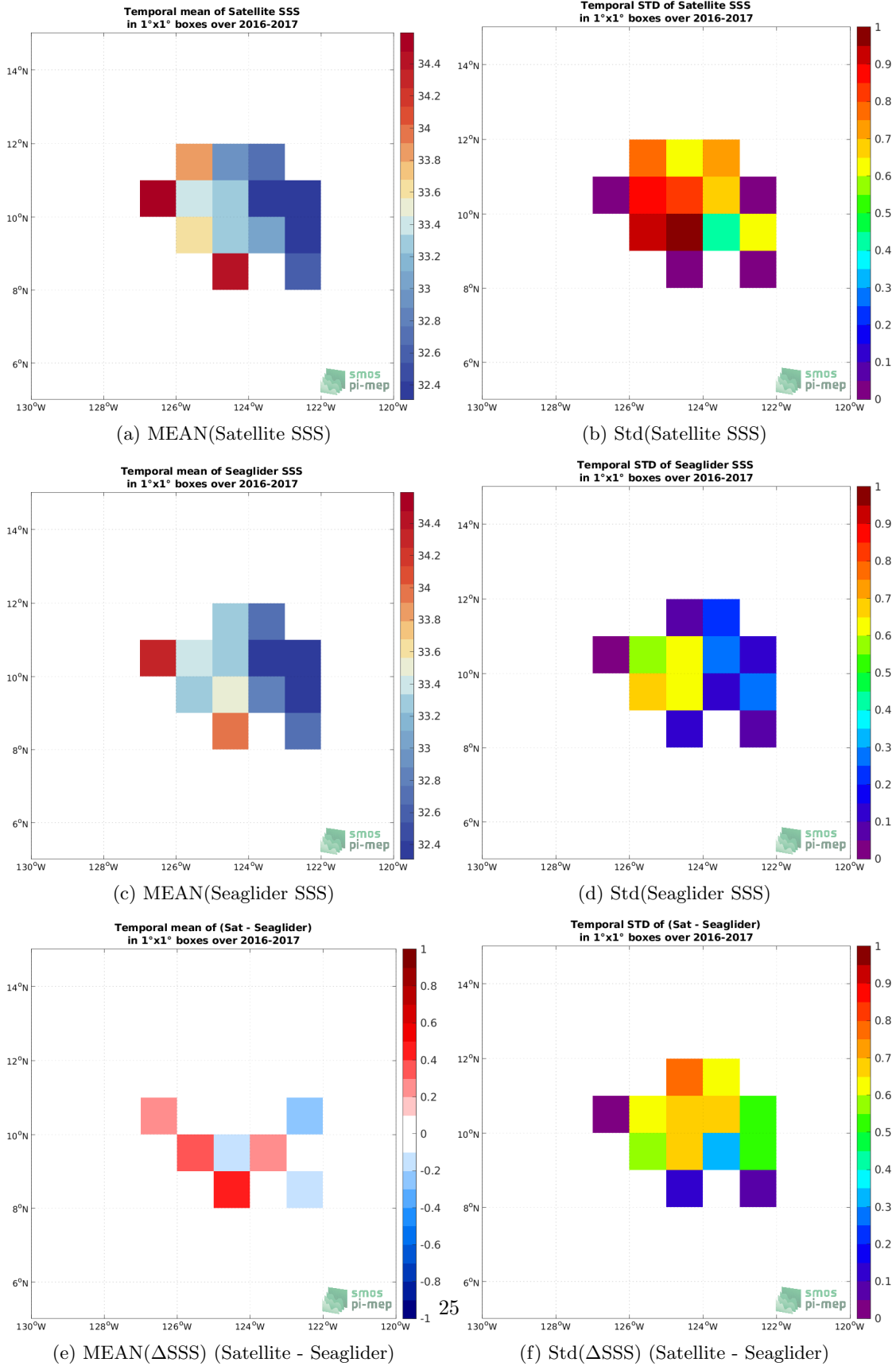
Figure 6: Temporal mean (left) and Std (right) of SSS from SMOS SSS L2 v700 (ESA) (top), Seaglider (middle), and of \Delta SSS (Satellite - Seaglider). Only match-up pairs are used to generate these maps.
