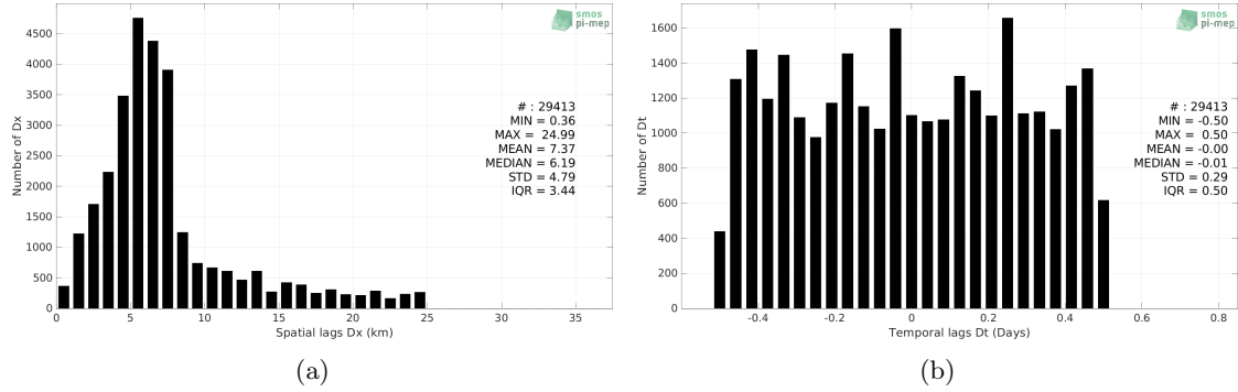
Figure 5: Histograms of the spatial (a) and temporal (b) lags between the location/time of the Seaglider measurement and the date of the corresponding SMOS SSS L2 v700 (ESA) SSS pixel.
