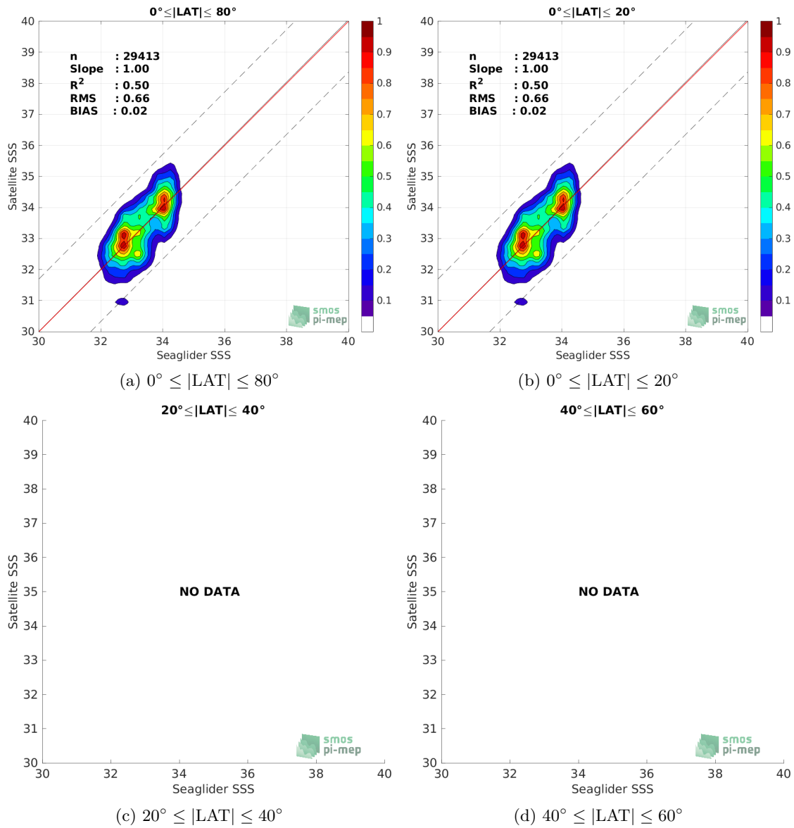
Figure 9: Contour maps of the concentration of SMOS SSS L2 v700 (ESA) SSS (y-axis) versus Seaglider SSS (x-axis) at match-up pairs for different latitude bands. For each plot, the red line shows x=y . The black thin and dashed lines indicate a linear fit through the data cloud and the \pm 95\% confidence levels, respectively. The number match-up pairs n , the slope and R^2 coefficient of the linear fit, the root mean square (RMS) and the mean bias between satellite and in situ data are indicated for each latitude band in each plots.
