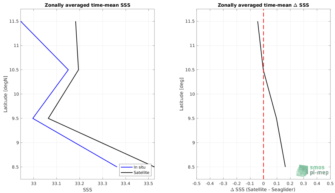
Figure 8: Left panel: Zonal mean SSS from SMOS SSS L2 v700 (ESA) satellite product (black) and from Seaglider (blue). Right panel: Zonal mean of \Delta SSS (Satellite - Seaglider) for all the collected Pi-MEP match-up pairs estimated over the full satellite product period.
