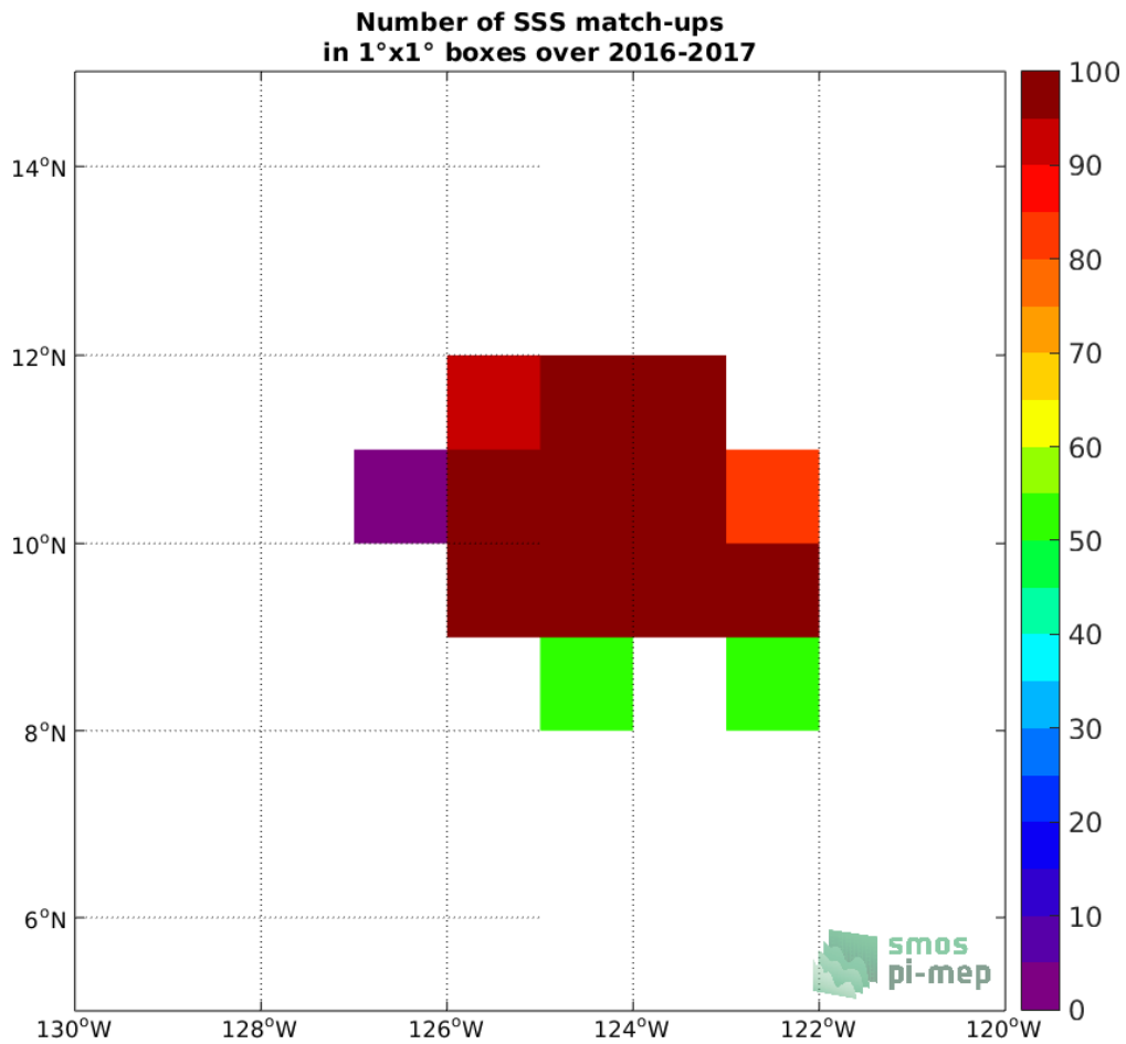
Figure 3: Number of SSS match-ups between Seaglider SSS and the SMOS SSS L2 v700 (ESA) SSS product for the SPURS 2 Pi-MEP region over 1^\circ \times 1^\circ boxes and for the full satellite product period.
