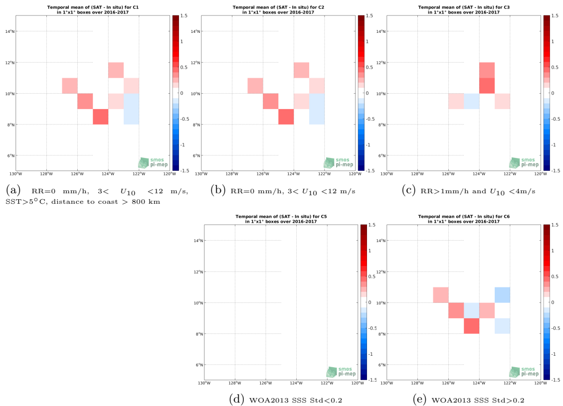
Figure 11: Temporal mean gridded over spatial boxes of size 1^\circ \times 1^\circ of \Delta SSS (SMOS SSS L2 v700 (ESA) - Seaglider) for 5 different subdatasets corresponding to:RR=0 mm/h, 3 < U_{10} < 12 m/s, SST >5^\circ C, distance to coast > 800 km (a), RR=0 mm/h, 3 < U_{10} < 12 m/s (b), RR >1 mm/h and U_{10} < 4 m/s (c), WOA2013 SSS Std <0.2 (d), WOA2013 SSS Std >0.2 (e).
