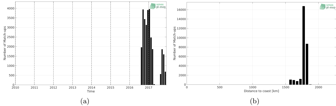
Figure 1: Number of match-ups between Seaglider and SMOS SSS L2 v700 (ESA) SSS as a function of time (a) and as function of the distance to coast (b) over the SPURS 2 Pi-MEP region and for the full satellite product period.
