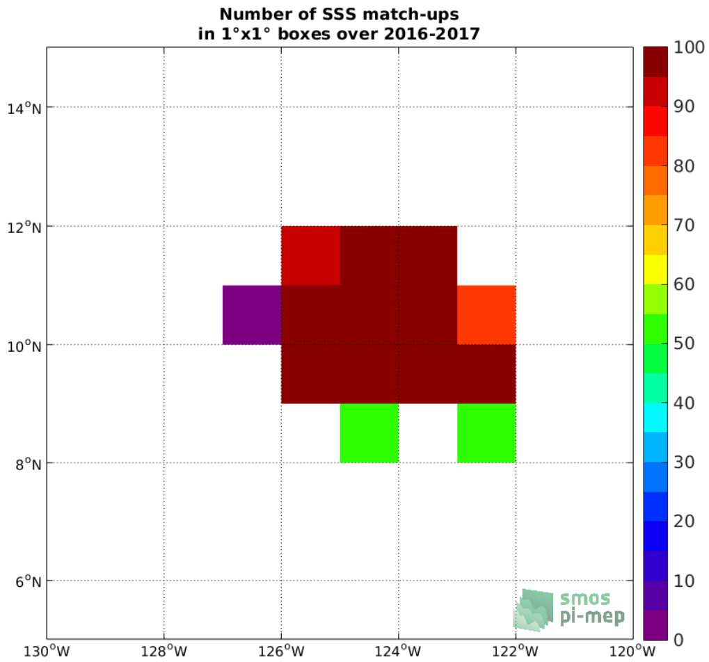
Figure 3: Number of SSS match-ups between Seaglider SSS and the SMOS SSS L2 v700 (ESA) SSS product for the SPURS 2 Pi-MEP region over 1°x1° boxes and for the full satellite product period.
