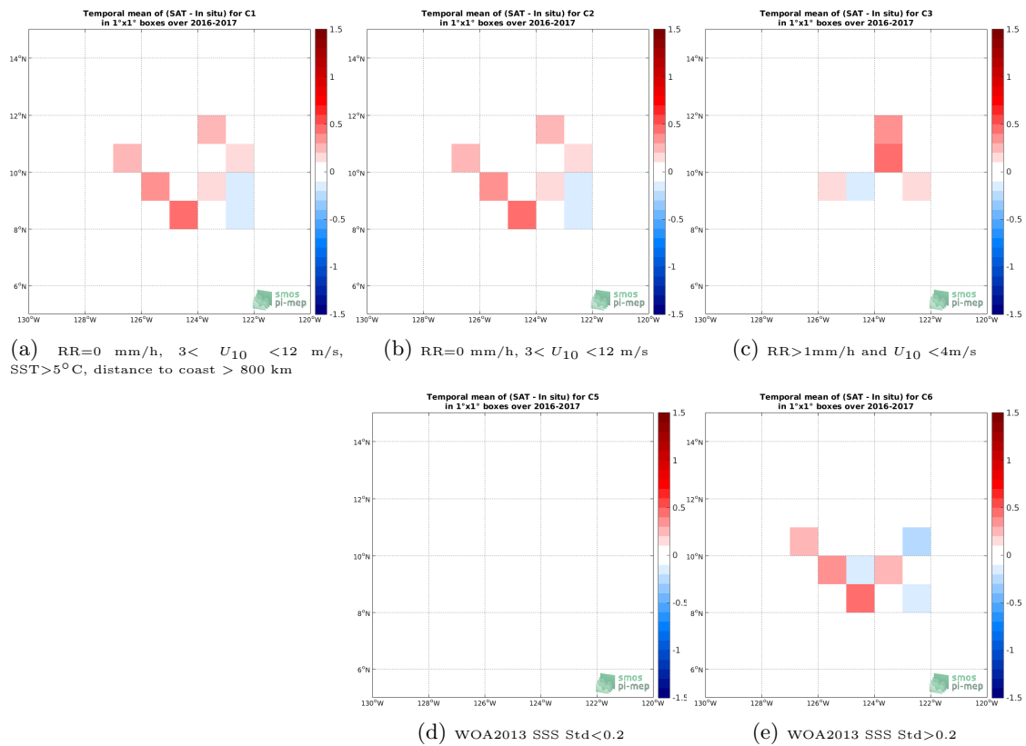
Figure 11: Temporal mean gridded over spatial boxes of size 1^\circ \times 1^\circ of \Delta SSS (SMOS SSS L2 v700 (ESA) - Seaglider) for 5 different subdatasets corresponding to:RR=0 mm/h, 3 < U_{10} < 12 m/s, SST > 5^\circ\text{C} , distance to coast > 800 km (a), RR=0 mm/h, 3 < U_{10} < 12 m/s (b), RR > 1 mm/h and U_{10} < 4 m/s (c), WOA2013 SSS Std < 0.2 (d), WOA2013 SSS Std > 0.2 (e).
