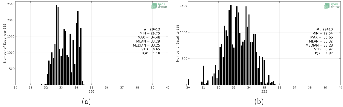
Figure 2: Histograms of SSS from Seaglider (a) and SMOS SSS L2 v700 (ESA) (b) considering all match-up pairs per bins of 0.1 over the SPURS 2 Pi-MEP region and for the full satellite product period.
