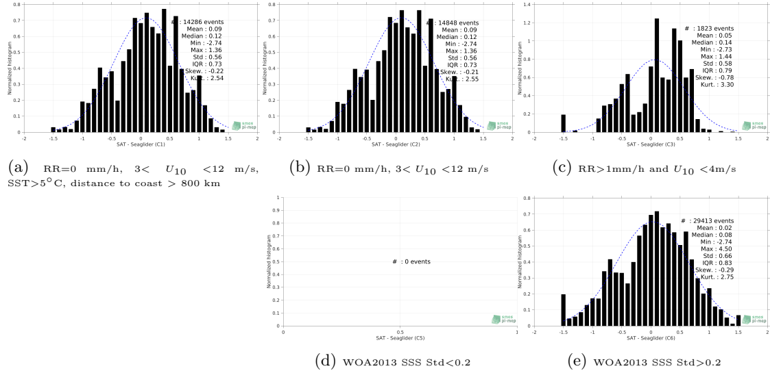
Figure 12: Normalized histogram of \Delta SSS (SMOS SSS L2 v700 (ESA) - Seaglider) for 5 different subdatasets corresponding to: RR=0 mm/h, 3 < U_{10} < 12 m/s, SST > 5°C, distance to coast > 800 km (a), RR=0 mm/h, 3 < U_{10} < 12 m/s (b), RR > 1mm/h and U_{10} < 4 m/s (c), WOA2013 SSS Std < 0.2 (d), WOA2013 SSS Std > 0.2 (e).
