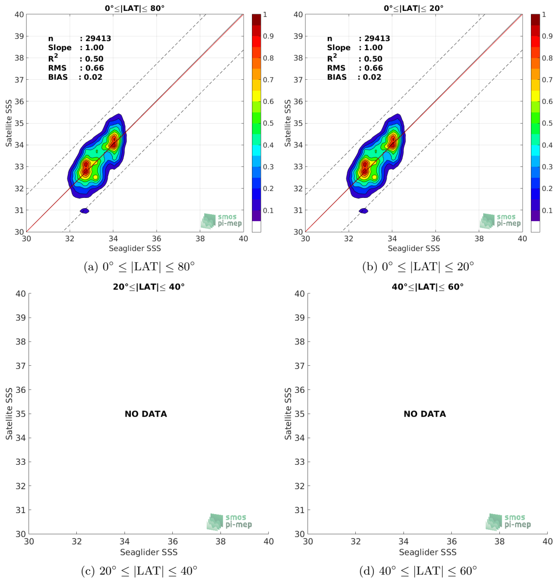
Figure 8: Contour maps of the concentration of SMOS SSS L2 v700 (ESA) SSS (y-axis) versus Seaglider SSS (x-axis) at match-up pairs for different latitude bands. For each plot, the red line shows x=y . The black thin and dashed lines indicate a linear fit through the data cloud and the \pm 95\% confidence levels, respectively. The number match-up pairs n , the slope and R^2 coefficient of the linear fit, the root mean square (RMS) and the mean bias between satellite and in situ data are indicated for each latitude band in each plots.
