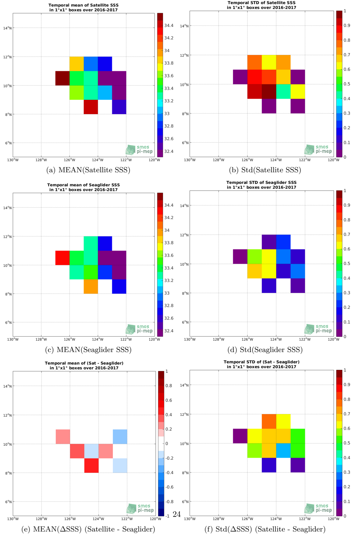
Figure 5: Temporal mean (left) and Std (right) of SSS from SMOS SSS L2 v700 (ESA) (top), Seaglider (middle), and of \Delta SSS (Satellite - Seaglider). Only match-up pairs are used to generate these maps.
