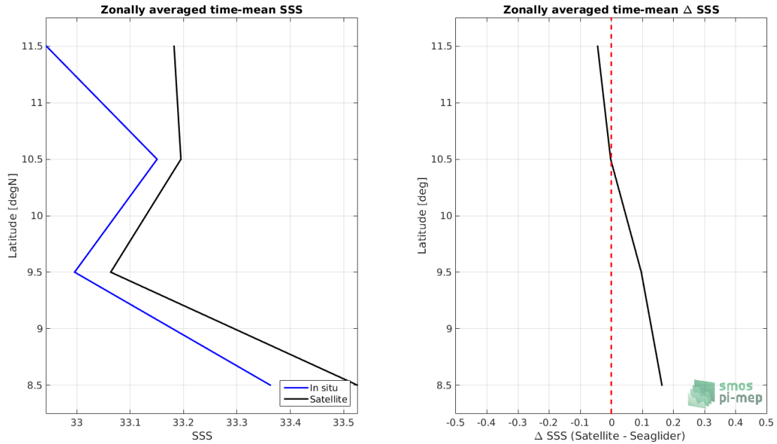
Figure 7: Left panel: Zonal mean SSS from SMOS SSS L2 v700 (ESA) satellite product (black) and from Seaglider (blue). Right panel: Zonal mean of \Delta SSS (Satellite - Seaglider) for all the collected Pi-MEP match-up pairs estimated over the full satellite product period.
