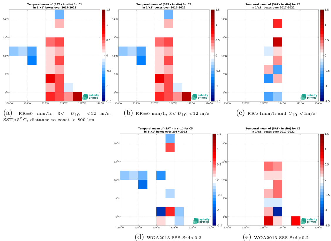
Figure 12: Temporal mean gridded over spatial boxes of size 1^\circ \times 1^\circ of \Delta SSS (SMOS SSS L2 v700 (ESA) - Saifdrone) for 5 different subdatasets corresponding to: RR=0 mm/h, 3 < U_{10} < 12 m/s, SST > 5^\circ C , distance to coast > 800 km (a), RR=0 mm/h, 3 < U_{10} < 12 m/s (b), RR > 1 mm/h and U_{10} < 4 m/s (c), WOA2013 SSS Std < 0.2 (d), WOA2013 SSS Std > 0.2 (e).
