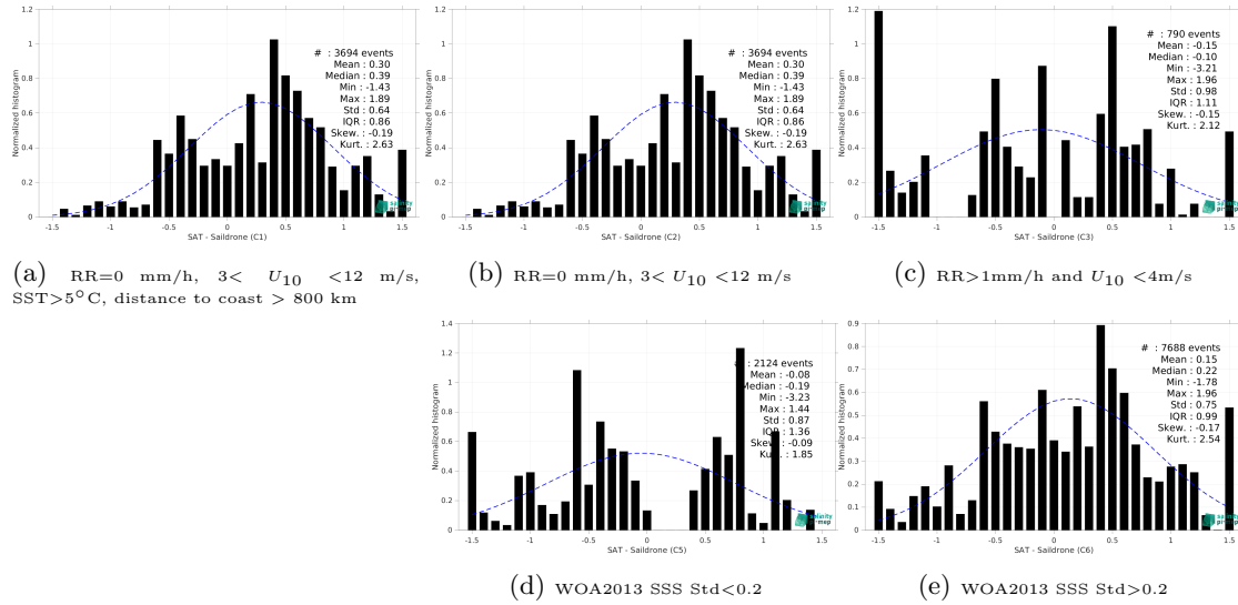
Figure 13: Normalized histogram of \Delta SSS (SMOS SSS L2 v700 (ESA) - Salldrone) for 5 different subdatasets corresponding to: RR=0 mm/h, 3 < U_{10} < 12 m/s, SST > 5°C, distance to coast > 800 km (a), RR=0 mm/h, 3 < U_{10} < 12 m/s (b), RR > 1mm/h and U_{10} < 4 m/s (c), WOA2013 SSS Std < 0.2 (d), WOA2013 SSS Std > 0.2 (e).
