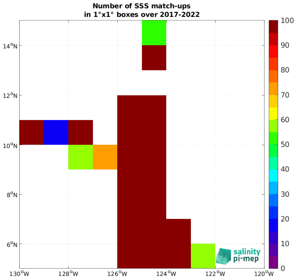
Figure 4: Number of SSS match-ups between Saildrone SSS and the SMOS SSS L2 v700 (ESA) SSS product for the SPURS 2 Pi-MEP region over 1^\circ \times 1^\circ boxes and for the full satellite product period.
