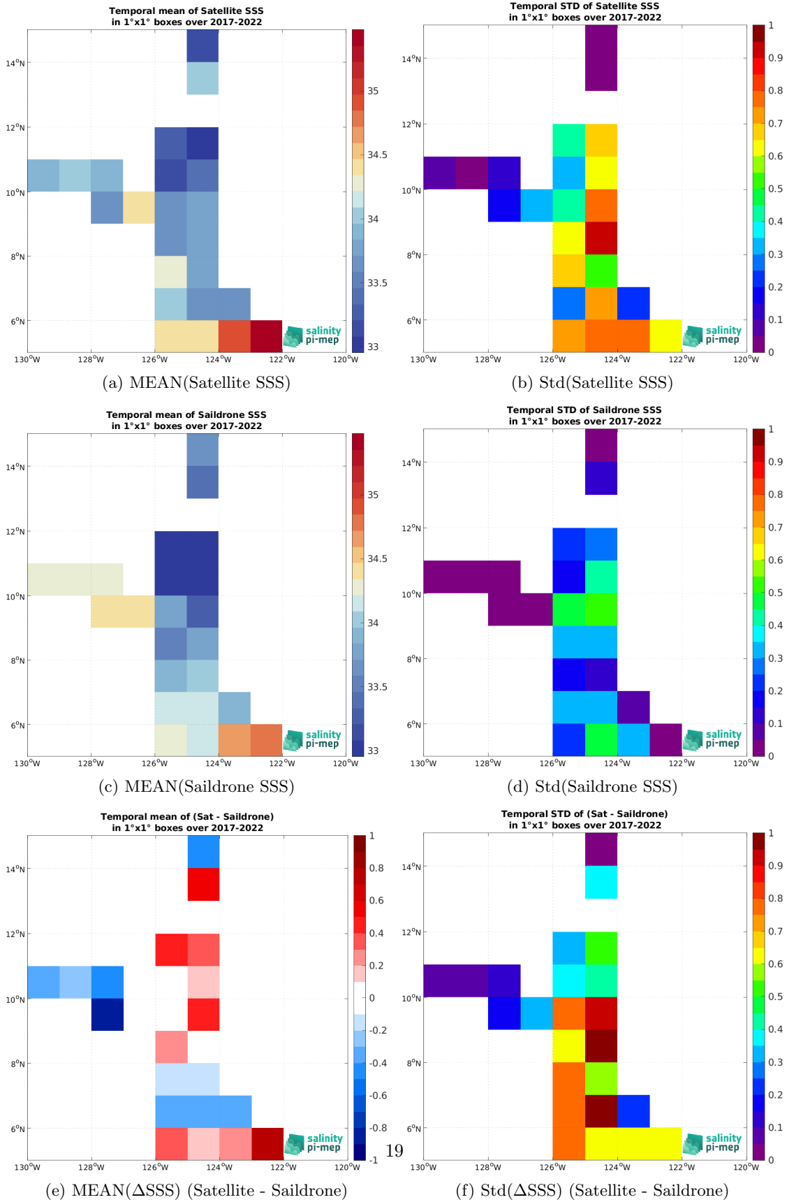
Figure 6: Temporal mean (left) and Std (right) of SSS from SMOS SSS L2 v700 (ESA) (top), Saildrone (middle), and of \Delta SSS (Satellite - Saildrone). Only match-up pairs are used to generate these maps.
