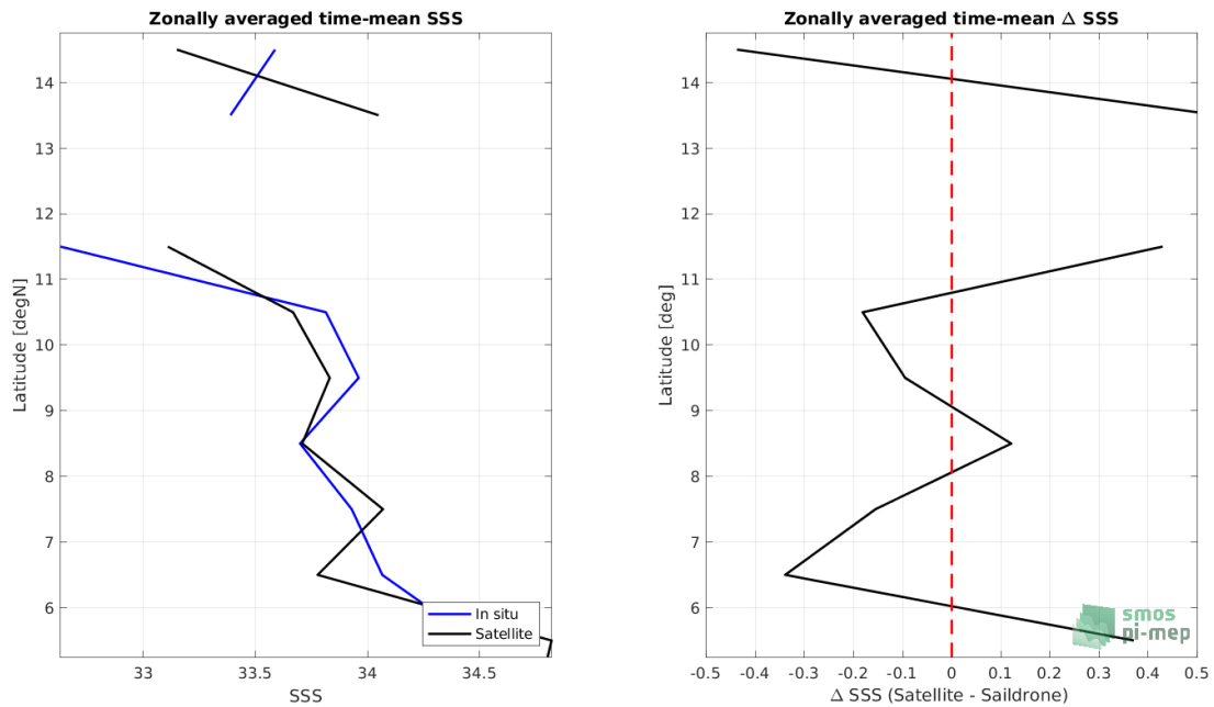
Figure 8: Left panel: Zonal mean SSS from SMOS SSS L2 v700 (ESA) satellite product (black) and from Saildrone (blue). Right panel: Zonal mean of \Delta SSS (Satellite - Saildrone) for all the collected Pi-MEP match-up pairs estimated over the full satellite product period.
