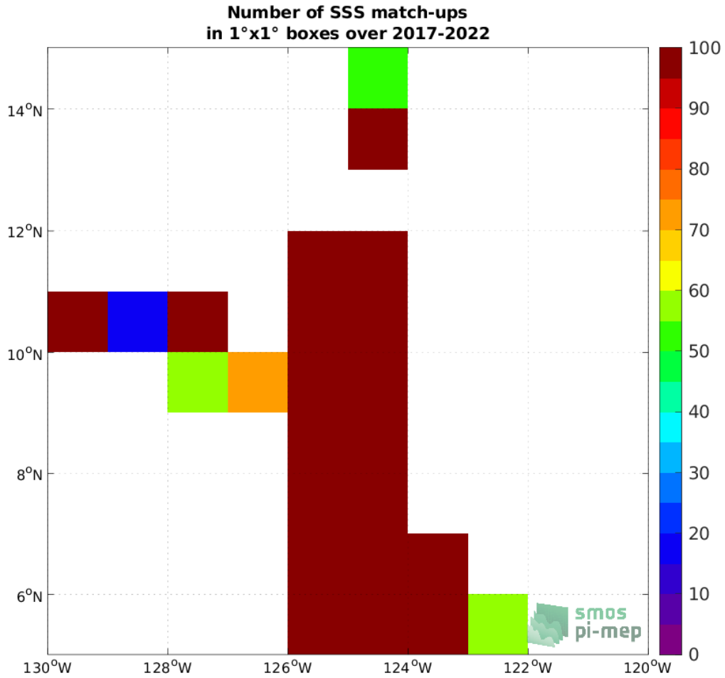
Figure 4: Number of SSS match-ups between Saildrone SSS and the SMOS SSS L2 v700 (ESA) SSS product for the SPURS 2 Pi-MEP region over 1°x1° boxes and for the full satellite product period.
