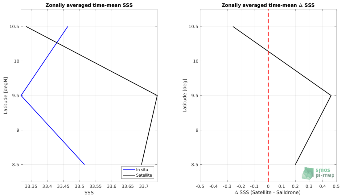
Figure 7: Left panel: Zonal mean SSS from SMOS SSS L2 v700 (ESA) satellite product (black) and from Sairdrone (blue). Right panel: Zonal mean of \Delta SSS (Satellite - Sairdrone) for all the collected Pi-MEP match-up pairs estimated over the full satellite product period.
