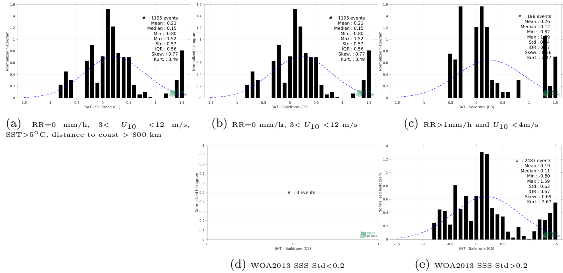
Figure 12: Normalized histogram of \Delta SSS (SMOS SSS L2 v700 (ESA) - Saildrone) for 5 different subdatasets corresponding to: RR=0 mm/h, 3 < U_{10} < 12 m/s, SST > 5°C, distance to coast > 800 km (a), RR=0 mm/h, 3 < U_{10} < 12 m/s (b), RR > 1mm/h and U_{10} < 4 m/s (c), WOA2013 SSS Std < 0.2 (d), WOA2013 SSS Std > 0.2 (e).
