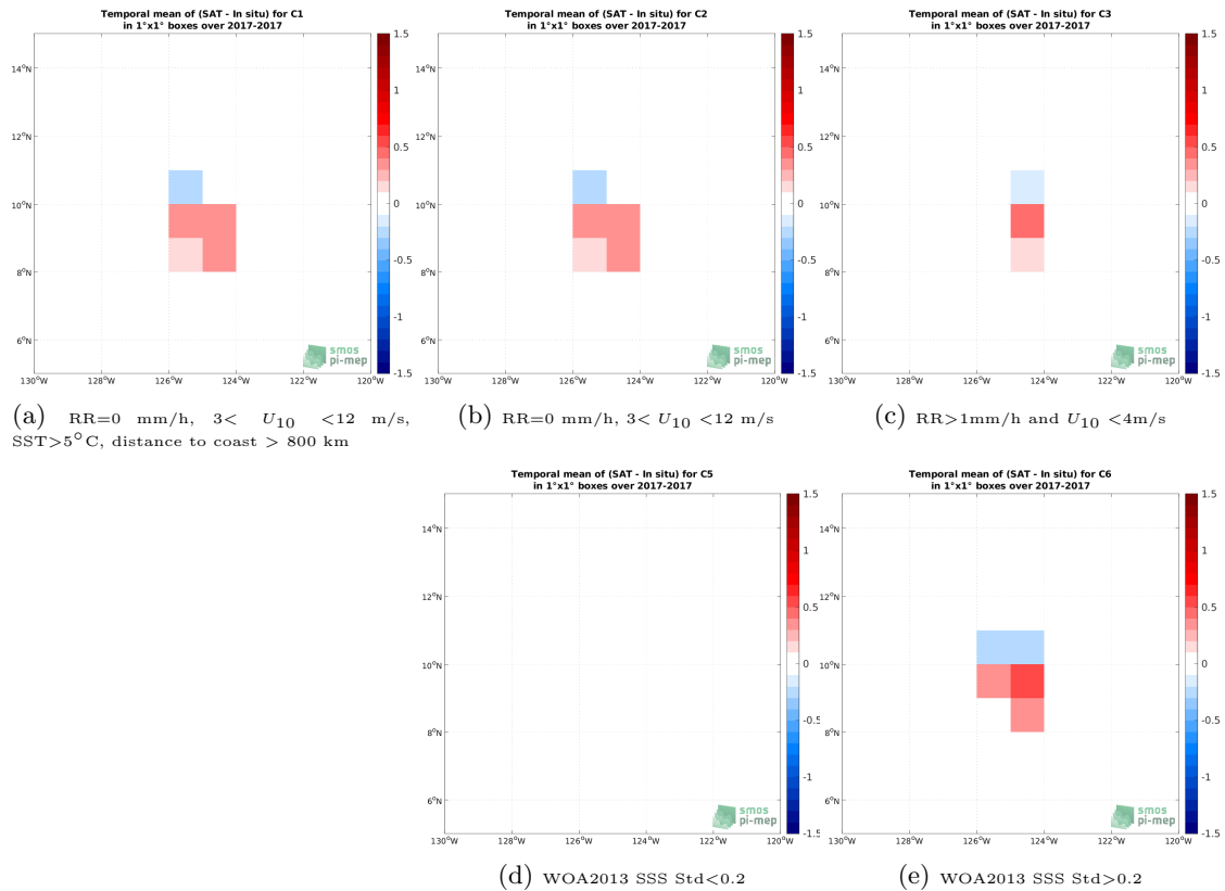
Figure 11: Temporal mean gridded over spatial boxes of size 1^\circ \times 1^\circ of \Delta SSS (SMOS SSS L2 v700 (ESA) - Saiclone) for 5 different subdatasets corresponding to:RR=0 mm/h, 3 < U_{10} < 12 m/s, SST>5°C, distance to coast > 800 km (a), RR=0 mm/h, 3 < U_{10} < 12 m/s (b), RR>1mm/h and U_{10} < 4 m/s (c), WOA2013 SSS Std<0.2 (d), WOA2013 SSS Std>0.2 (e).
