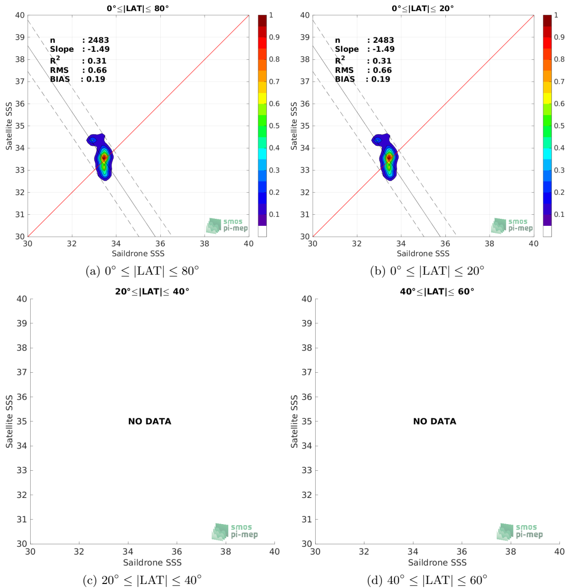
Figure 8: Contour maps of the concentration of SMOS SSS L2 v700 (ESA) SSS (y-axis) versus Saildrone SSS (x-axis) at match-up pairs for different latitude bands. For each plot, the red line shows x=y . The black thin and dashed lines indicate a linear fit through the data cloud and the \pm 95\% confidence levels, respectively. The number match-up pairs n , the slope and R^2 coefficient of the linear fit, the root mean square (RMS) and the mean bias between satellite and in situ data are indicated for each latitude band in each plots.
