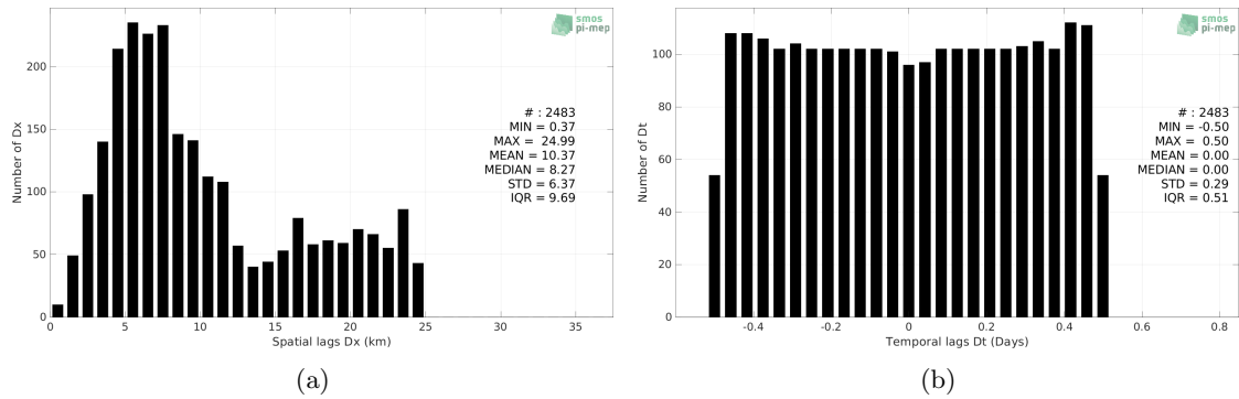
Figure 4: Histograms of the spatial (a) and temporal (b) lags between the location/time of the Saildrone measurement and the date of the corresponding SMOS SSS L2 v700 (ESA) SSS pixel.
