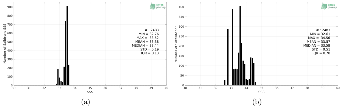
Figure 2: Histograms of SSS from Saildrone (a) and SMOS SSS L2 v700 (ESA) (b) considering all match-up pairs per bins of 0.1 over the SPURS 2 Pi-MEP region and for the full satellite product period.
