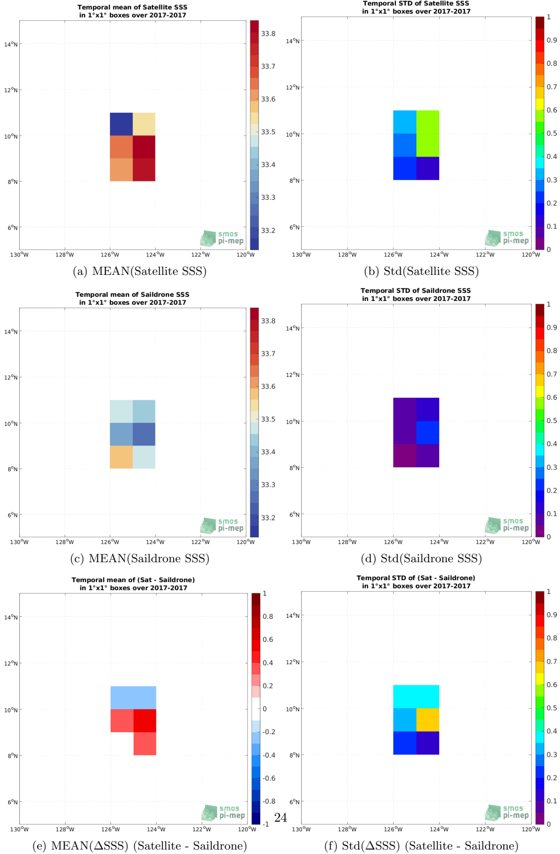
Figure 5: Temporal mean (left) and Std (right) of SSS from SMOS SSS L2 v700 (ESA) (top), Saildrone (middle), and of \Delta SSS (Satellite - Saildrone). Only match-up pairs are used to generate these maps.
