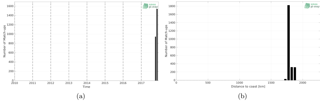
Figure 1: Number of match-ups between Saildrone and SMOS SSS L2 v700 (ESA) SSS as a function of time (a) and as function of the distance to coast (b) over the SPURS 2 Pi-MEP region and for the full satellite product period.
