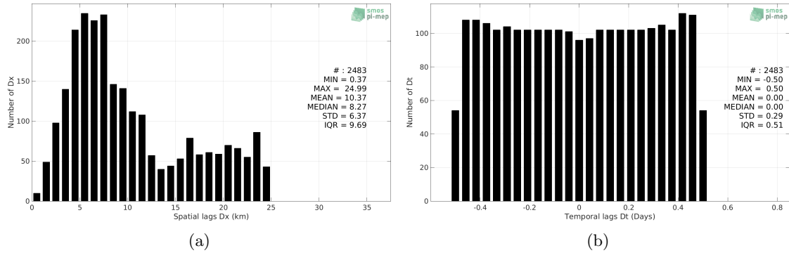
Figure 4: Histograms of the spatial (a) and temporal (b) lags between the location/time of the Sairdrone measurement and the date of the corresponding SMOS SSS L2 v700 (ESA) SSS pixel.
