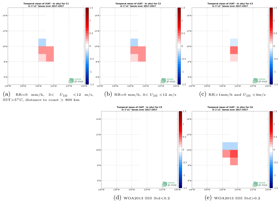
Figure 11: Temporal mean gridded over spatial boxes of size 1^\circ \times 1^\circ of \Delta\text{SSS} (SMOS SSS L2 v700 (ESA) - Saildrone) for 5 different subdatasets corresponding to:RR=0 mm/h, 3 < U_{10} < 12 m/s, SST >5^\circ\text{C} , distance to coast > 800 km (a), RR=0 mm/h, 3 < U_{10} < 12 m/s (b), RR >1 mm/h and U_{10} < 4 m/s (c), WOA2013 SSS Std <0.2 (d), WOA2013 SSS Std >0.2 (e).
