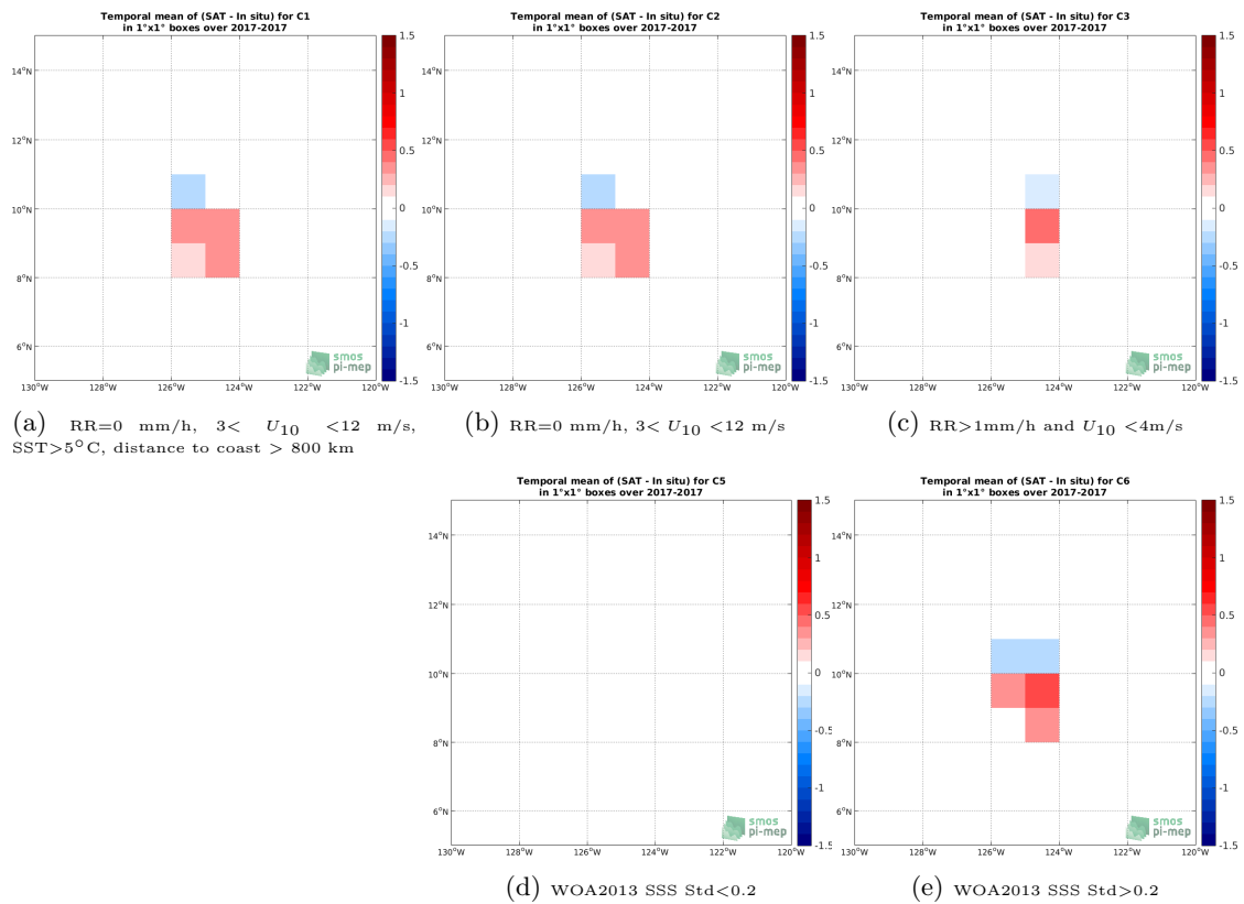
Figure 11: Temporal mean gridded over spatial boxes of size 1^\circ \times 1^\circ of \Delta SSS (SMOS SSS L2 v700 (ESA) - Sairdrone) for 5 different subdatasets corresponding to:RR=0 mm/h, 3 < U_{10} < 12 m/s, SST >5^\circ\text{C} , distance to coast > 800 km (a), RR=0 mm/h, 3 < U_{10} < 12 m/s (b), RR >1 mm/h and U_{10} < 4 m/s (c), WOA2013 SSS Std <0.2 (d), WOA2013 SSS Std >0.2 (e).
