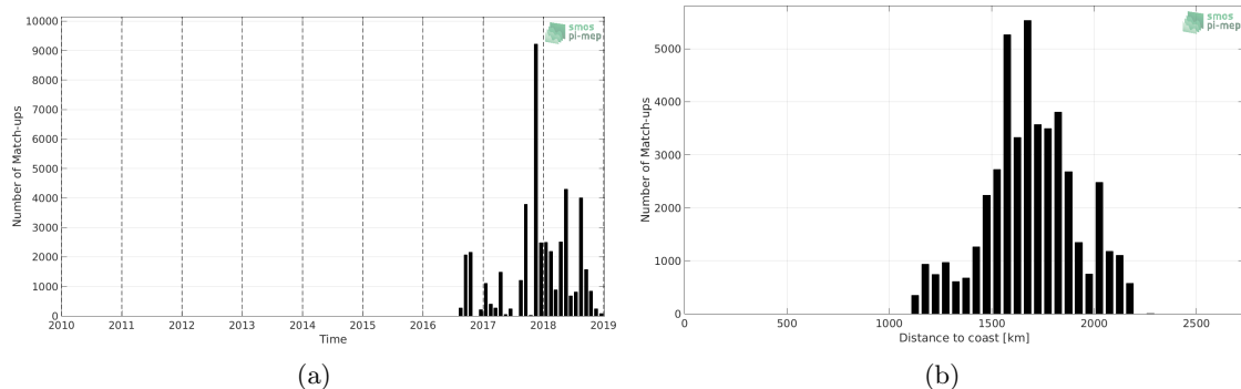
Figure 1: Number of match-ups between Surface drifters and SMOS SSS L2 v700 (ESA) SSS as a function of time (a) and as function of the distance to coast (b) over the SPURS 2 Pi-MEP region and for the full satellite product period.
