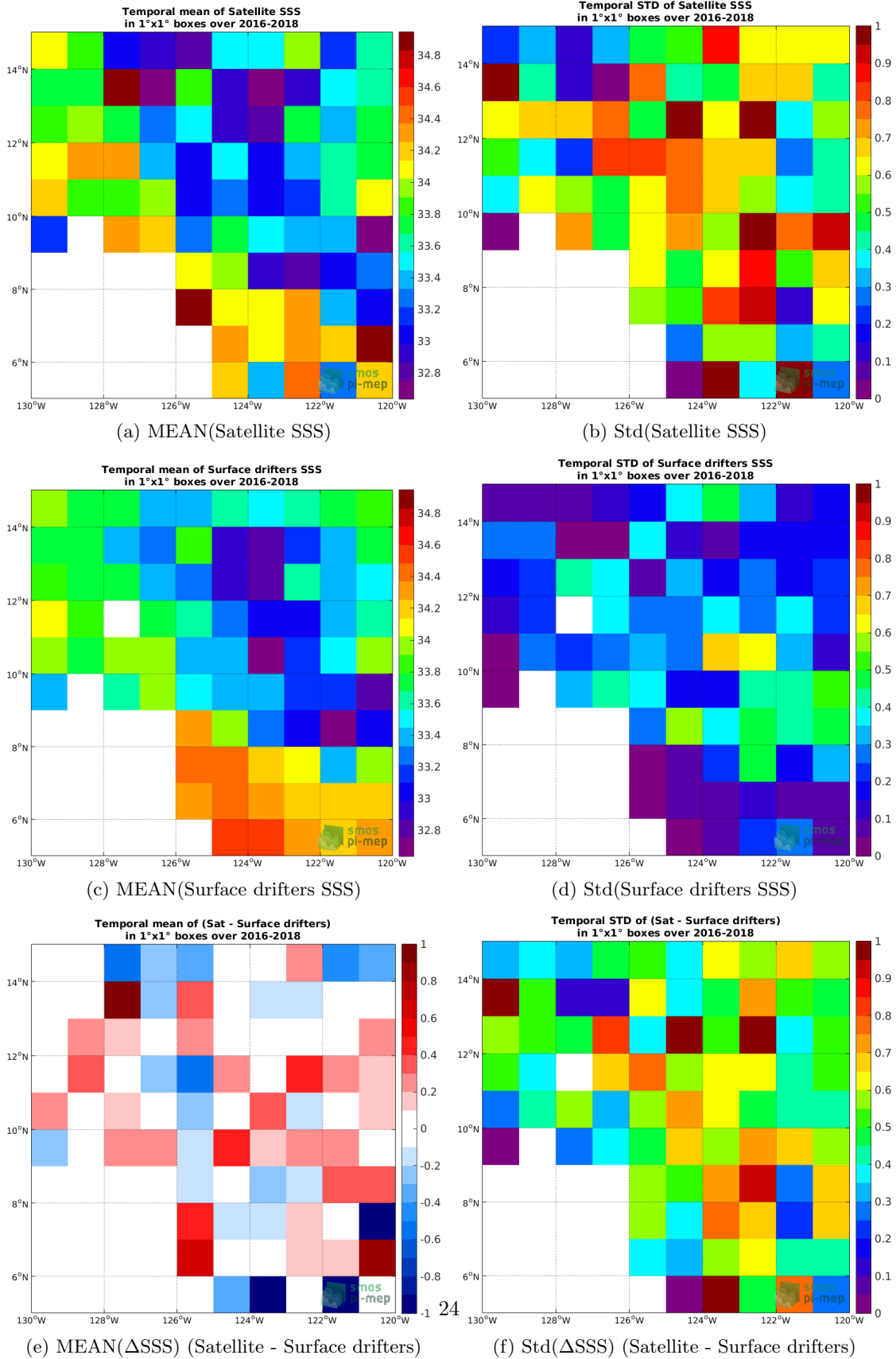
Figure 5: Temporal mean (left) and Std (right) of SSS from SMOS SSS L2 v700 (ESA) (top), Surface drifters (middle), and of \Delta SSS (Satellite - Surface drifters). Only match-up pairs are used to generate these maps.
