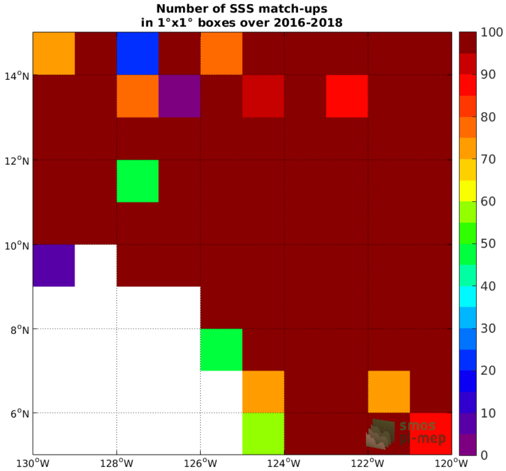
Figure 3: Number of SSS match-ups between Surface drifters SSS and the SMOS SSS L2 v700 (ESA) SSS product for the SPURS 2 Pi-MEP region over 1°x1° boxes and for the full satellite product period.
