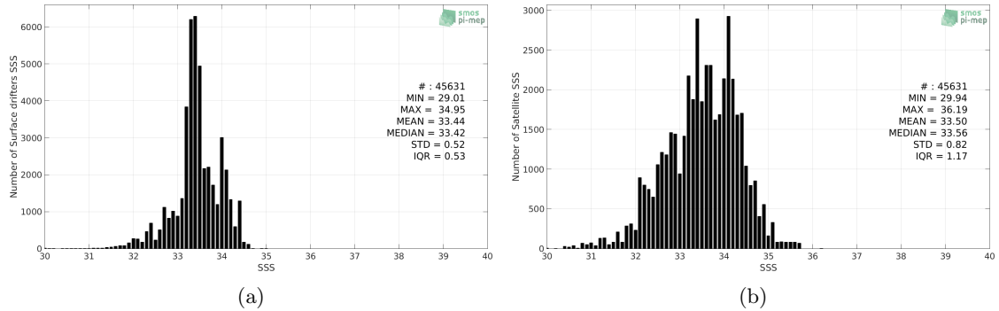
Figure 2: Histograms of SSS from Surface drifters (a) and SMOS SSS L2 v700 (ESA) (b) considering all match-up pairs per bins of 0.1 over the SPURS 2 Pi-MEP region and for the full satellite product period.
