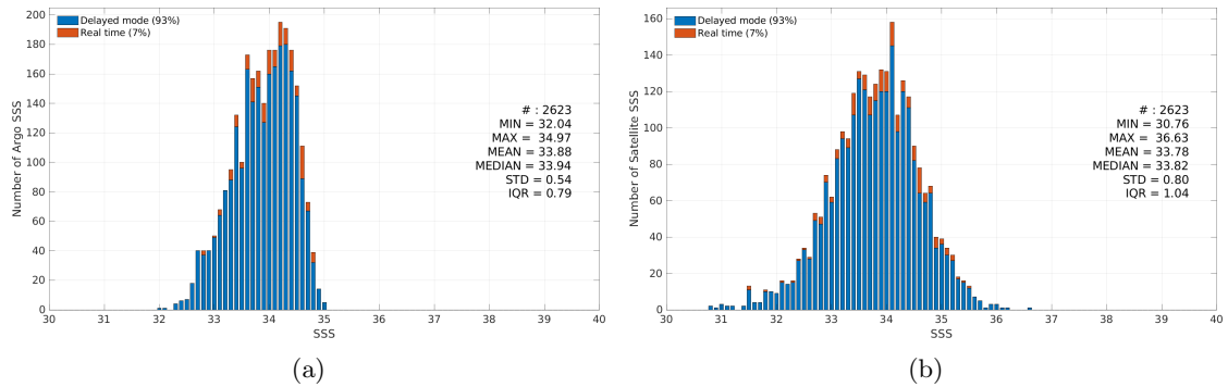
Figure 3: Histograms of SSS from Argo (a) and SMOS SSS L2 v700 (ESA) (b) considering all match-up pairs per bins of 0.1 over the SPURS 2 Pi-MEP region and for the full satellite product period.
