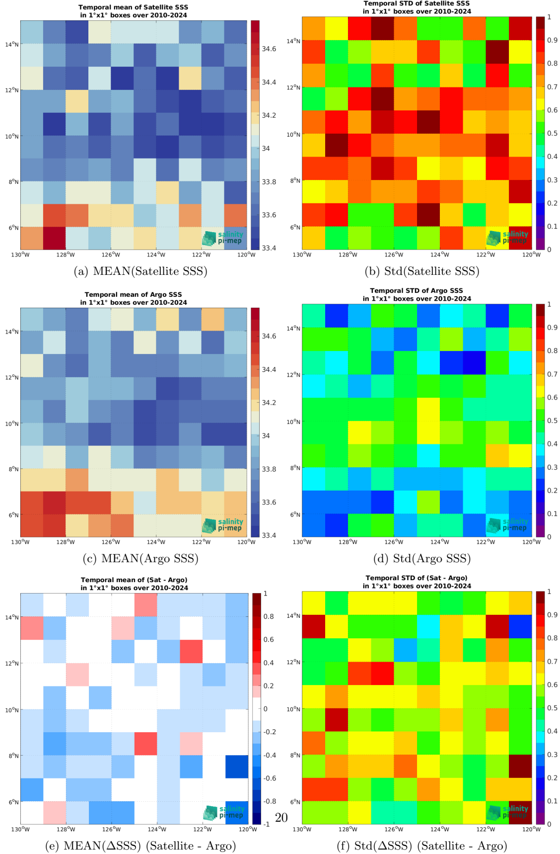
Figure 7: Temporal mean (left) and Std (right) of SSS from SMOS SSS L2 v700 (ESA) (top), Argo (middle), and of \Delta SSS (Satellite - Argo). Only match-up pairs are used to generate these maps.
