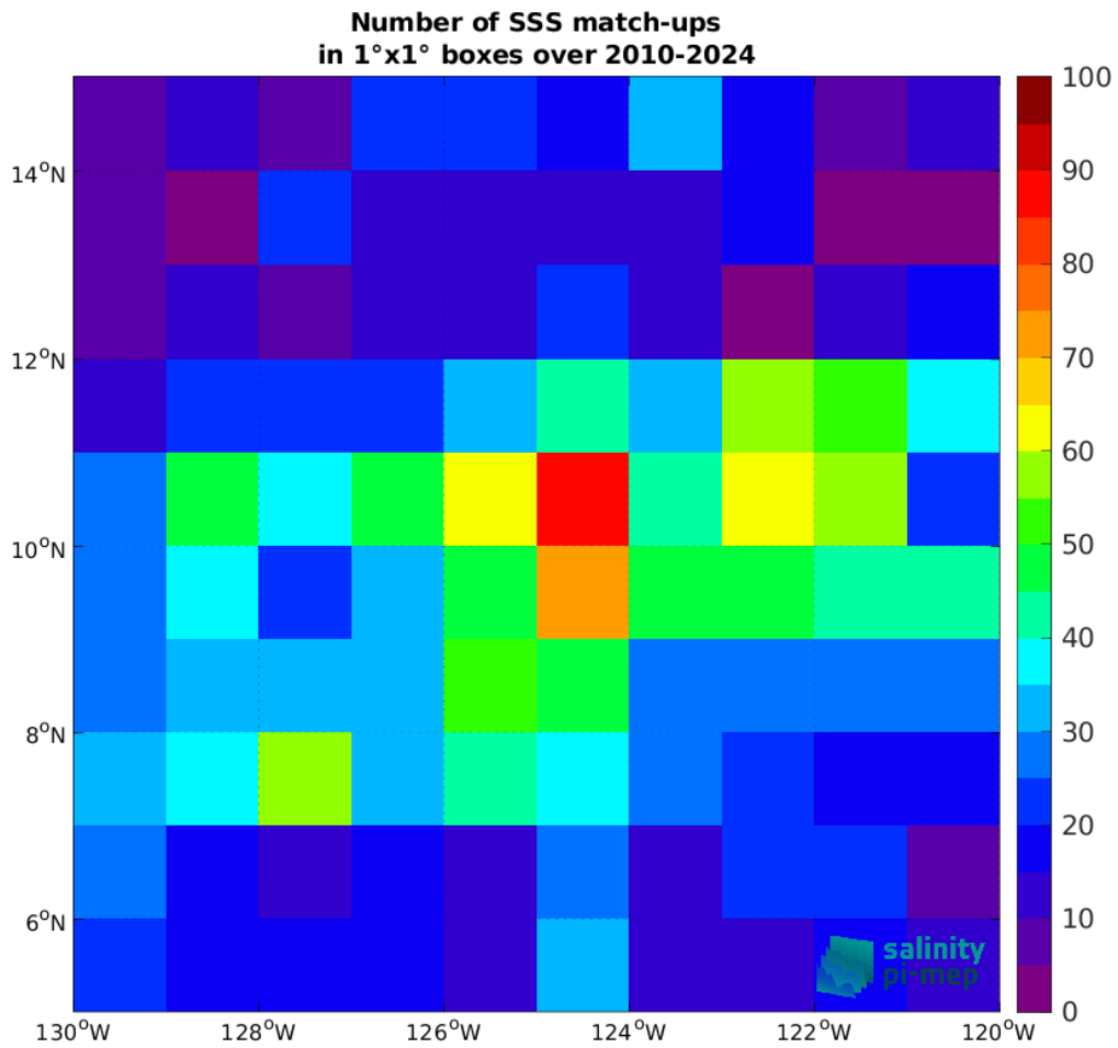
Figure 5: Number of SSS match-ups between Argo SSS and the SMOS SSS L2 v700 (ESA) SSS product for the SPURS 2 Pi-MEP region over 1°x1° boxes and for the full satellite product period.
