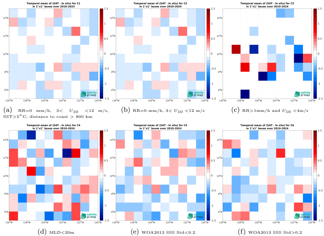
Figure 14: Temporal mean gridded over spatial boxes of size 1^\circ \times 1^\circ of \Delta SSS (SMOS SSS L2 v700 (ESA) - Argo) for 6 different subdatasets corresponding to:RR=0 mm/h, 3 < U_{10} < 12 m/s, SST >5^\circ\text{C} , distance to coast > 800 km (a), RR=0 mm/h, 3 < U_{10} < 12 m/s (b), RR >1 mm/h and U_{10} < 4 m/s (c),MLD <20 m (d),WOA2013 SSS Std <0.2 (e),WOA2013 SSS Std >0.2 (f).
