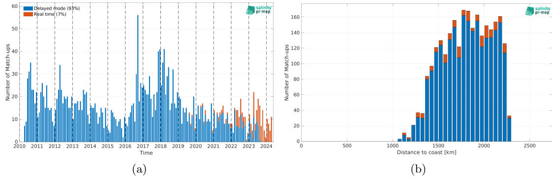
Figure 2: Number of match-ups between Argo and SMOS SSS L2 v700 (ESA) SSS as a function of time (a) and as function of the distance to coast (b) over the SPURS 2 Pi-MEP region and for the full satellite product period.
