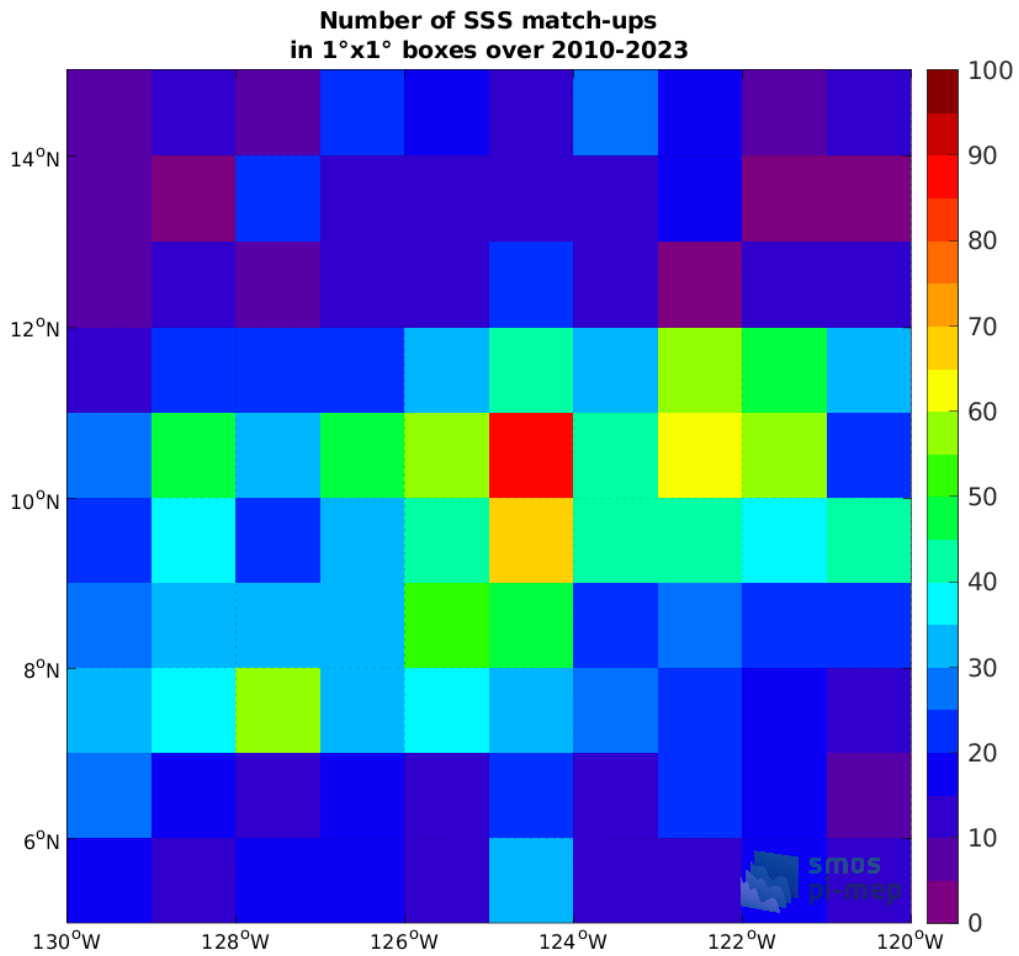
Figure 4: Number of SSS match-ups between Argo SSS and the SMOS SSS L2 v700 (ESA) SSS product for the SPURS 2 Pi-MEP region over 1°x1° boxes and for the full satellite product period.
