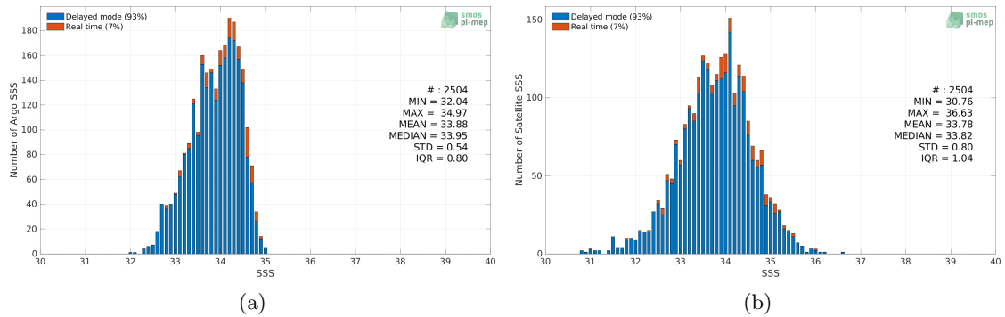
Figure 2: Histograms of SSS from Argo (a) and SMOS SSS L2 v700 (ESA) (b) considering all match-up pairs per bins of 0.1 over the SPURS 2 Pi-MEP region and for the full satellite product period.
