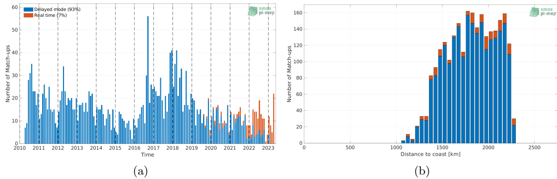
Figure 1: Number of match-ups between Argo and SMOS SSS L2 v700 (ESA) SSS as a function of time (a) and as function of the distance to coast (b) over the SPURS 2 Pi-MEP region and for the full satellite product period.
