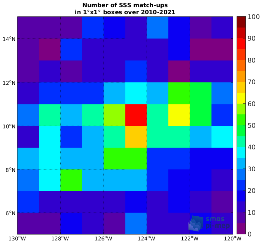
Figure 4: Number of SSS match-ups between Argo SSS and the SMOS SSS L2 v700 (ESA) SSS product for the SPURS 2 Pi-MEP region over 1°x1° boxes and for the full satellite product period.
