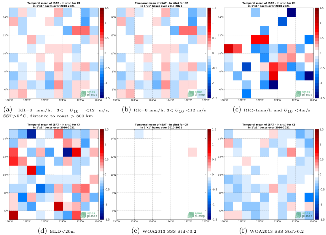
Figure 12: Temporal mean gridded over spatial boxes of size 1^\circ \times 1^\circ of \Delta SSS (SMOS SSS L2 v700 (ESA) - Argo) for 6 different subdatasets corresponding to:RR=0 mm/h, 3 < U_{10} < 12 m/s, SST >5^\circ C, distance to coast > 800 km (a), RR=0 mm/h, 3 < U_{10} < 12 m/s (b), RR >1 mm/h and U_{10} < 4 m/s (c),MLD <20 m (d),WOA2013 SSS Std <0.2 (e),WOA2013 SSS Std >0.2 (f).
