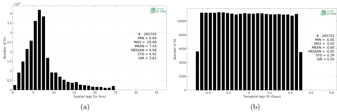
Figure 4: Histograms of the spatial (a) and temporal (b) lags between the location/time of the Waveglider measurement and the date of the corresponding SMOS SSS L2 v662 (ESA) SSS pixel.
