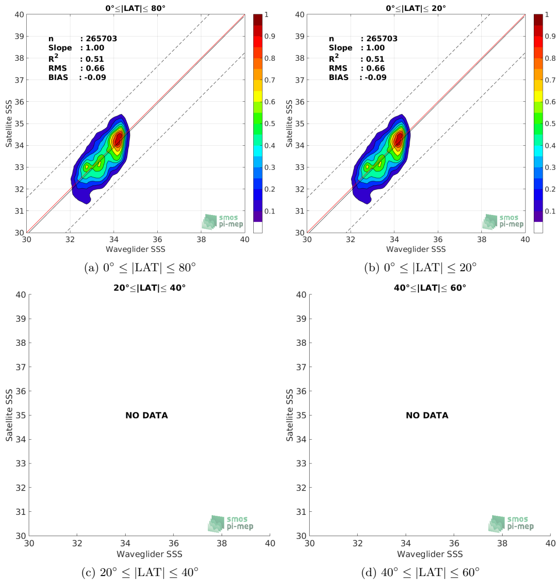
Figure 8: Contour maps of the concentration of SMOS SSS L2 v662 (ESA) SSS (y-axis) versus Waveglider SSS (x-axis) at match-up pairs for different latitude bands. For each plot, the red line shows x=y . The black thin and dashed lines indicate a linear fit through the data cloud and the \pm 95\% confidence levels, respectively. The number match-up pairs n , the slope and R^2 coefficient of the linear fit, the root mean square (RMS) and the mean bias between satellite and in situ data are indicated for each latitude band in each plots.
