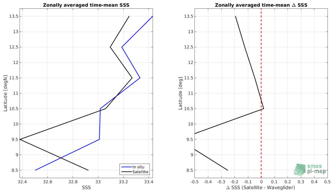
Figure 7: Left panel: Zonal mean SSS from SMOS SSS L2 v662 (ESA) satellite product (black) and from Waveglider (blue). Right panel: Zonal mean of \Delta SSS (Satellite - Waveglider) for all the collected Pi-MEP match-up pairs estimated over the full satellite product period.
