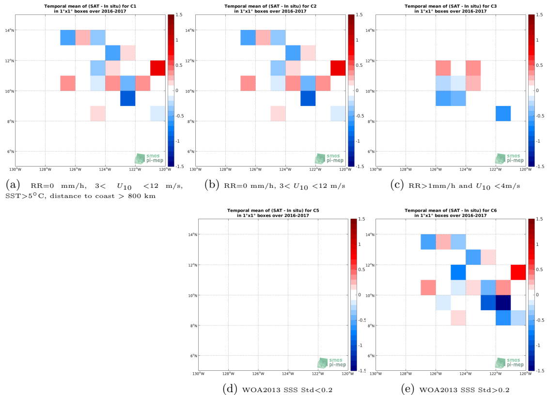
Figure 11: Temporal mean gridded over spatial boxes of size 1°x1° of \Delta SSS (SMOS SSS L2 v662 (ESA) - Waveglider) for 5 different subdatasets corresponding to: RR=0 mm/h, 3 < U_{10} < 12 m/s, SST > 5°C, distance to coast > 800 km (a), RR=0 mm/h, 3 < U_{10} < 12 m/s (b), RR > 1mm/h and U_{10} < 4 m/s (c), WOA2013 SSS Std < 0.2 (d), WOA2013 SSS Std > 0.2 (e).
