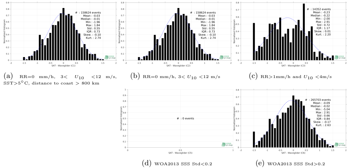
Figure 12: Normalized histogram of \Delta SSS (SMOS SSS L2 v662 (ESA) - Waveglider) for 5 different subdatasets corresponding to: RR=0 mm/h, 3 < U_{10} < 12 m/s, SST>5°C, distance to coast > 800 km (a), RR=0 mm/h, 3 < U_{10} < 12 m/s (b), RR>1mm/h and U_{10} < 4 m/s (c), WOA2013 SSS Std<0.2 (d), WOA2013 SSS Std>0.2 (e).
