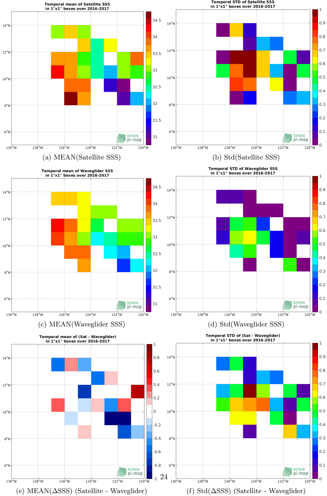
Figure 5: Temporal mean (left) and Std (right) of SSS from SMOS SSS L2 v662 (ESA) (top), Waveglider (middle), and of \Delta SSS (Satellite - Waveglider). Only match-up pairs are used to generate these maps.
