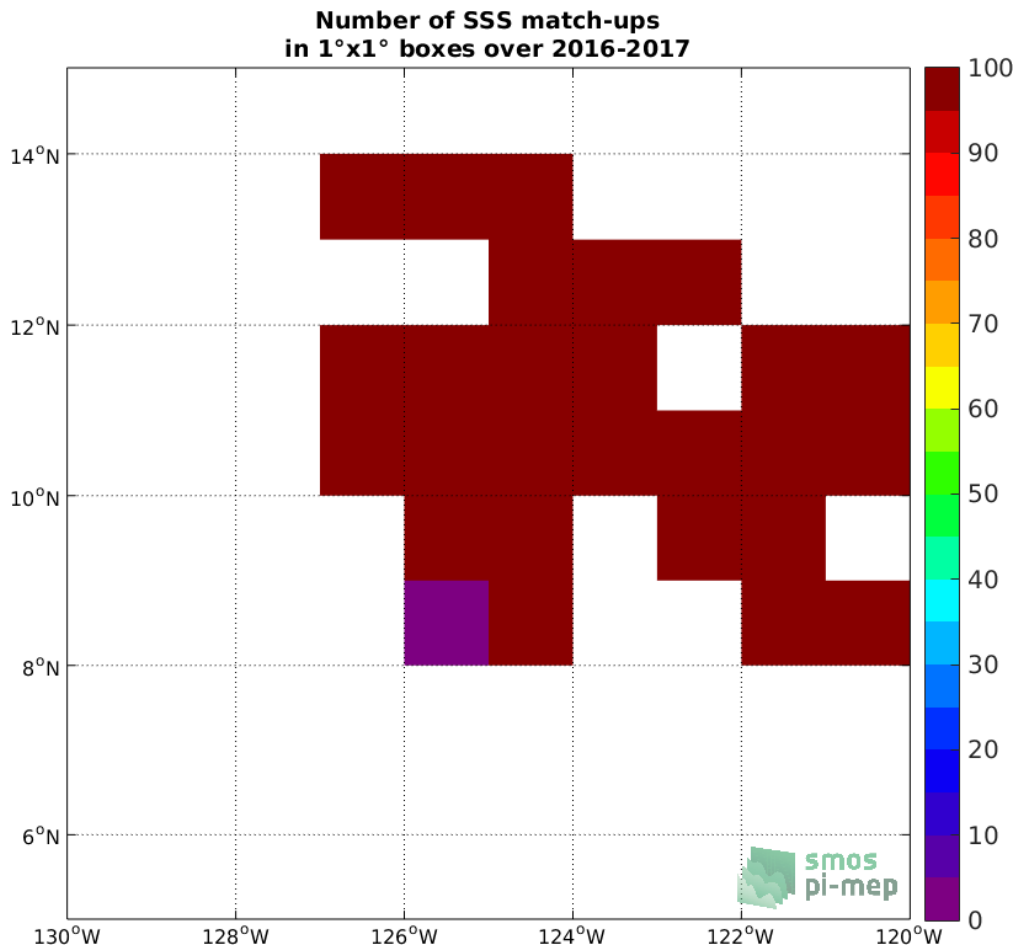
Figure 3: Number of SSS match-ups between Waveglider SSS and the SMOS SSS L2 v662 (ESA) SSS product for the SPURS 2 Pi-MEP region over 1°x1° boxes and for the full satellite product period.
