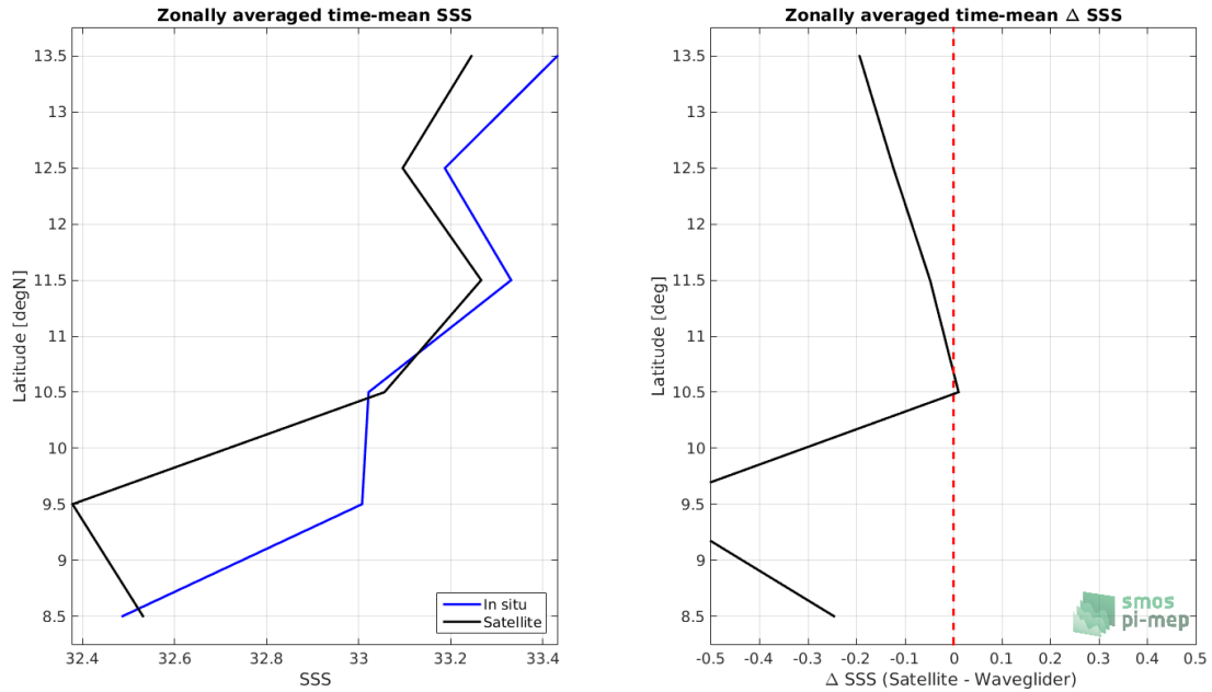
Figure 8: Left panel: Zonal mean SSS from SMOS SSS L2 v662 (ESA) satellite product (black) and from Waveglider (blue). Right panel: Zonal mean of \Delta SSS (Satellite - Waveglider) for all the collected Pi-MEP match-up pairs estimated over the full satellite product period.
