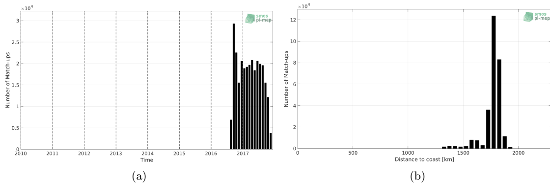
Figure 1: Number of match-ups between Waveglider and SMOS SSS L2 v662 (ESA) SSS as a function of time (a) and as function of the distance to coast (b) over the SPURS 2 Pi-MEP region and for the full satellite product period.
