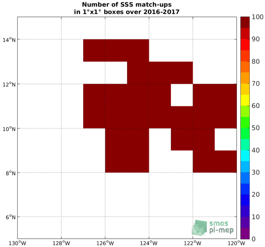
Figure 4: Number of SSS match-ups between Waveglider SSS and the SMOS SSS L2 v662 (ESA) SSS product for the SPURS 2 Pi-MEP region over 1°x1° boxes and for the full satellite product period.
