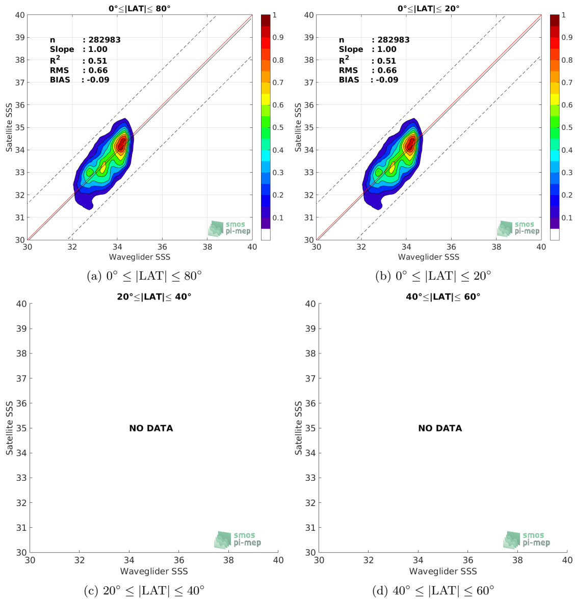
Figure 9: Contour maps of the concentration of SMOS SSS L2 v662 (ESA) SSS (y-axis) versus Waveglider SSS (x-axis) at match-up pairs for different latitude bands. For each plot, the red line shows x=y . The black thin and dashed lines indicate a linear fit through the data cloud and the \pm 95\% confidence levels, respectively. The number match-up pairs n , the slope and R^2 coefficient of the linear fit, the root mean square (RMS) and the mean bias between satellite and in situ data are indicated for each latitude band in each plots.
