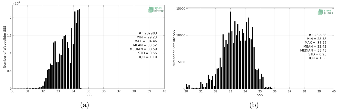
Figure 2: Histograms of SSS from Waveglider (a) and SMOS SSS L2 v662 (ESA) (b) considering all match-up pairs per bins of 0.1 over the SPURS 2 Pi-MEP region and for the full satellite product period.
