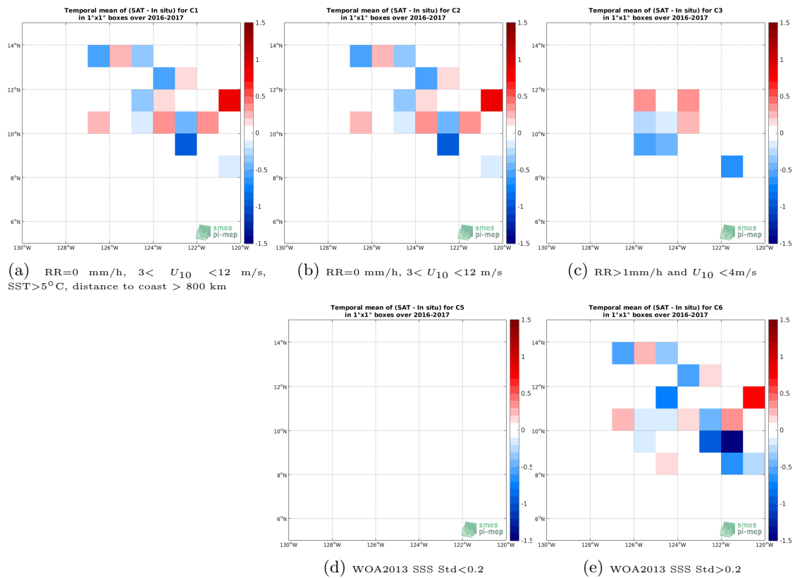
Figure 12: Temporal mean gridded over spatial boxes of size 1^\circ \times 1^\circ of \Delta SSS (SMOS SSS L2 v662 (ESA) - Waveglider) for 5 different subdatasets corresponding to:RR=0 mm/h, 3 < U_{10} < 12 m/s, SST >5^\circ\text{C} , distance to coast > 800 km (a), RR=0 mm/h, 3 < U_{10} < 12 m/s (b), RR >1 mm/h and U_{10} < 4 m/s (c), WOA2013 SSS Std <0.2 (d), WOA2013 SSS Std >0.2 (e).
