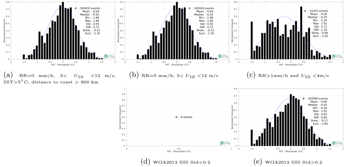
Figure 13: Normalized histogram of \Delta SSS (SMOS SSS L2 v662 (ESA) - Waveglider) for 5 different subdatasets corresponding to: RR=0 mm/h, 3 < U_{10} < 12 m/s, SST > 5°C, distance to coast > 800 km (a), RR=0 mm/h, 3 < U_{10} < 12 m/s (b), RR > 1mm/h and U_{10} < 4 m/s (c), WOA2013 SSS Std < 0.2 (d), WOA2013 SSS Std > 0.2 (e).
