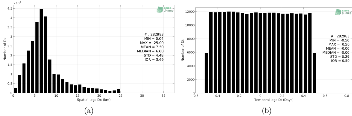
Figure 5: Histograms of the spatial (a) and temporal (b) lags between the time of the Waveglider measurements and the date of the corresponding SMOS SSS L2 v662 (ESA) SSS product.
