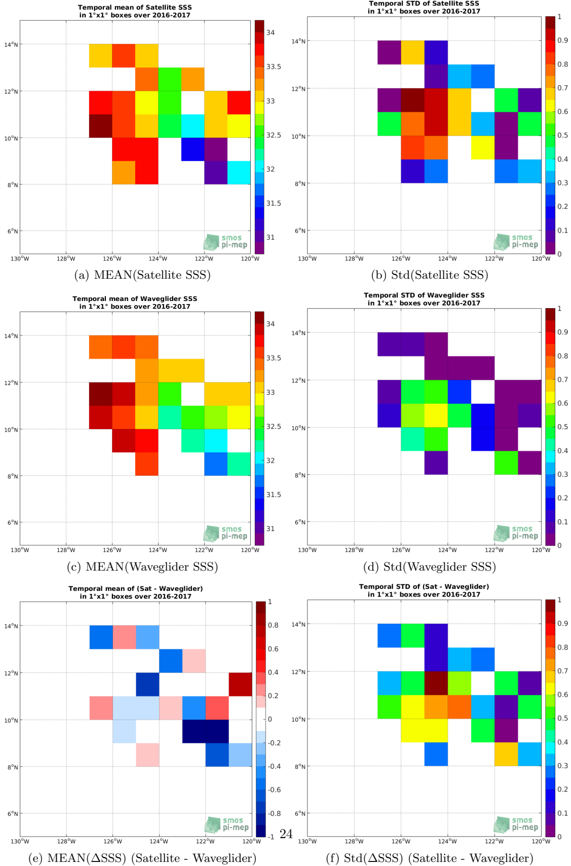
Figure 6: Temporal mean (left) and Std (right) of SSS from SMOS SSS L2 v662 (ESA) (top), Waveglider (middle), and of \Delta SSS (Satellite - Waveglider). Only match-up pairs are used to generate these maps.
