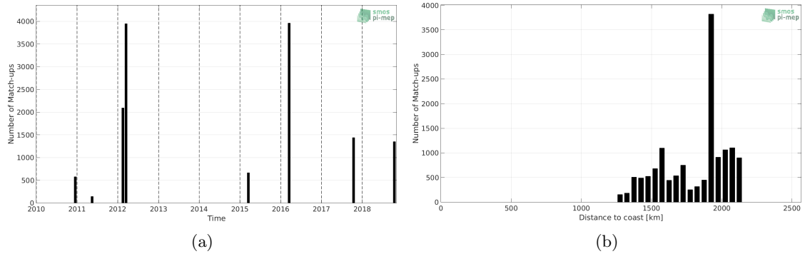
Figure 1: Number of match-ups between TSG (SAMOS) and SMOS SSS L2 v662 (ESA) SSS as a function of time (a) and as function of the distance to coast (b) over the SPURS 2 Pi-MEP region and for the full satellite product period.
