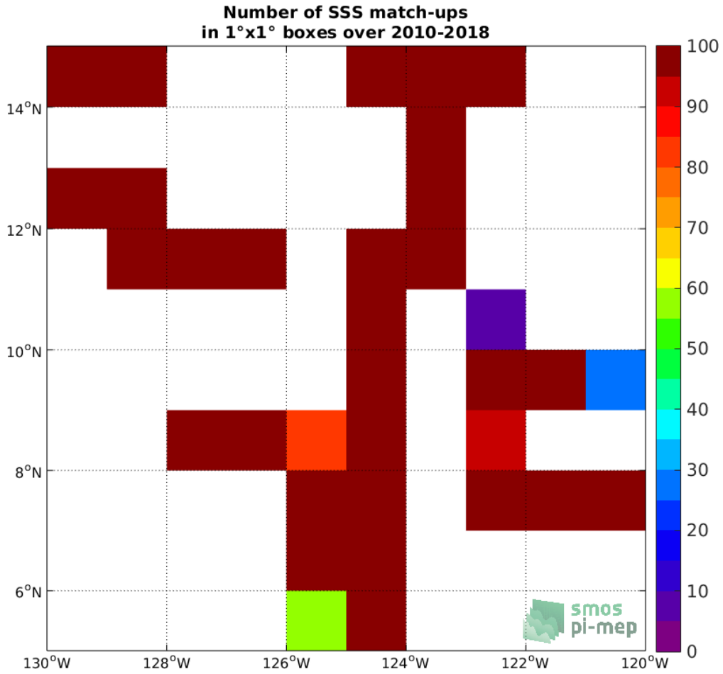
Figure 4: Number of SSS match-ups between TSG (SAMOS) SSS and the SMOS SSS L2 v662 (ESA) SSS product for the SPURS 2 Pi-MEP region over 1°x1° boxes and for the full satellite product period.
