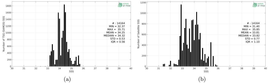
Figure 2: Histograms of SSS from TSG (SAMOS) (a) and SMOS SSS L2 v662 (ESA) (b) considering all match-up pairs per bins of 0.1 over the SPURS 2 Pi-MEP region and for the full satellite product period.
