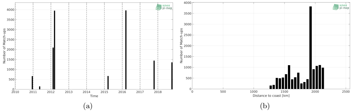
Figure 1: Number of match-ups between TSG-SAMOS and SMOS L2 v662 (ESA) SSS as a function of time (a) and as function of the distance to coast (b) over the SPURS 2 Pi-MEP region and for the full satellite product period.
