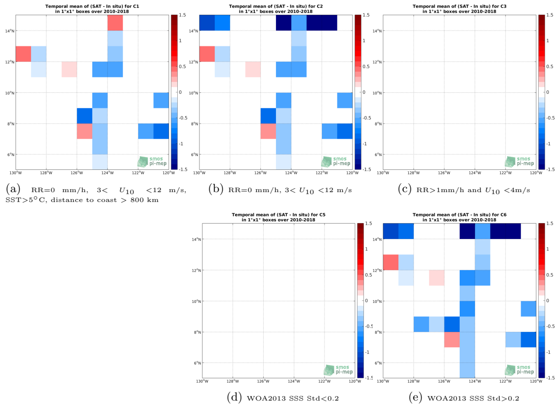
Figure 12: Temporal mean gridded over spatial boxes of size 1^\circ \times 1^\circ of \Delta SSS (SMOS L2 v662 (ESA) - TSG-SAMOS) for 5 different subdatasets corresponding to:RR=0 mm/h, 3 < U_{10} < 12 m/s, SST >5^\circ\text{C} , distance to coast > 800 km (a), RR=0 mm/h, 3 < U_{10} < 12 m/s (b), RR >1 mm/h and U_{10} < 4 m/s (c), WOA2013 SSS Std <0.2 (d), WOA2013 SSS Std >0.2 (e).
