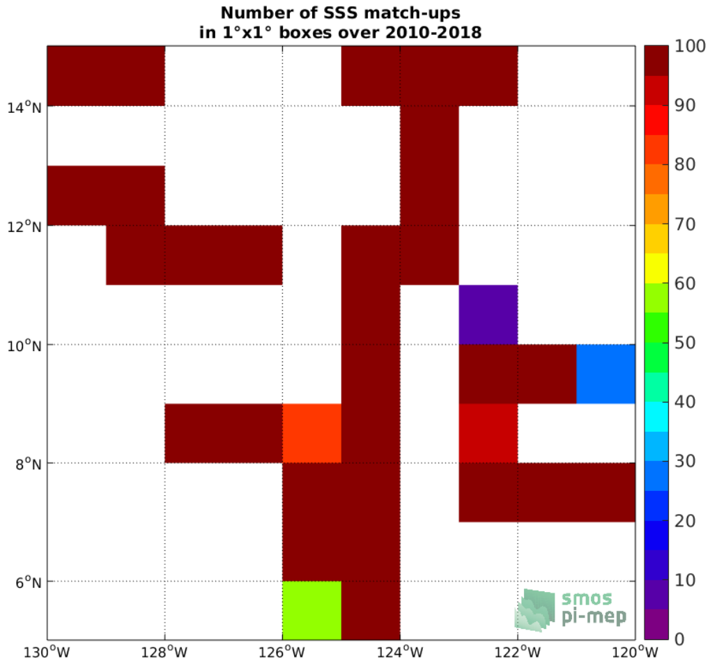
Figure 4: Number of SSS match-ups between TSG-SAMOS SSS and the SMOS L2 v662 (ESA) SSS product for the SPURS 2 Pi-MEP region over 1°x1° boxes and for the full satellite product period.
