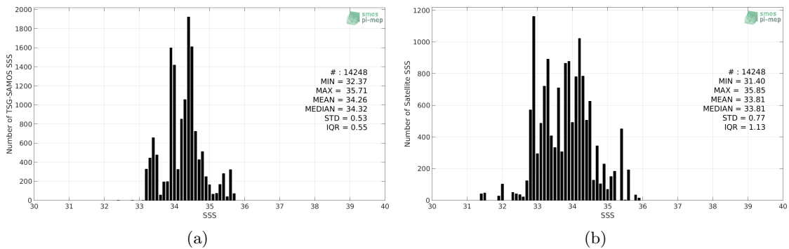
Figure 2: Histograms of SSS from TSG-SAMOS (a) and SMOS L2 v662 (ESA) (b) considering all match-up pairs per bins of 0.1 over the SPURS 2 Pi-MEP region and for the full satellite product period.
