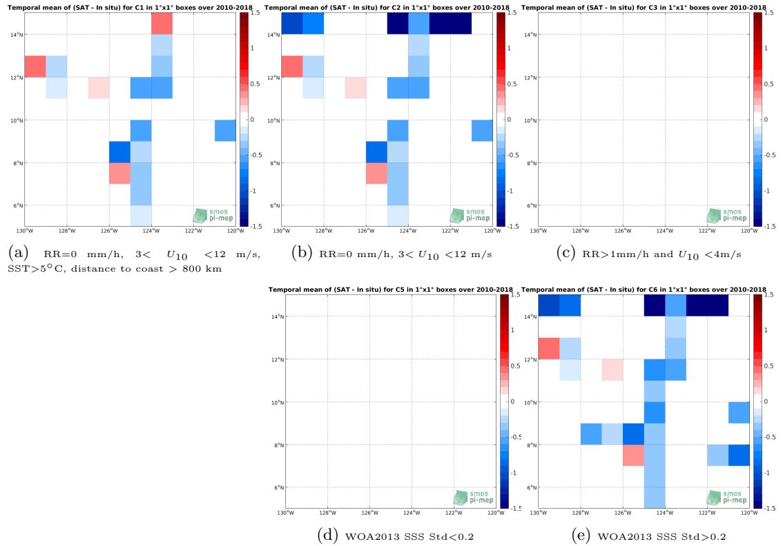
Figure 12: Temporal mean gridded over spatial boxes of size 1^\circ \times 1^\circ of \Delta SSS (SMOS-L2-DPGS-v662 - TSG-SAMOS) for 5 different subdatasets corresponding to: RR=0 mm/h, 3 < U_{10} < 12 m/s, SST > 5^\circ C , distance to coast > 800 km (a), RR=0 mm/h, 3 < U_{10} < 12 m/s (b), RR > 1 mm/h and U_{10} < 4 m/s (c), WOA2013 SSS Std < 0.2 (d), WOA2013 SSS Std > 0.2 (e).
