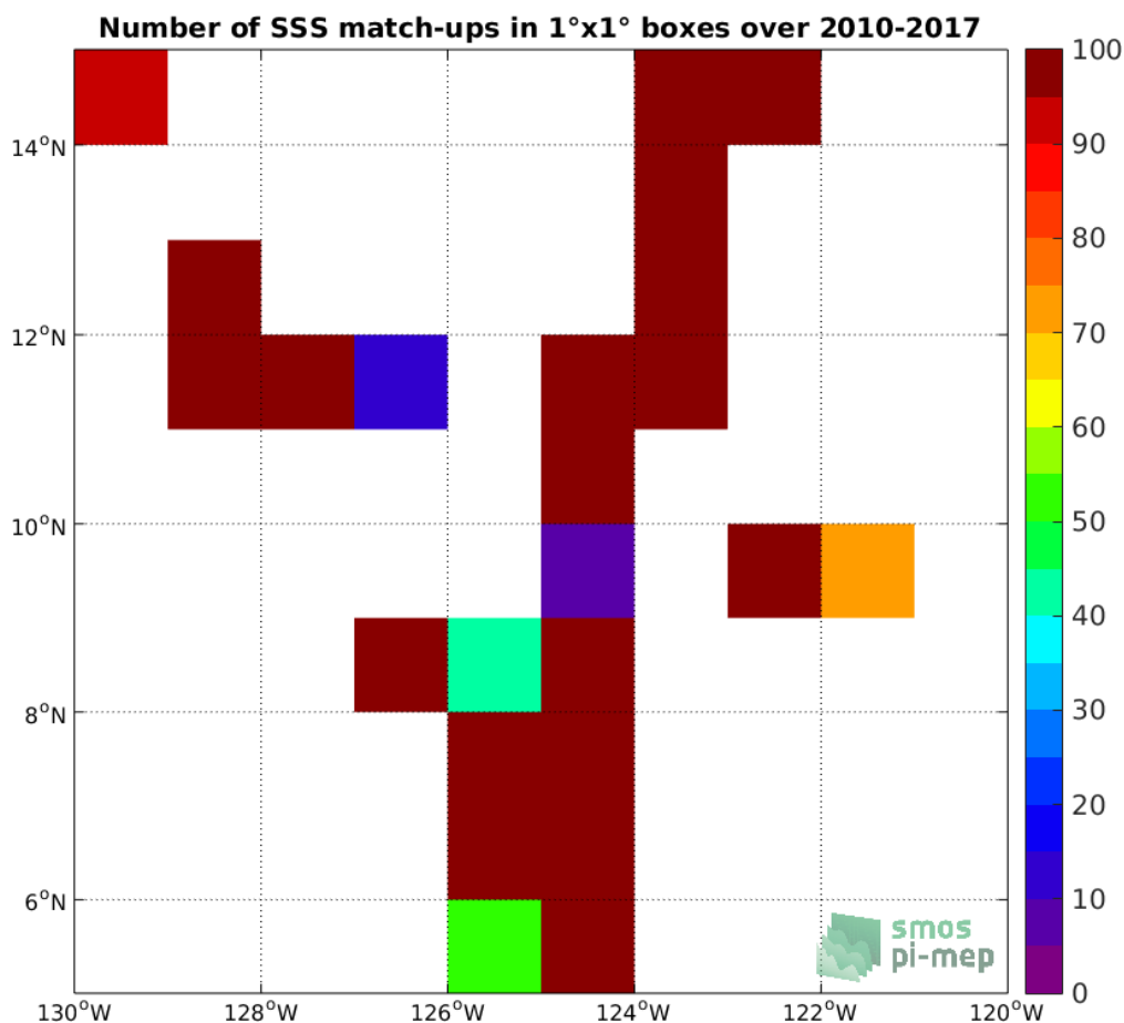
Figure 4: Number of SSS match-ups between TSG-SAMOS SSS and the SMOS-L2-DPGS-v662 SSS product for the SPURS 2 Pi-MEP region over 1°x1° boxes and for the full satellite product period.
