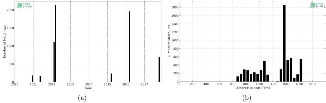
Figure 1: Number of match-ups between TSG-SAMOS and SMOS-L2-DPGS-v662 SSS as a function of time (a) and as function of the distance to coast (b) over the SPURS 2 Pi-MEP region and for the full satellite product period.
