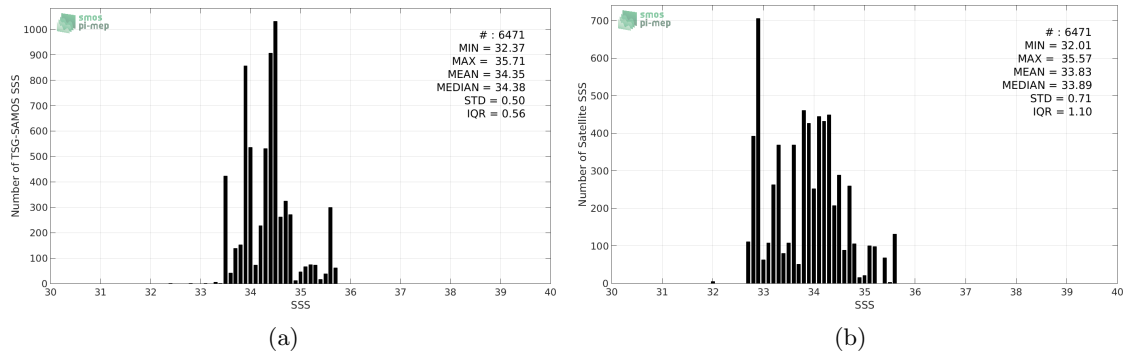
Figure 2: Histograms of SSS from TSG-SAMOS (a) and SMOS-L2-DPGS-v662 (b) considering all match-up pairs per bins of 0.1 over the SPURS 2 Pi-MEP region and for the full satellite product period.
