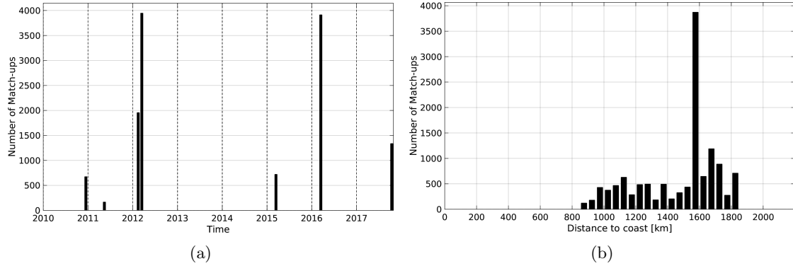
Figure 1: Number of match-ups between TSG-SAMOS and SMOS-L2-DPGS-v662 SSS as a function of time (a) and as function of the distance to coast (b) over the SPURS 2 Pi-MEP region and for the full satellite product period.
