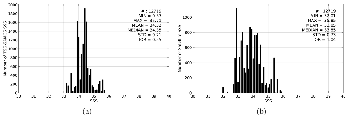
Figure 2: Histograms of SSS from TSG-SAMOS (a) and SMOS-L2-DPGS-v662 (b) considering all match-up pairs per bins of 0.1 over the SPURS 2 Pi-MEP region and for the full satellite product period.
