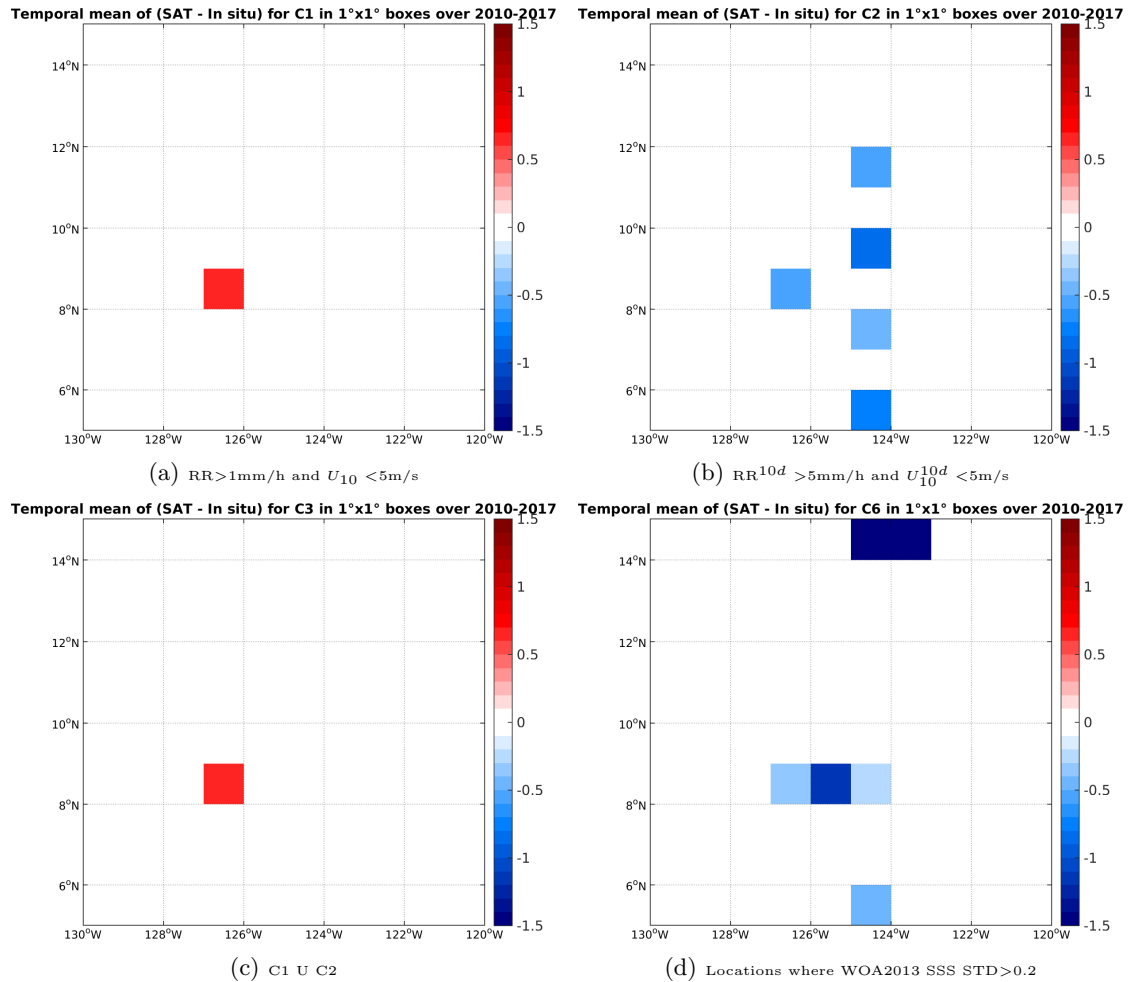
Figure 12: Temporal mean gridded over spatial boxes of size 1^\circ \times 1^\circ of \Delta SSS (SMOS-L2-DPGS-v662 - TSG-SAMOS) for 4 different subdatasets corresponding to: RR > 1\text{mm/h} and U_{10} < 5\text{m/s} (a), RR^{10d} > 5\text{mm/h} and U_{10}^{10d} < 5\text{m/s} (b), C1 U C2 (c), Locations where WOA2013 SSS STD > 0.2 (d).
