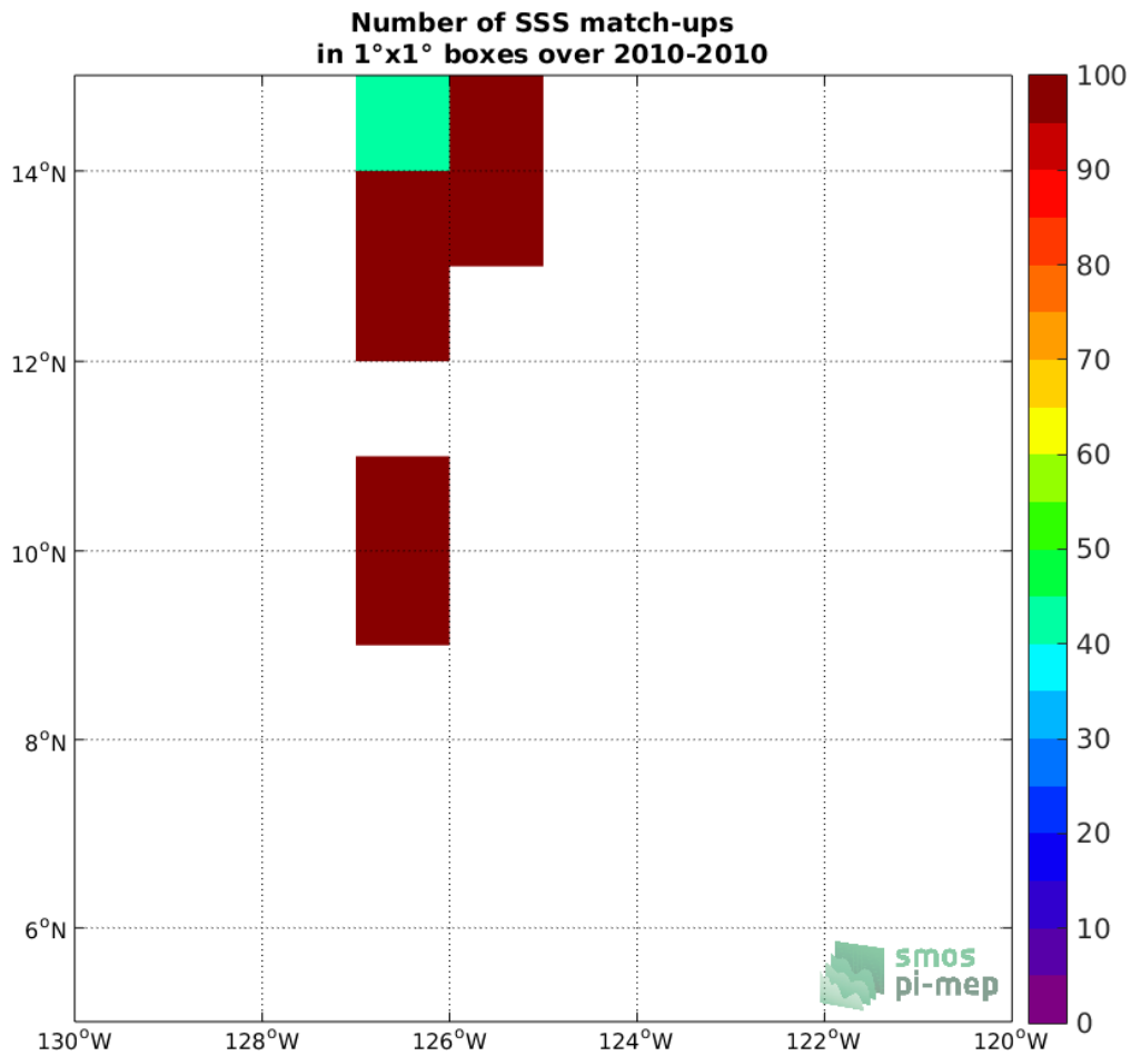
Figure 4: Number of SSS match-ups between TSG (GOSUD-Sailing-ship) SSS and the SMOS SSS L2 v662 (ESA) SSS product for the SPURS 2 Pi-MEP region over 1^\circ \times 1^\circ boxes and for the full satellite product period.
