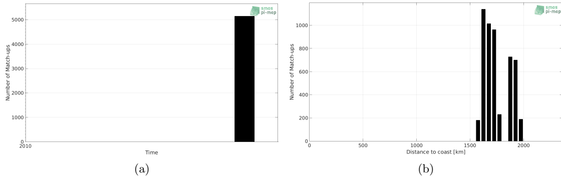
Figure 1: Number of match-ups between TSG (GOSUD-Sailing-ship) and SMOS SSS L2 v662 (ESA) SSS as a function of time (a) and as function of the distance to coast (b) over the SPURS 2 Pi-MEP region and for the full satellite product period.
