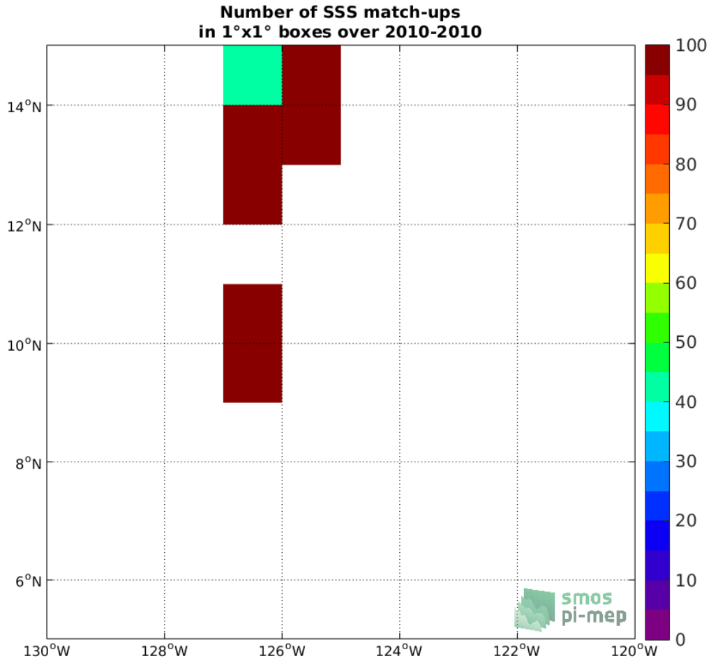
Figure 4: Number of SSS match-ups between TSG (GOSUD-Sailing-ship) SSS and the SMOS SSS L2 v662 (ESA) SSS product for the SPURS 2 Pi-MEP region over 1°x1° boxes and for the full satellite product period.
