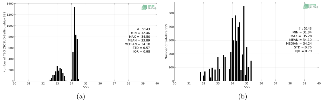
Figure 2: Histograms of SSS from TSG (GOSUD-Sailing-ship) (a) and SMOS SSS L2 v662 (ESA) (b) considering all match-up pairs per bins of 0.1 over the SPURS 2 Pi-MEP region and for the full satellite product period.
