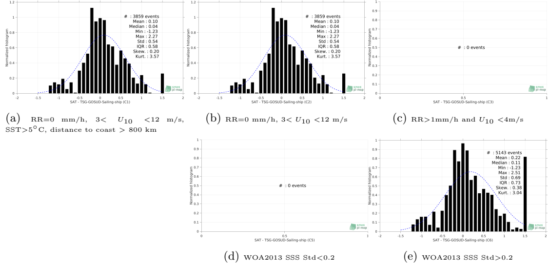
Figure 13: Normalized histogram of \Delta\text{SSS} (SMOS L2 v662 (ESA) - TSG-GOSUD-Sailing-ship) for 5 different subdatasets corresponding to: RR=0 mm/h, 3 < U_{10} < 12 m/s, SST > 5^{\circ}\text{C} , distance to coast > 800 km (a), RR=0 mm/h, 3 < U_{10} < 12 m/s (b), RR > 1\text{mm/h} and U_{10} < 4\text{m/s} (c), WOA2013 SSS Std < 0.2 (d), WOA2013 SSS Std > 0.2 (e).
