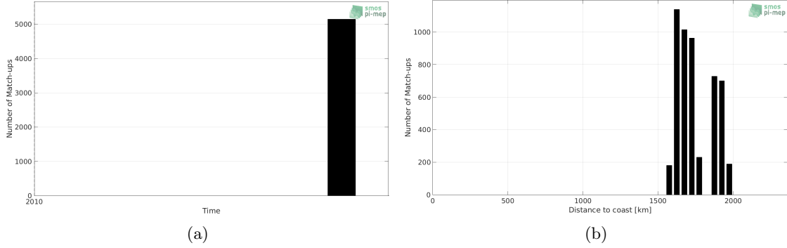
Figure 1: Number of match-ups between TSG-GOSUD-Sailing-ship and SMOS L2 v662 (ESA) SSS as a function of time (a) and as function of the distance to coast (b) over the SPURS 2 Pi-MEP region and for the full satellite product period.
