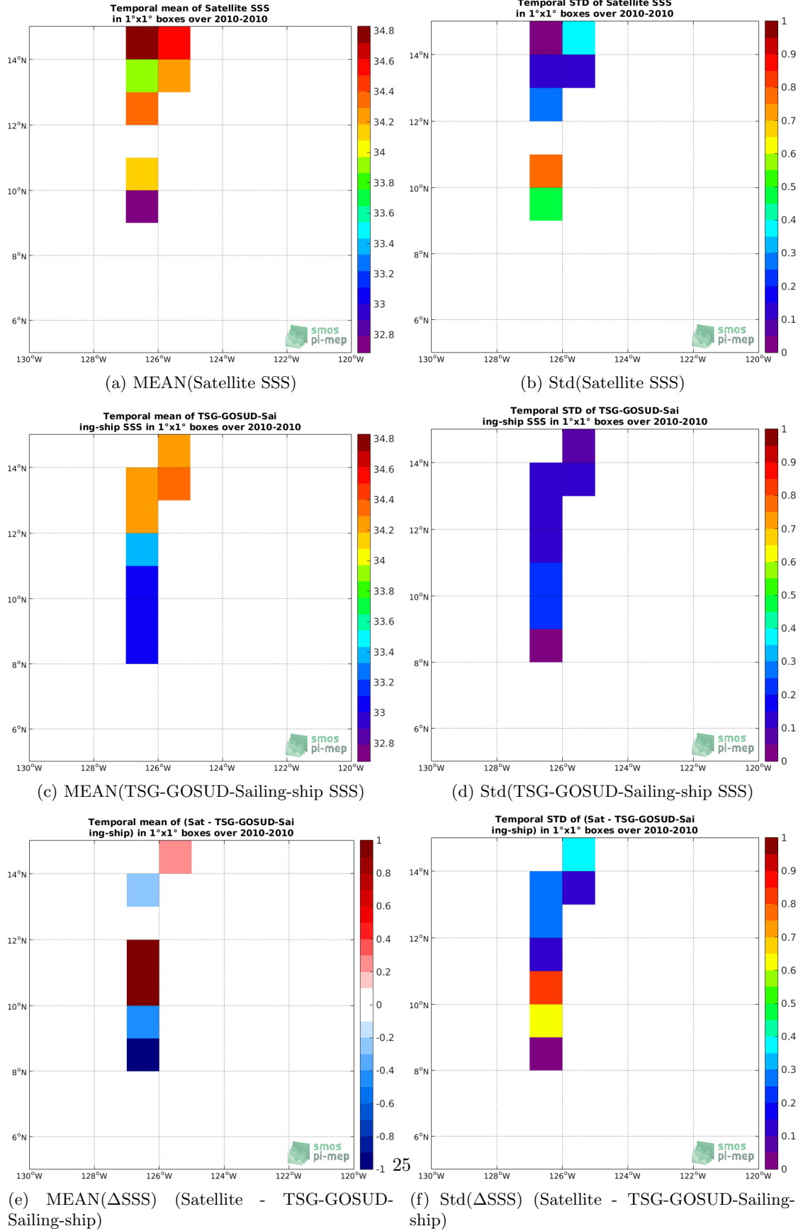
Figure 6: Temporal mean (left) and Std (right) of SSS from SMOS L2 v662 (ESA) (top), TSG-GOSUD-Sailing-ship (middle), and of \Delta SSS (Satellite - TSG-GOSUD-Sailing-ship). Only match-up pairs are used to generate these maps.
