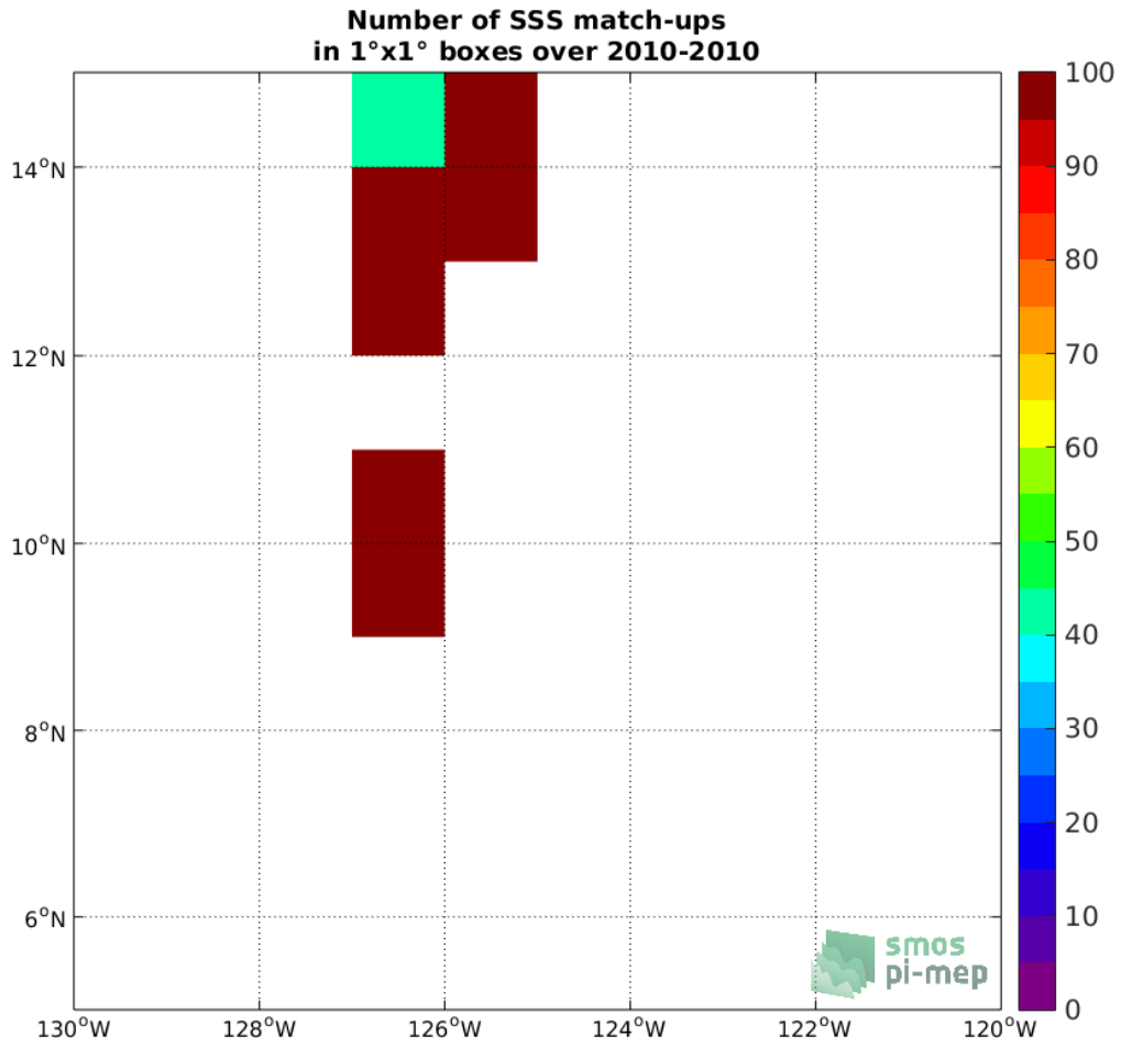
Figure 4: Number of SSS match-ups between TSG-GOSUD-Sailing-ship SSS and the SMOS L2 v662 (ESA) SSS product for the SPURS 2 Pi-MEP region over 1°x1° boxes and for the full satellite product period.
