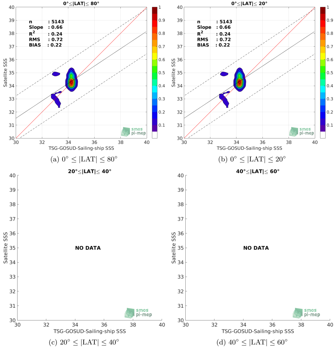
Figure 9: Contour maps of the concentration of SMOS L2 v662 (ESA) SSS (y-axis) versus TSG-GOSUD-Sailing-ship SSS (x-axis) at match-up pairs for different latitude bands. For each plot, the red line shows x=y . The black thin and dashed lines indicate a linear fit through the data cloud and the \pm 95\% confidence levels, respectively. The number match-up pairs n , the slope and R^2 coefficient of the linear fit, the root mean square (RMS) and the mean bias between satellite and in situ data are indicated for each latitude band in each plots.
