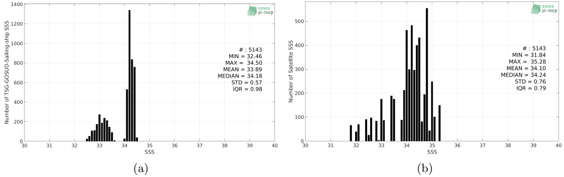
Figure 2: Histograms of SSS from TSG-GOSUD-Sailing-ship (a) and SMOS-L2-DPGS-v662 (b) considering all match-up pairs per bins of 0.1 over the SPURS 2 Pi-MEP region and for the full satellite product period.
