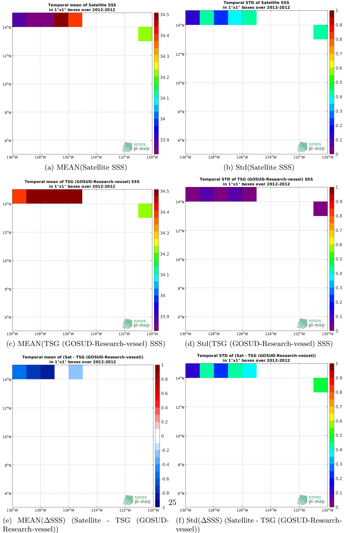
Figure 6: Temporal mean (left) and Std (right) of SSS from SMOS SSS L2 v662 (ESA) (top), TSG (GOSUD-Research-vessel) (middle), and of \Delta SSS (Satellite - TSG (GOSUD-Research-vessel)). Only match-up pairs are used to generate these maps.
