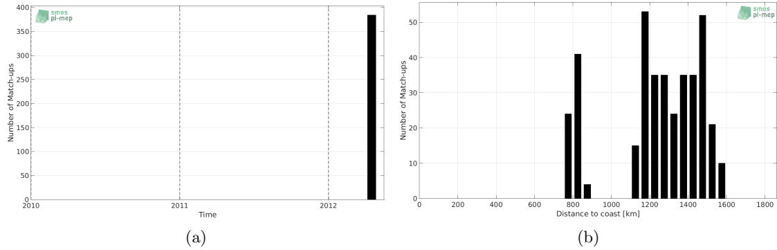
Figure 1: Number of match-ups between TSG-GOSUD-Research-vessel and SMOS-L2-DPGS-v662 SSS as a function of time (a) and as function of the distance to coast (b) over the SPURS 2 Pi-MEP region and for the full satellite product period.
