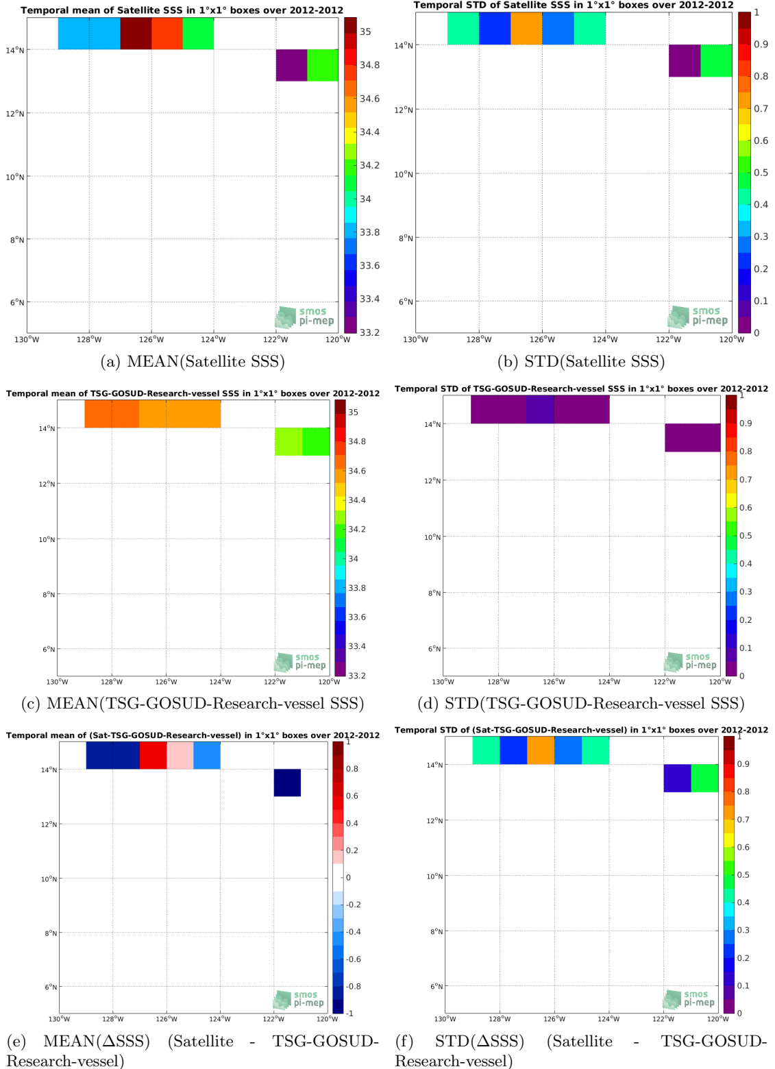
Figure 6: Temporal mean (left) and STD (right) of SSS from SMOS-L2-DPGS-v662 (top), TSG-GOSUD-Research-vessel (middle), and of \Delta SSS (Satellite - TSG-GOSUD-Research-vessel). Only match-up pairs are used to generate these maps!
