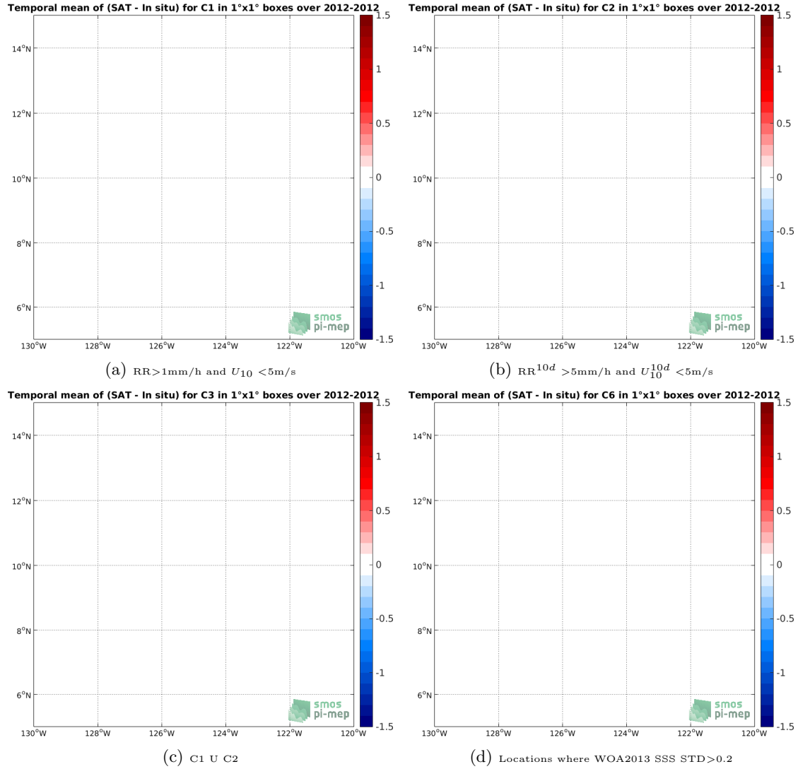
Figure 12: Temporal mean gridded over spatial boxes of size 1^\circ \times 1^\circ of \Delta SSS (SMOS-L2-DPGS-v662 - TSG-GOSUD-Research-vessel) for 4 different subdatasets corresponding to: RR > 1\text{mm/h} and U_{10} < 5\text{m/s} (a), RR^{10d} > 5\text{mm/h} and U_{10}^{10d} < 5\text{m/s} (b), C1 U C2 (c), Locations where WOA2013 SSS STD > 0.2 (d).
