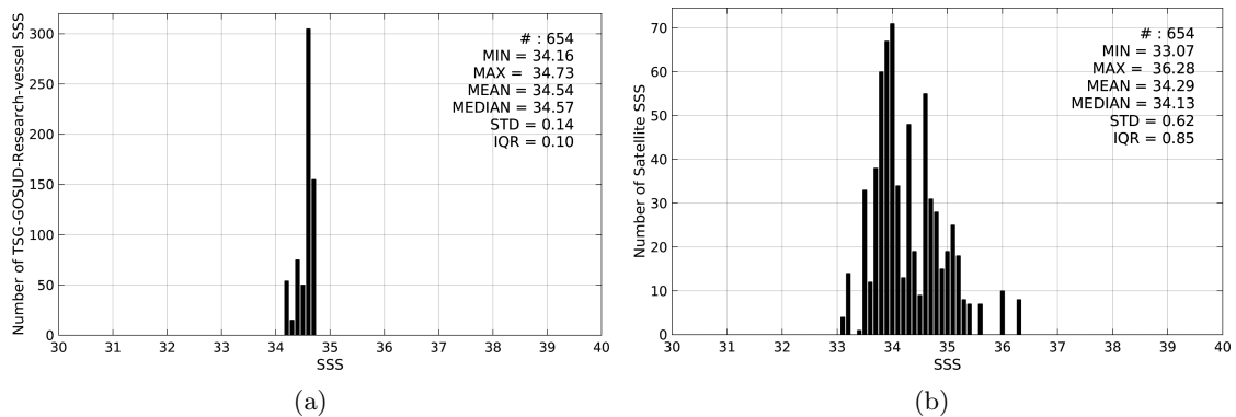
Figure 2: Histograms of SSS from TSG-GOSUD-Research-vessel (a) and SMOS-L2-DPGS-v662 (b) considering all match-up pairs per bins of 0.1 over the SPURS 2 Pi-MEP region and for the full satellite product period.
