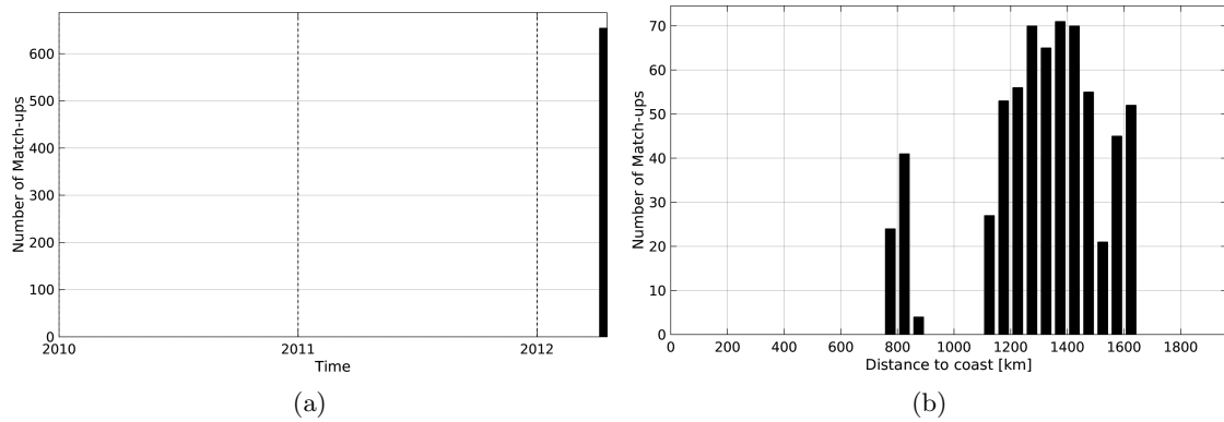
Figure 1: Number of match-ups between TSG-GOSUD-Research-vessel and SMOS-L2-DPGS-v662 SSS as a function of time (a) and as function of the distance to coast (b) over the SPURS 2 Pi-MEP region and for the full satellite product period.
