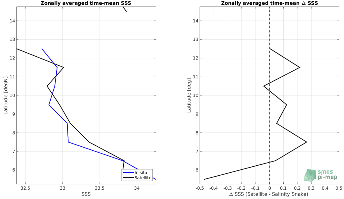
Figure 7: Left panel: Zonal mean SSS from SMOS SSS L2 v662 (ESA) satellite product (black) and from Salinity Snake (blue). Right panel: Zonal mean of \Delta SSS (Satellite - Salinity Snake) for all the collected Pi-MEP match-up pairs estimated over the full satellite product period.
