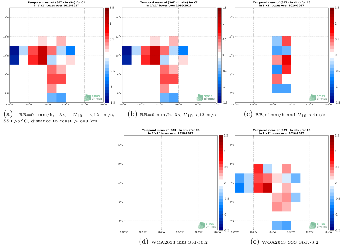
Figure 11: Temporal mean gridded over spatial boxes of size 1^\circ \times 1^\circ of \Delta SSS (SMOS SSS L2 v662 (ESA) - Salinity Snake) for 5 different subdatasets corresponding to: RR=0 mm/h, 3 < U_{10} < 12 m/s, SST > 5^\circ\text{C} , distance to coast > 800 km (a), RR=0 mm/h, 3 < U_{10} < 12 m/s (b), RR > 1 mm/h and U_{10} < 4 m/s (c), WOA2013 SSS Std < 0.2 (d), WOA2013 SSS Std > 0.2 (e).
