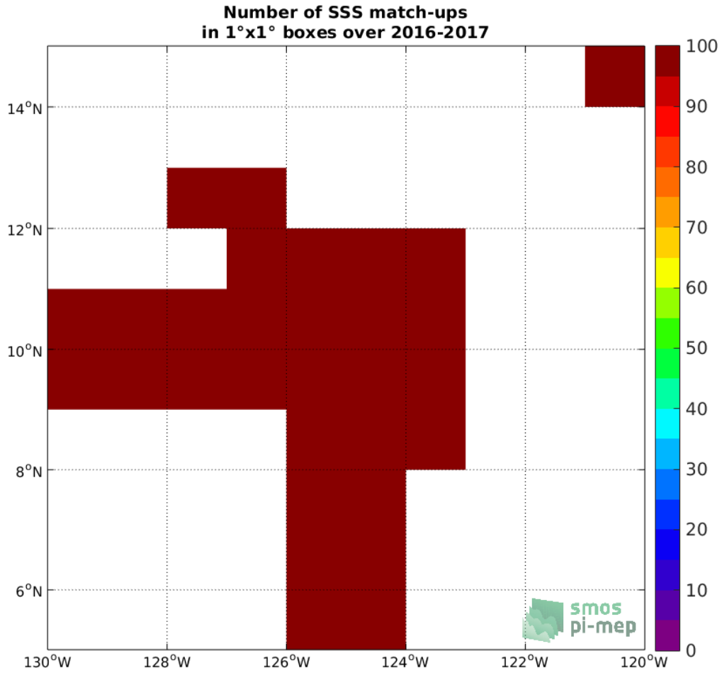
Figure 3: Number of SSS match-ups between Salinity Snake SSS and the SMOS SSS L2 v662 (ESA) SSS product for the SPURS 2 Pi-MEP region over 1°x1° boxes and for the full satellite product period.
