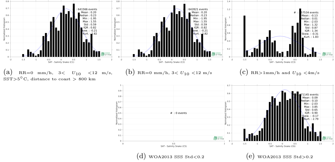
Figure 12: Normalized histogram of \Delta SSS (SMOS SSS L2 v662 (ESA) - Salinity Snake) for 5 different subdatasets corresponding to: RR=0 mm/h, 3 < U_{10} < 12 m/s, SST>5°C, distance to coast > 800 km (a), RR=0 mm/h, 3 < U_{10} < 12 m/s (b), RR>1mm/h and U_{10} < 4 m/s (c), WOA2013 SSS Std<0.2 (d), WOA2013 SSS Std>0.2 (e).
