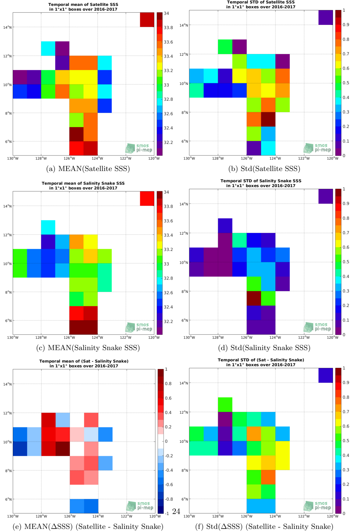
Figure 5: Temporal mean (left) and Std (right) of SSS from SMOS SSS L2 v662 (ESA) (top), Salinity Snake (middle), and of \Delta SSS (Satellite - Salinity Snake). Only match-up pairs are used to generate these maps.
