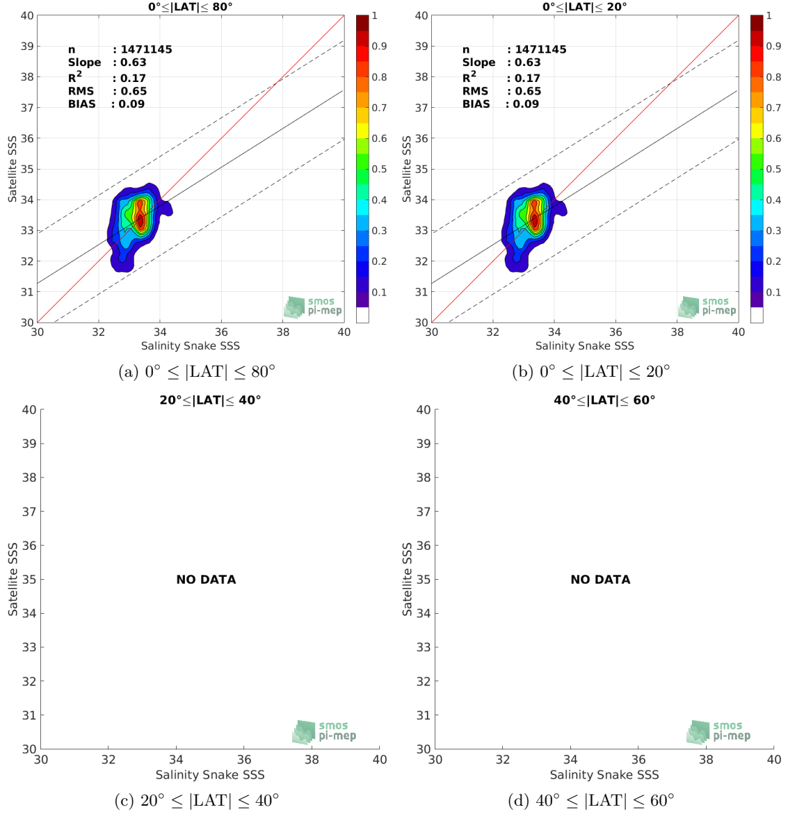
Figure 8: Contour maps of the concentration of SMOS SSS L2 v662 (ESA) SSS (y-axis) versus Salinity Snake SSS (x-axis) at match-up pairs for different latitude bands. For each plot, the red line shows x=y . The black thin and dashed lines indicate a linear fit through the data cloud and the \pm 95\% confidence levels, respectively. The number match-up pairs n , the slope and R^2 coefficient of the linear fit, the root mean square (RMS) and the mean bias between satellite and in situ data are indicated for each latitude band in each plots.
