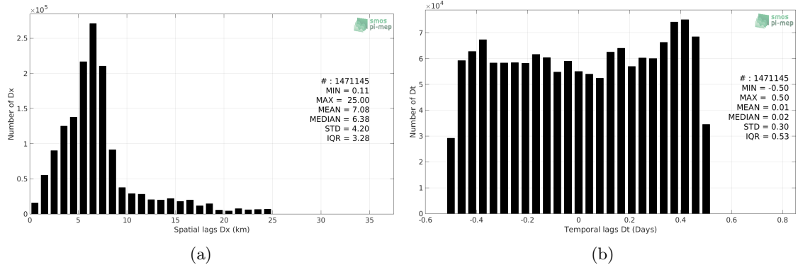
Figure 4: Histograms of the spatial (a) and temporal (b) lags between the location/time of the Salinity Snake measurement and the date of the corresponding SMOS SSS L2 v662 (ESA) SSS pixel.
