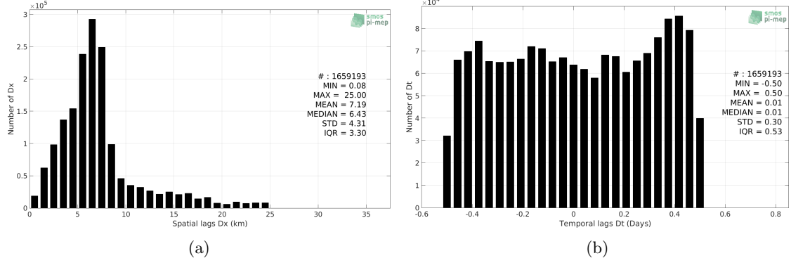
Figure 5: Histograms of the spatial (a) and temporal (b) lags between the time of the Salinity Snake measurements and the date of the corresponding SMOS SSS L2 v662 (ESA) SSS product.
