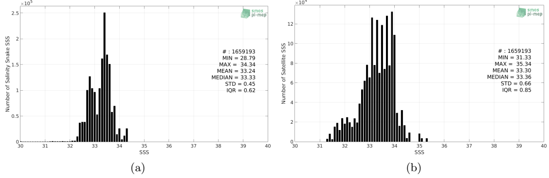
Figure 2: Histograms of SSS from Salinity Snake (a) and SMOS SSS L2 v662 (ESA) (b) considering all match-up pairs per bins of 0.1 over the SPURS 2 Pi-MEP region and for the full satellite product period.
