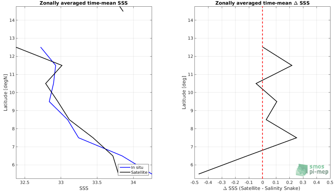
Figure 8: Left panel: Zonal mean SSS from SMOS SSS L2 v662 (ESA) satellite product (black) and from Salinity Snake (blue). Right panel: Zonal mean of \Delta SSS (Satellite - Salinity Snake) for all the collected Pi-MEP match-up pairs estimated over the full satellite product period.
