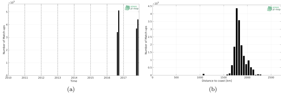
Figure 1: Number of match-ups between Salinity Snake and SMOS SSS L2 v662 (ESA) SSS as a function of time (a) and as function of the distance to coast (b) over the SPURS 2 Pi-MEP region and for the full satellite product period.
