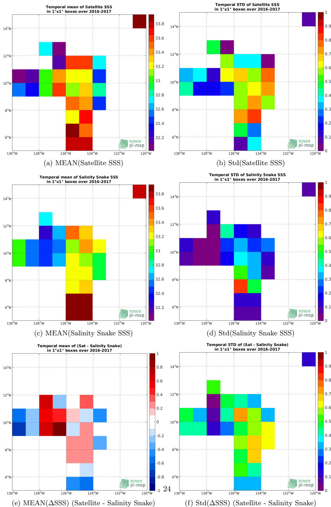
Figure 6: Temporal mean (left) and Std (right) of SSS from SMOS SSS L2 v662 (ESA) (top), Salinity Snake (middle), and of \Delta SSS (Satellite - Salinity Snake). Only match-up pairs are used to generate these maps.
