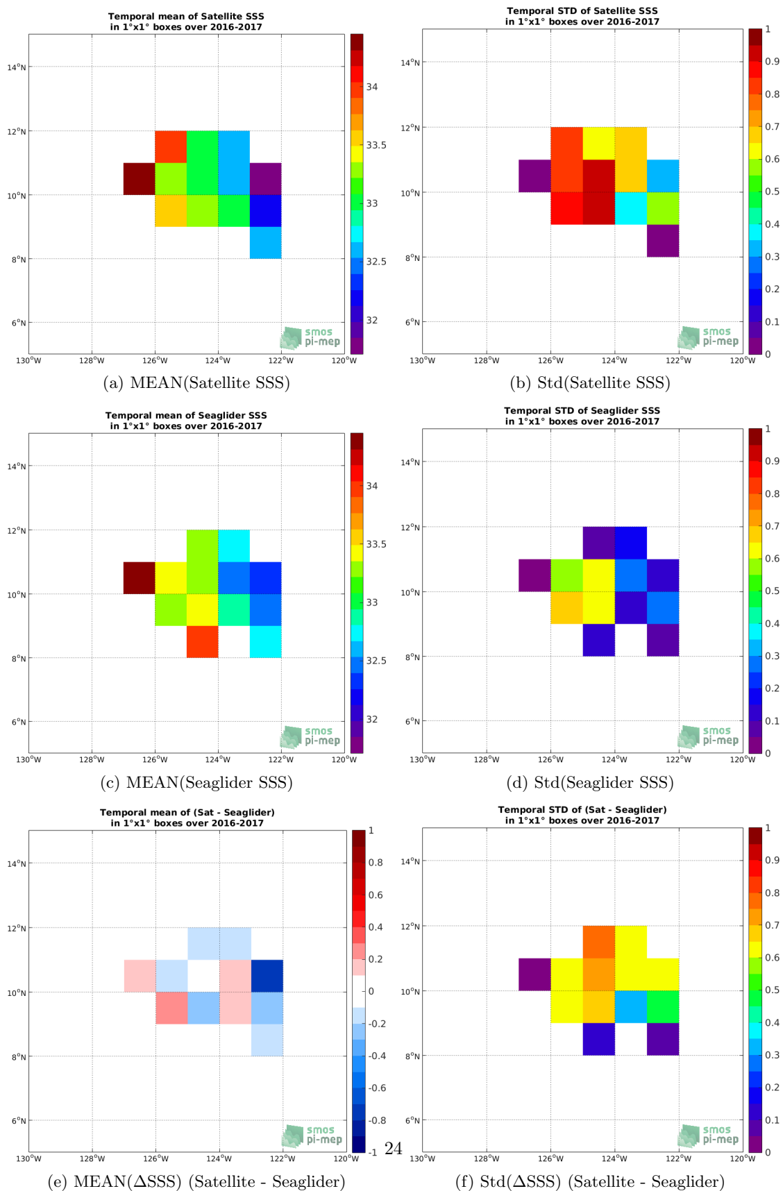
Figure 6: Temporal mean (left) and Std (right) of SSS from SMOS SSS L2 v662 (ESA) (top), Seaglider (middle), and of \Delta SSS (Satellite - Seaglider). Only match-up pairs are used to generate these maps.
