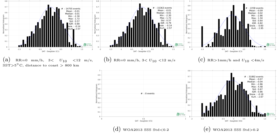
Figure 13: Normalized histogram of \Delta SSS (SMOS SSS L2 v662 (ESA) - Seaglider) for 5 different subdatasets corresponding to: RR=0 mm/h, 3 < U_{10} < 12 m/s, SST>5°C, distance to coast > 800 km (a), RR=0 mm/h, 3 < U_{10} < 12 m/s (b), RR>1mm/h and U_{10} < 4 m/s (c), WOA2013 SSS Std<0.2 (d), WOA2013 SSS Std>0.2 (e).
