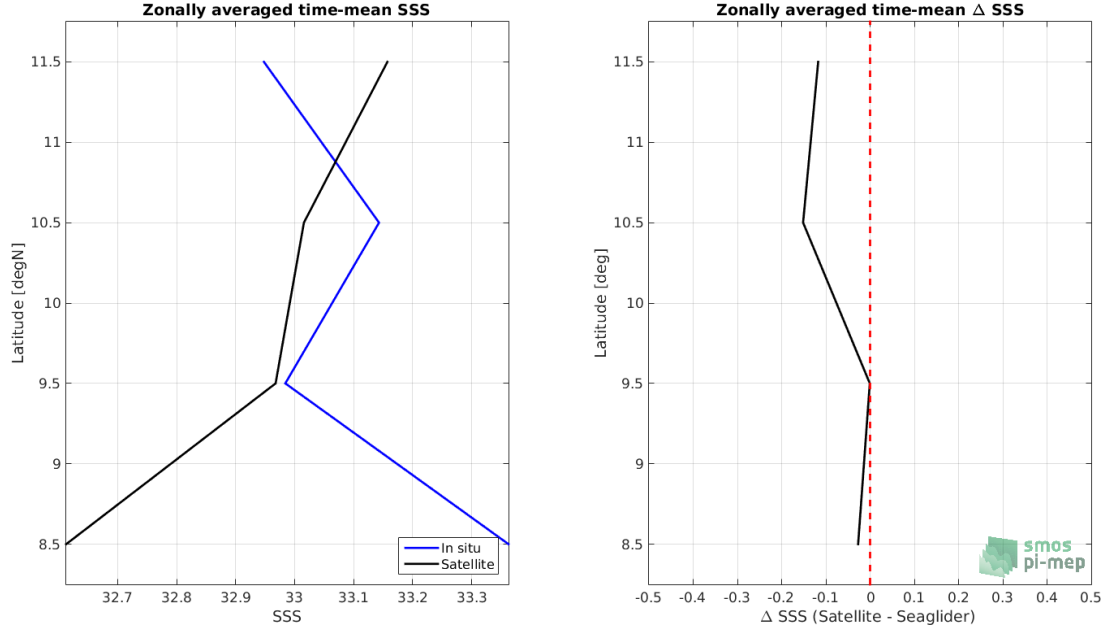
Figure 8: Left panel: Zonal mean SSS from SMOS SSS L2 v662 (ESA) satellite product (black) and from Seaglider (blue). Right panel: Zonal mean of \Delta SSS (Satellite - Seaglider) for all the collected Pi-MEP match-up pairs estimated over the full satellite product period.
