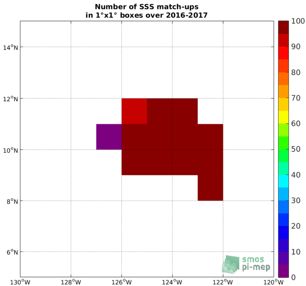
Figure 4: Number of SSS match-ups between Seaglider SSS and the SMOS SSS L2 v662 (ESA) SSS product for the SPURS 2 Pi-MEP region over 1°x1° boxes and for the full satellite product period.
