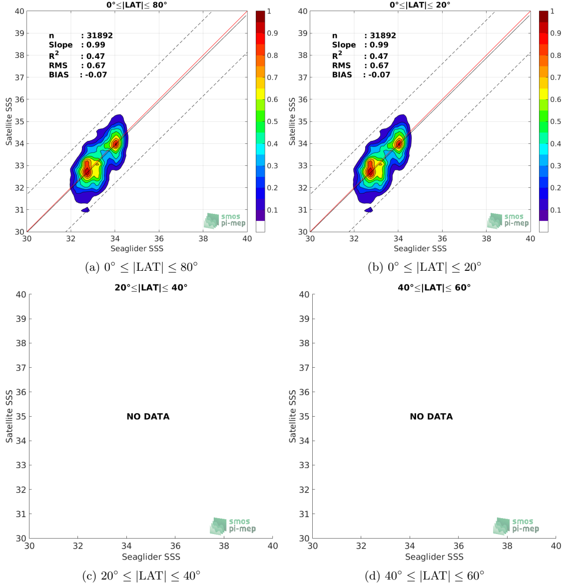
Figure 9: Contour maps of the concentration of SMOS SSS L2 v662 (ESA) SSS (y-axis) versus Seaglider SSS (x-axis) at match-up pairs for different latitude bands. For each plot, the red line shows x=y . The black thin and dashed lines indicate a linear fit through the data cloud and the \pm 95\% confidence levels, respectively. The number match-up pairs n , the slope and R^2 coefficient of the linear fit, the root mean square (RMS) and the mean bias between satellite and in situ data are indicated for each latitude band in each plots.
