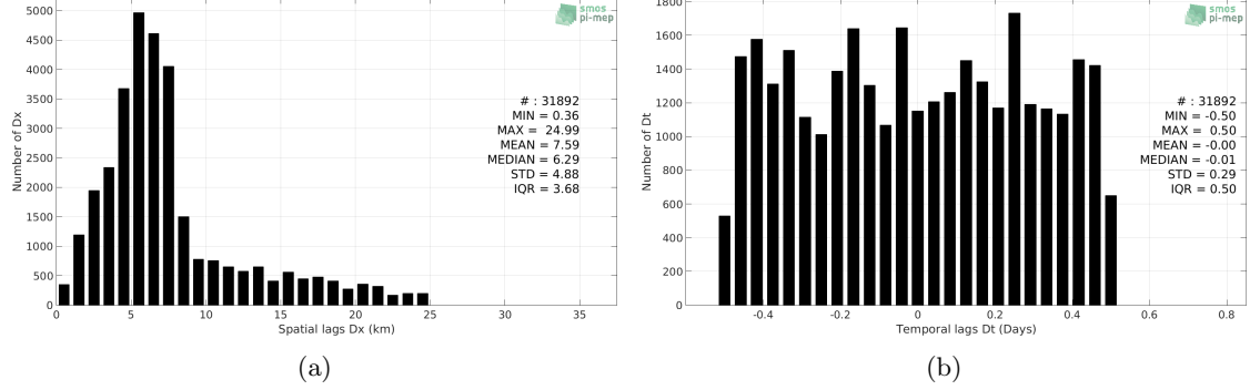
Figure 5: Histograms of the spatial (a) and temporal (b) lags between the time of the Seaglider measurements and the date of the corresponding SMOS SSS L2 v662 (ESA) SSS product.
