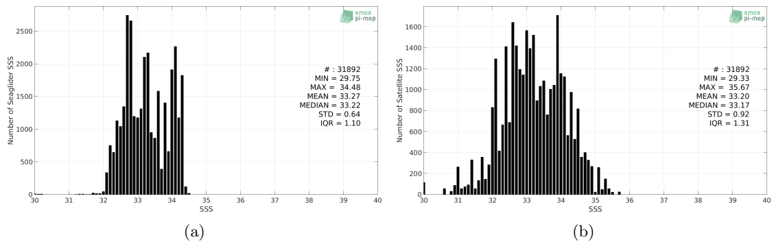
Figure 2: Histograms of SSS from Seaglider (a) and SMOS SSS L2 v662 (ESA) (b) considering all match-up pairs per bins of 0.1 over the SPURS 2 Pi-MEP region and for the full satellite product period.
