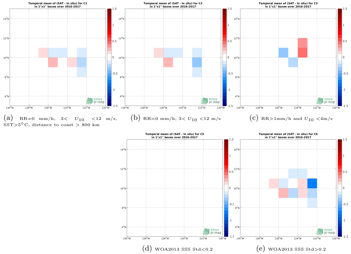
Figure 12: Temporal mean gridded over spatial boxes of size 1^\circ \times 1^\circ of \Delta SSS (SMOS SSS L2 v662 (ESA) - Seaglider) for 5 different subdatasets corresponding to: RR=0 mm/h, 3 < U_{10} < 12 m/s, SST >5^\circ\text{C} , distance to coast > 800 km (a), RR=0 mm/h, 3 < U_{10} < 12 m/s (b), RR >1 mm/h and U_{10} < 4 m/s (c), WOA2013 SSS Std <0.2 (d), WOA2013 SSS Std >0.2 (e).
