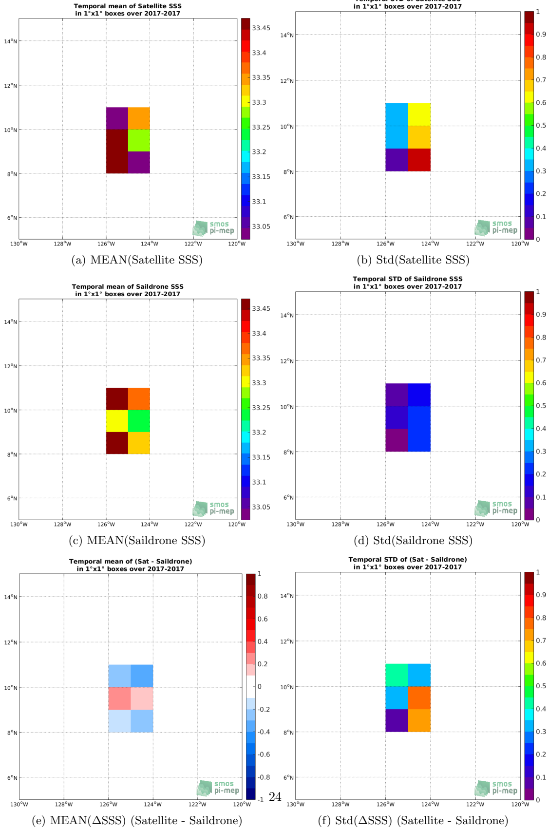
Figure 5: Temporal mean (left) and Std (right) of SSS from SMOS SSS L2 v662 (ESA) (top), Saildrone (middle), and of \Delta SSS (Satellite - Saildrone). Only match-up pairs are used to generate these maps.
