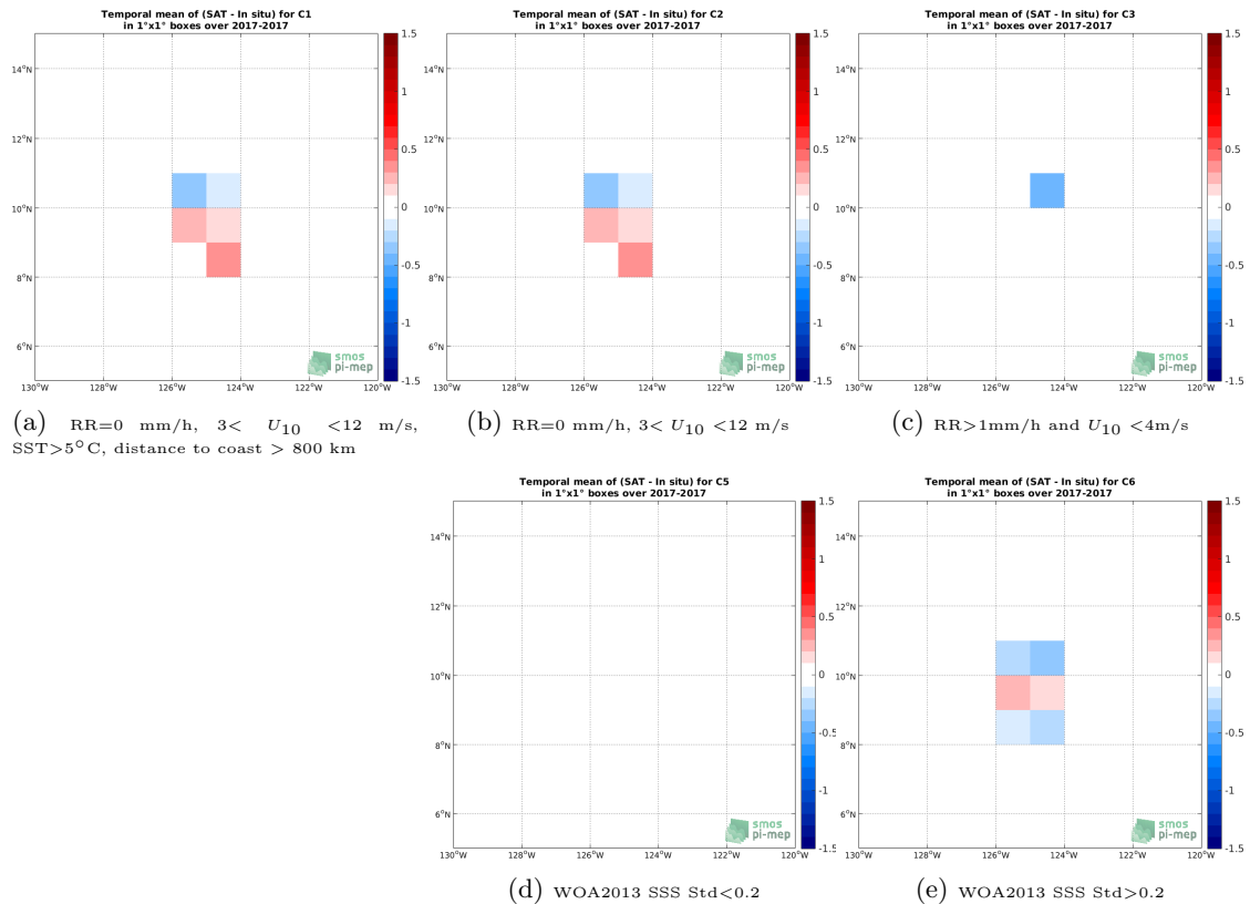
Figure 11: Temporal mean gridded over spatial boxes of size 1^\circ \times 1^\circ of \Delta SSS (SMOS SSS L2 v662 (ESA) - Saildrone) for 5 different subdatasets corresponding to: RR=0 mm/h, 3 < U_{10} < 12 m/s, SST > 5^\circ C , distance to coast > 800 km (a), RR=0 mm/h, 3 < U_{10} < 12 m/s (b), RR > 1 mm/h and U_{10} < 4 m/s (c), WOA2013 SSS Std < 0.2 (d), WOA2013 SSS Std > 0.2 (e).
