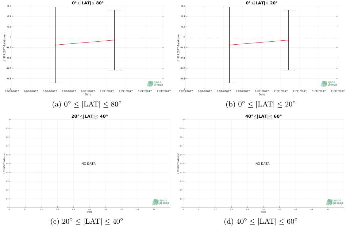
Figure 9: Monthly median (red curves) of \Delta\text{SSS} (Satellite - Sailability) and \pm 1 Std (black vertical thick bars) as function of time for all the collected Pi-MEP match-up pairs estimated over the SPURS 2 Pi-MEP region and for the full satellite product period are shown for different latitude bands: (a) 80°S-80°N, (b) 20°S-20°N, (c) 40°S-20°S and 20°N-40°N and (d) 60°S-40°S and 40°N-60°N.
