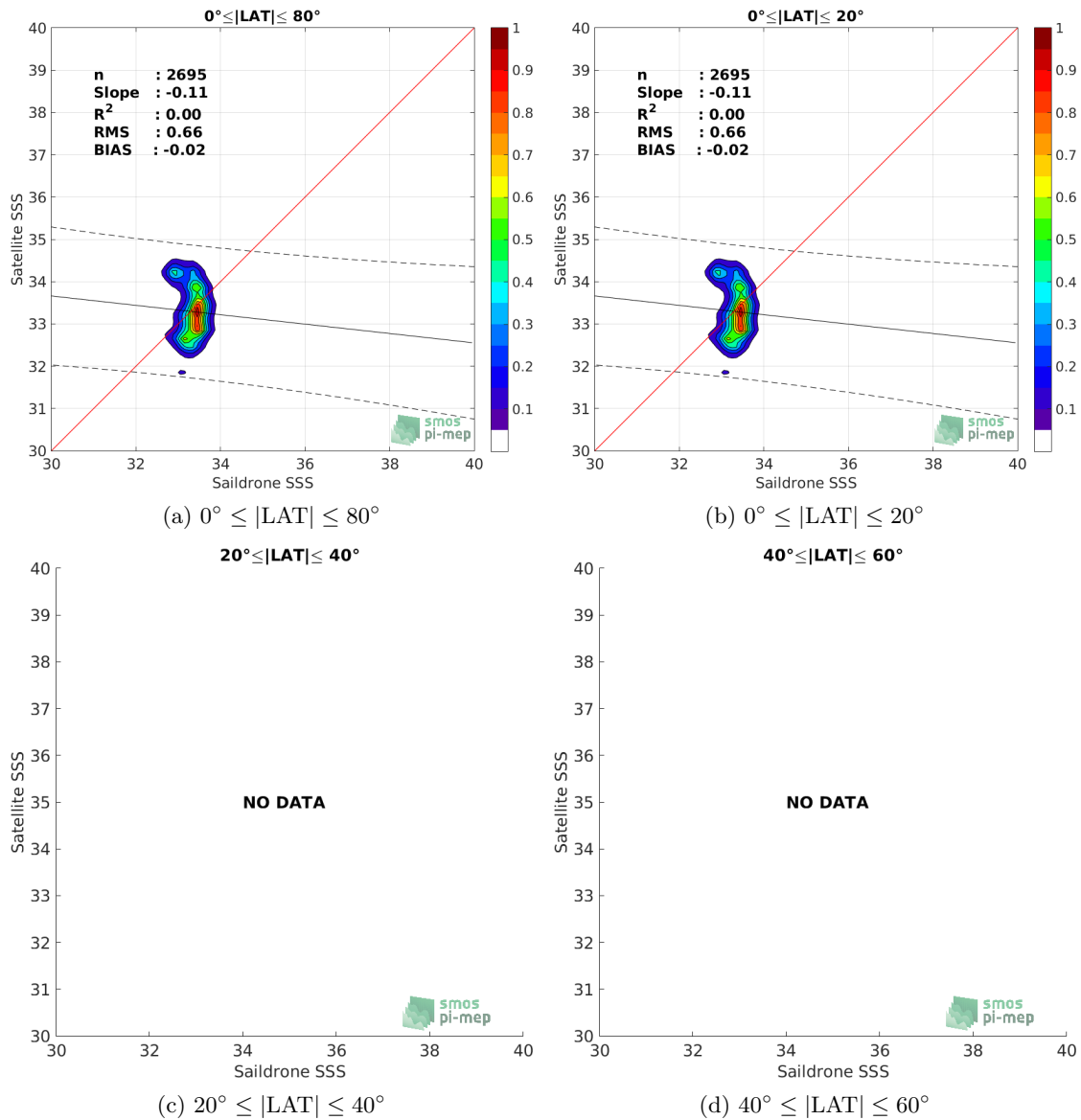
Figure 8: Contour maps of the concentration of SMOS SSS L2 v662 (ESA) SSS (y-axis) versus Saildrone SSS (x-axis) at match-up pairs for different latitude bands. For each plot, the red line shows x=y . The black thin and dashed lines indicate a linear fit through the data cloud and the \pm 95\% confidence levels, respectively. The number match-up pairs n , the slope and R^2 coefficient of the linear fit, the root mean square (RMS) and the mean bias between satellite and in situ data are indicated for each latitude band in each plots.
