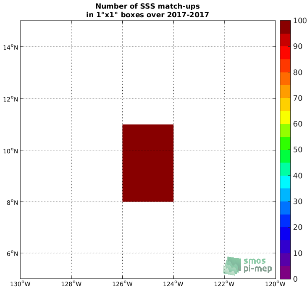
Figure 3: Number of SSS match-ups between Sairdrone SSS and the SMOS SSS L2 v662 (ESA) SSS product for the SPURS 2 Pi-MEP region over 1°x1° boxes and for the full satellite product period.
