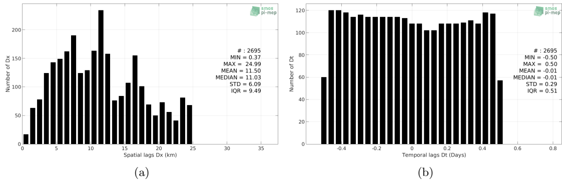
Figure 4: Histograms of the spatial (a) and temporal (b) lags between the location/time of the Saildrone measurement and the date of the corresponding SMOS SSS L2 v662 (ESA) SSS pixel.
