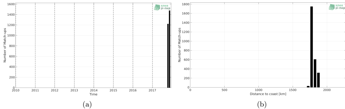
Figure 1: Number of match-ups between Saildrone and SMOS SSS L2 v662 (ESA) SSS as a function of time (a) and as function of the distance to coast (b) over the SPURS 2 Pi-MEP region and for the full satellite product period.
