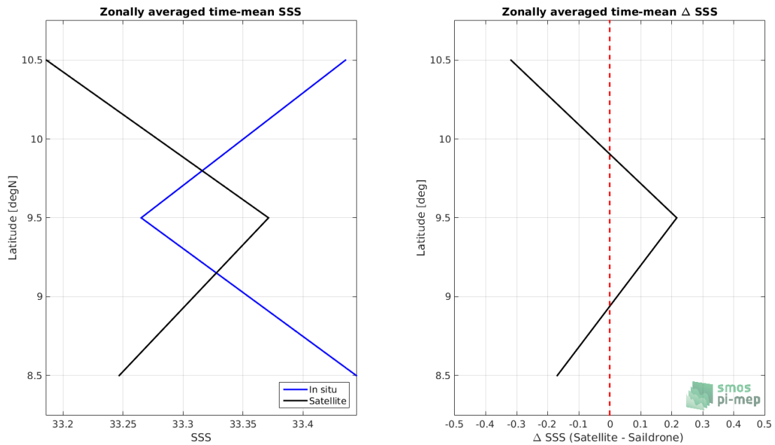
Figure 7: Left panel: Zonal mean SSS from SMOS SSS L2 v662 (ESA) satellite product (black) and from Sairdrone (blue). Right panel: Zonal mean of \Delta SSS (Satellite - Sairdrone) for all the collected Pi-MEP match-up pairs estimated over the full satellite product period.
