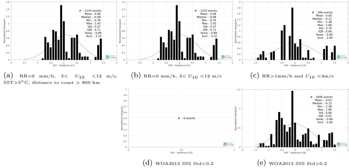
Figure 12: Normalized histogram of \Delta SSS (SMOS SSS L2 v662 (ESA) - Saildrone) for 5 different subdatasets corresponding to: RR=0 mm/h, 3 < U_{10} < 12 m/s, SST > 5°C, distance to coast > 800 km (a), RR=0 mm/h, 3 < U_{10} < 12 m/s (b), RR > 1mm/h and U_{10} < 4 m/s (c), WOA2013 SSS Std < 0.2 (d), WOA2013 SSS Std > 0.2 (e).
