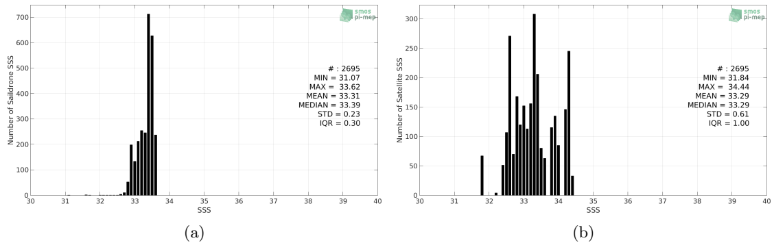
Figure 2: Histograms of SSS from Saildrone (a) and SMOS SSS L2 v662 (ESA) (b) considering all match-up pairs per bins of 0.1 over the SPURS 2 Pi-MEP region and for the full satellite product period.
