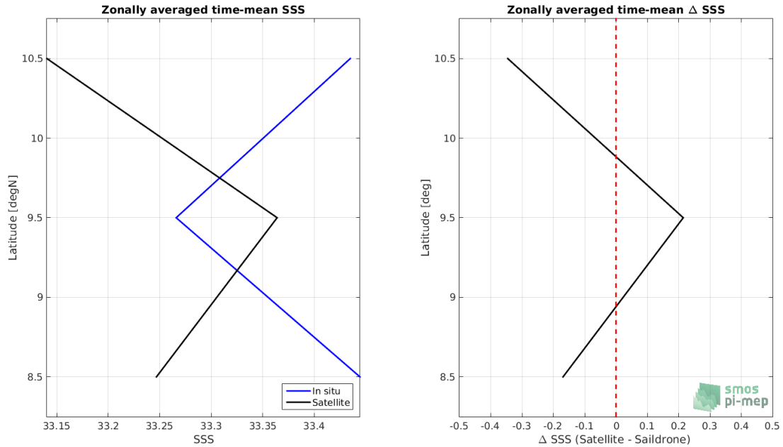
Figure 8: Left panel: Zonal mean SSS from SMOS SSS L2 v662 (ESA) satellite product (black) and from Saildrone (blue). Right panel: Zonal mean of \Delta SSS (Satellite - Saildrone) for all the collected Pi-MEP match-up pairs estimated over the full satellite product period.
