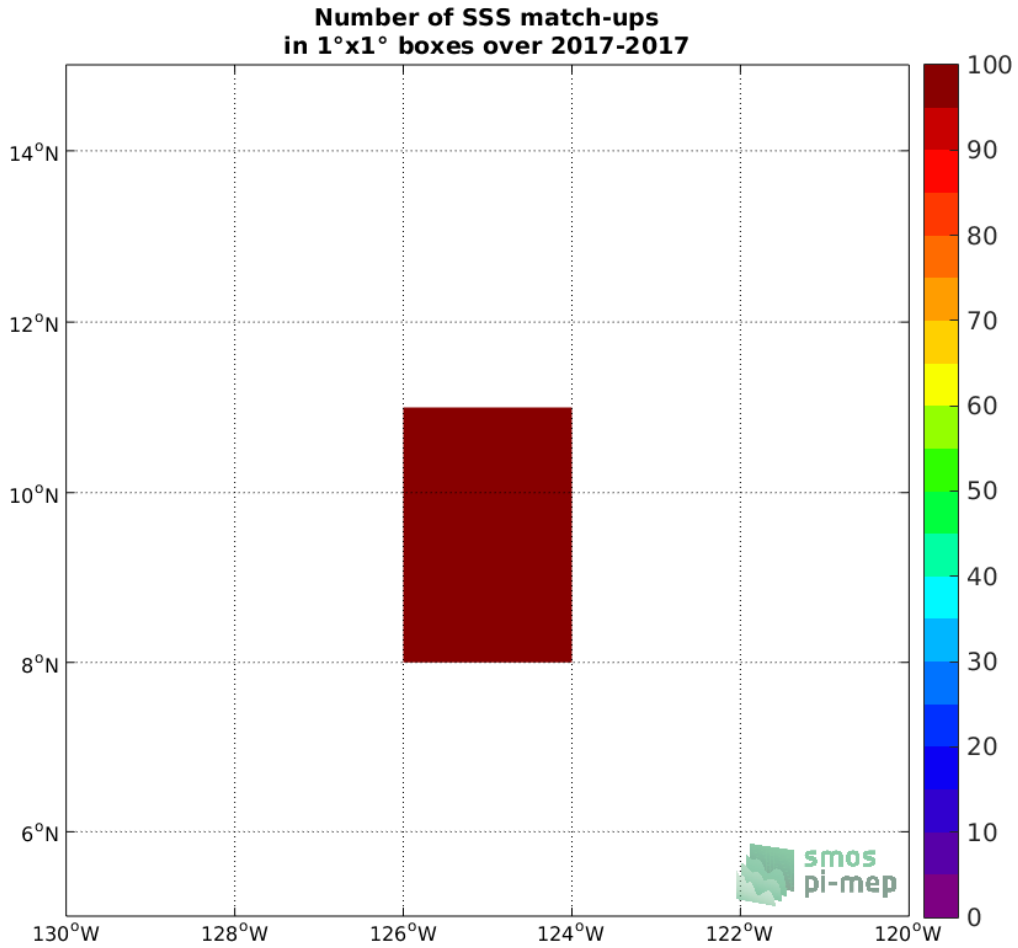
Figure 4: Number of SSS match-ups between Sairdrone SSS and the SMOS SSS L2 v662 (ESA) SSS product for the SPURS 2 Pi-MEP region over 1°x1° boxes and for the full satellite product period.
