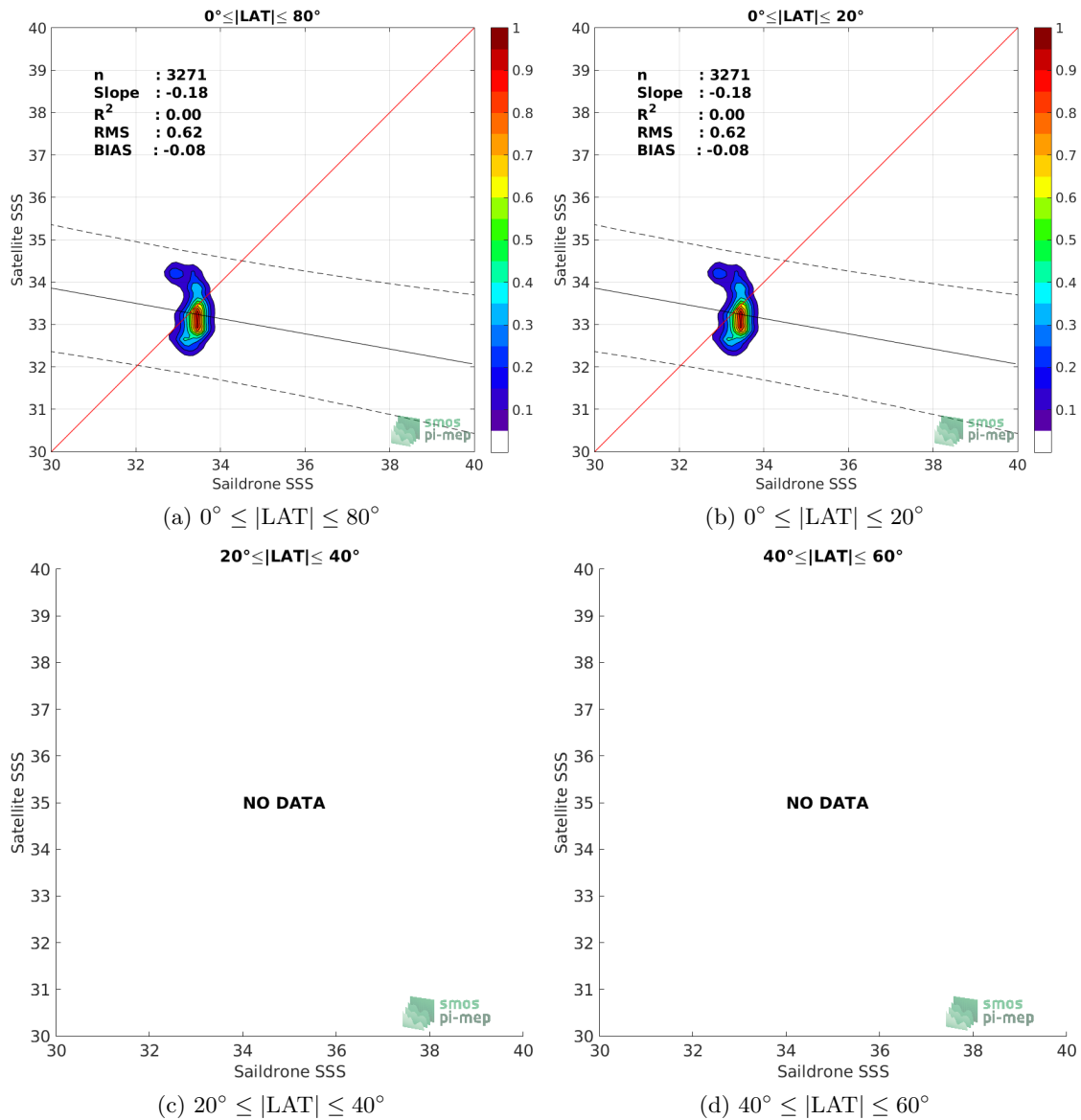
Figure 9: Contour maps of the concentration of SMOS SSS L2 v662 (ESA) SSS (y-axis) versus Saildrone SSS (x-axis) at match-up pairs for different latitude bands. For each plot, the red line shows x=y . The black thin and dashed lines indicate a linear fit through the data cloud and the \pm 95\% confidence levels, respectively. The number match-up pairs n , the slope and R^2 coefficient of the linear fit, the root mean square (RMS) and the mean bias between satellite and in situ data are indicated for each latitude band in each plots.
