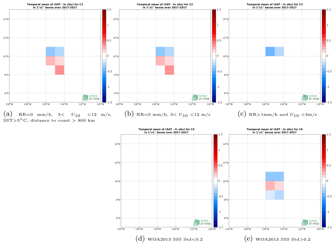
Figure 12: Temporal mean gridded over spatial boxes of size 1^\circ \times 1^\circ of \Delta SSS (SMOS SSS L2 v662 (ESA) - Sairdrone) for 5 different subdatasets corresponding to:RR=0 mm/h, 3 < U_{10} < 12 m/s, SST >5^\circ C, distance to coast > 800 km (a), RR=0 mm/h, 3 < U_{10} < 12 m/s (b), RR >1 mm/h and U_{10} < 4 m/s (c), WOA2013 SSS Std <0.2 (d), WOA2013 SSS Std >0.2 (e).
