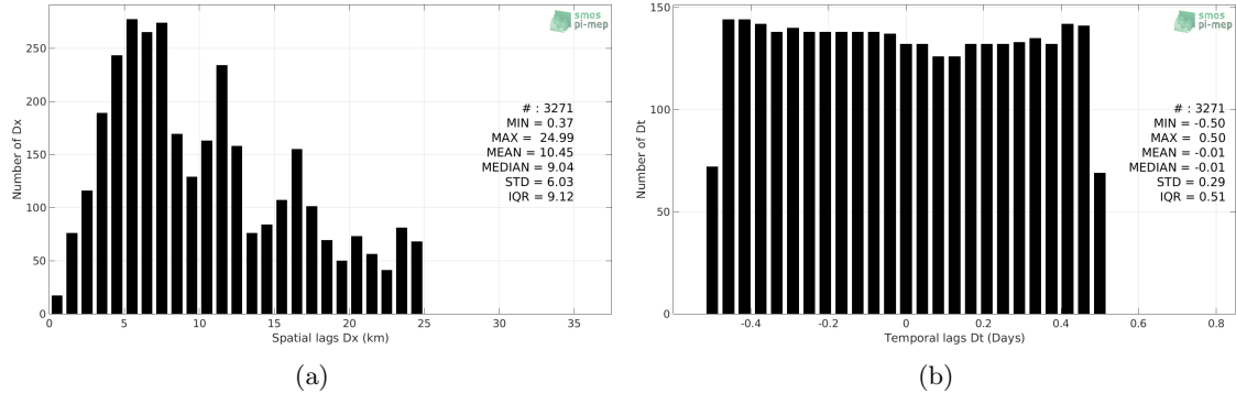
Figure 5: Histograms of the spatial (a) and temporal (b) lags between the time of the Saildrone measurements and the date of the corresponding SMOS SSS L2 v662 (ESA) SSS product.
