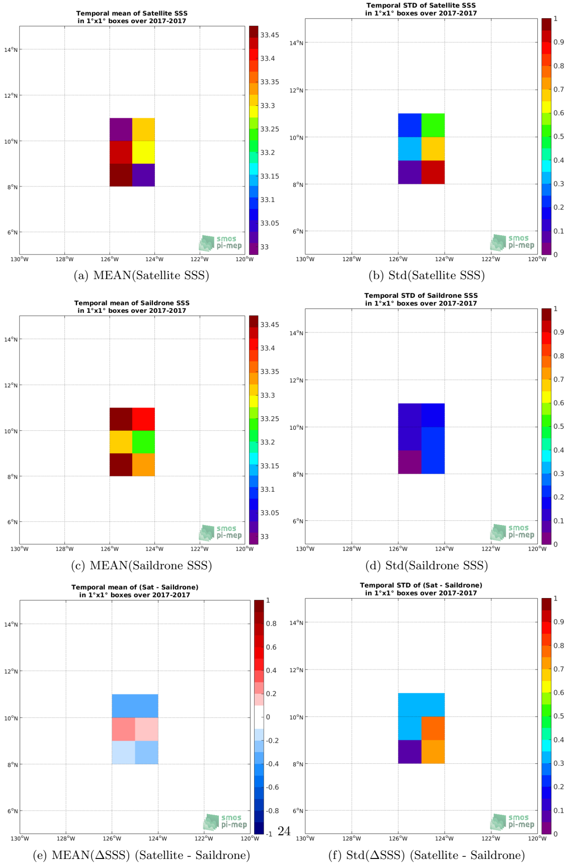
Figure 6: Temporal mean (left) and Std (right) of SSS from SMOS SSS L2 v662 (ESA) (top), Saildrone (middle), and of \Delta SSS (Satellite - Saildrone). Only match-up pairs are used to generate these maps.
