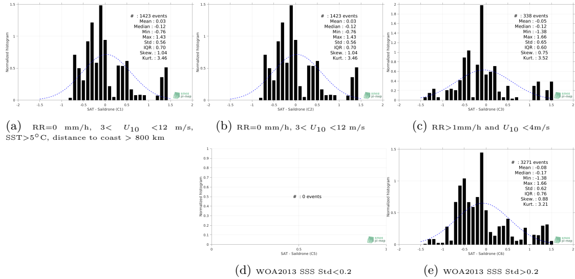
Figure 13: Normalized histogram of \Delta SSS (SMOS SSS L2 v662 (ESA) - Saildrone) for 5 different subdatasets corresponding to: RR=0 mm/h, 3 < U_{10} < 12 m/s, SST > 5°C, distance to coast > 800 km (a), RR=0 mm/h, 3 < U_{10} < 12 m/s (b), RR > 1mm/h and U_{10} < 4 m/s (c), WOA2013 SSS Std < 0.2 (d), WOA2013 SSS Std > 0.2 (e).
