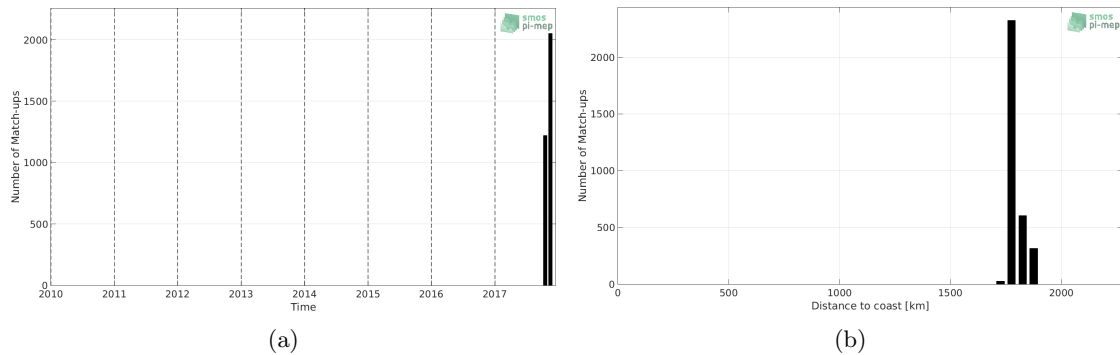
Figure 1: Number of match-ups between Sairdron and SMOS SSS L2 v662 (ESA) SSS as a function of time (a) and as function of the distance to coast (b) over the SPURS 2 Pi-MEP region and for the full satellite product period.
