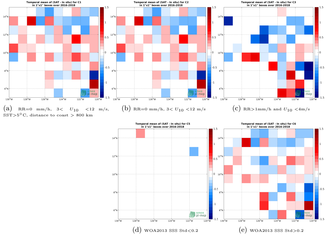
Figure 11: Temporal mean gridded over spatial boxes of size 1^\circ \times 1^\circ of \Delta SSS (SMOS SSS L2 v662 (ESA) - Surface drifters) for 5 different subdatasets corresponding to: RR=0 mm/h, 3 < U_{10} < 12 m/s, SST >5^\circ\text{C} , distance to coast > 800 km (a), RR=0 mm/h, 3 < U_{10} < 12 m/s (b), RR >1 mm/h and U_{10} <4 m/s (c), WOA2013 SSS Std <0.2 (d), WOA2013 SSS Std >0.2 (e).
