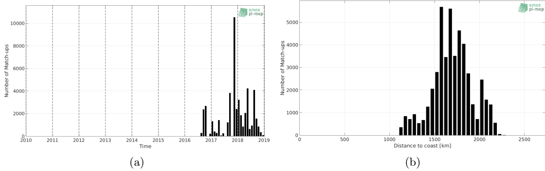
Figure 1: Number of match-ups between Surface drifters and SMOS SSS L2 v662 (ESA) SSS as a function of time (a) and as function of the distance to coast (b) over the SPURS 2 Pi-MEP region and for the full satellite product period.
