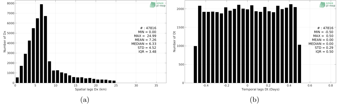
Figure 4: Histograms of the spatial (a) and temporal (b) lags between the location/time of the Surface drifters measurement and the date of the corresponding SMOS SSS L2 v662 (ESA) SSS pixel.
