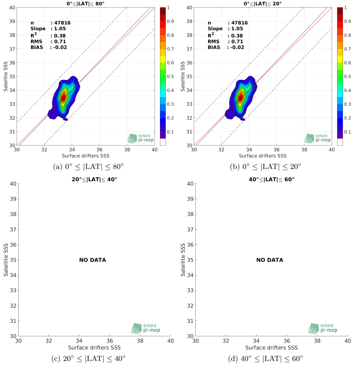
Figure 8: Contour maps of the concentration of SMOS SSS L2 v662 (ESA) SSS (y-axis) versus Surface drifters SSS (x-axis) at match-up pairs for different latitude bands. For each plot, the red line shows x=y . The black thin and dashed lines indicate a linear fit through the data cloud and the \pm 95\% confidence levels, respectively. The number match-up pairs n , the slope and R^2 coefficient of the linear fit, the root mean square (RMS) and the mean bias between satellite and in situ data are indicated for each latitude band in each plots.
