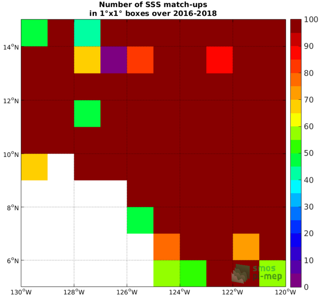
Figure 3: Number of SSS match-ups between Surface drifters SSS and the SMOS SSS L2 v662 (ESA) SSS product for the SPURS 2 Pi-MEP region over 1^\circ \times 1^\circ boxes and for the full satellite product period.
