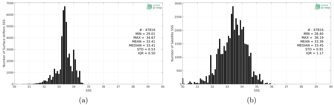
Figure 2: Histograms of SSS from Surface drifters (a) and SMOS SSS L2 v662 (ESA) (b) considering all match-up pairs per bins of 0.1 over the SPURS 2 Pi-MEP region and for the full satellite product period.
