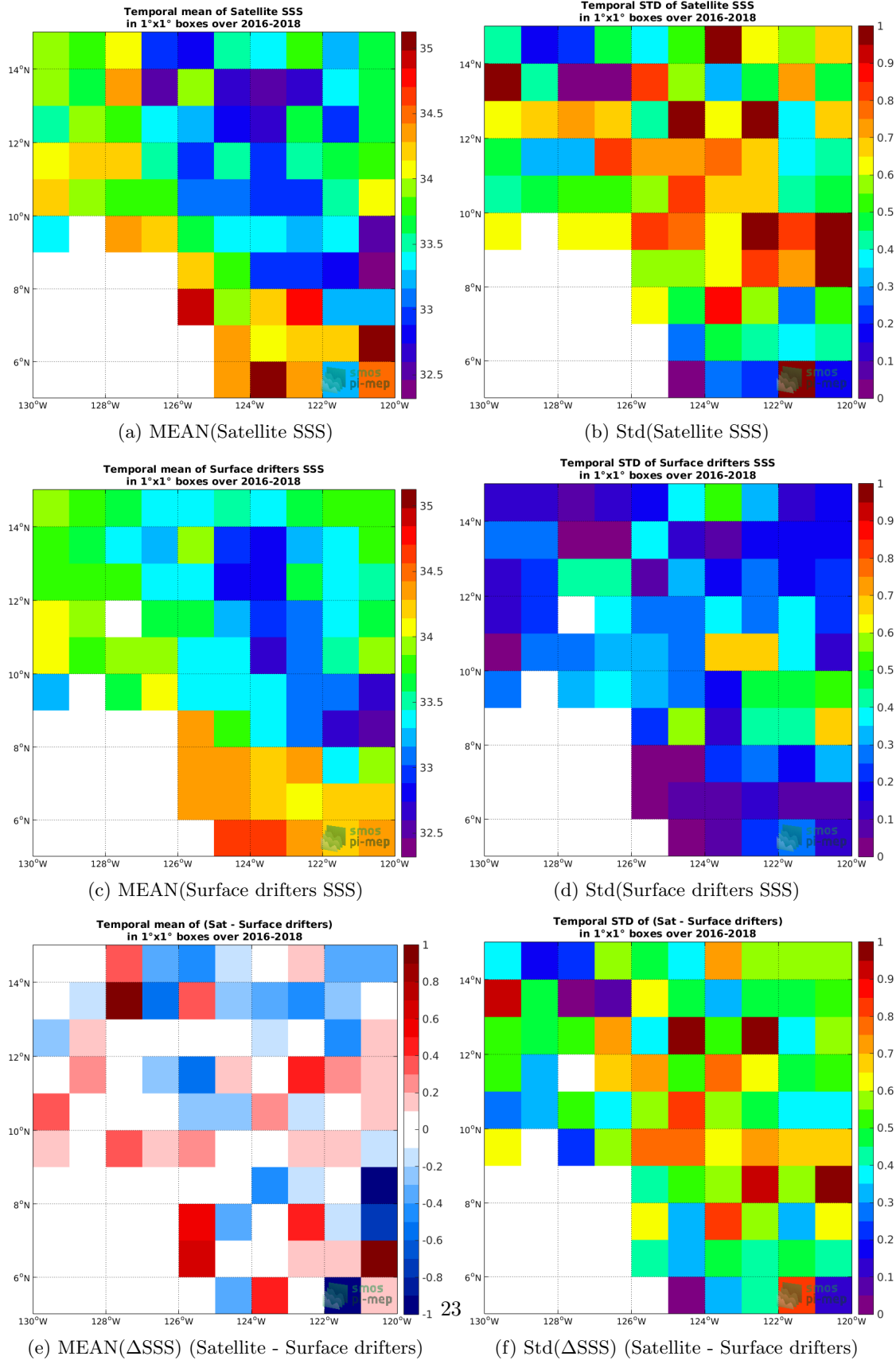
Figure 5: Temporal mean (left) and Std (right) of SSS from SMOS SSS L2 v662 (ESA) (top), Surface drifters (middle), and of \Delta SSS (Satellite - Surface drifters). Only match-up pairs are used to generate these maps.
