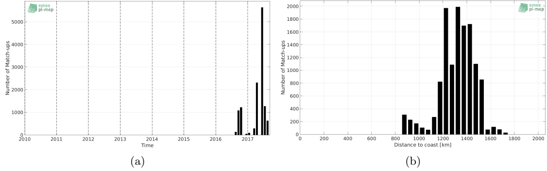
Figure 1: Number of match-ups between Surface drifters and SMOS-L2-DPGS-v662 SSS as a function of time (a) and as function of the distance to coast (b) over the SPURS 2 Pi-MEP region and for the full satellite product period.
