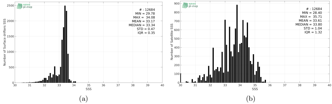
Figure 2: Histograms of SSS from Surface drifters (a) and SMOS-L2-DPGS-v662 (b) considering all match-up pairs per bins of 0.1 over the SPURS 2 Pi-MEP region and for the full satellite product period.
