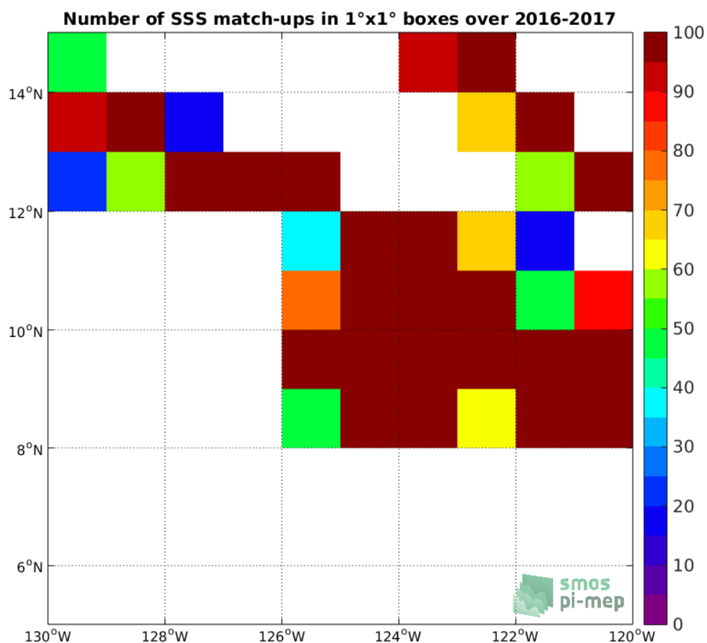
Figure 3: Number of SSS match-ups between Surface drifters SSS and the SMOS-L2-DPGS-v662 SSS product for the SPURS 2 Pi-MEP region over 1°x1° boxes and for the full satellite product period.
