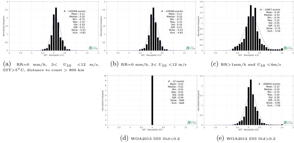
Figure 12: Normalized histogram of \Delta\text{SSS} (SMAP SSS L4 OI v1 - 7 Days (IPRC) - Waveglider) for 5 different subdatasets corresponding to: RR=0 mm/h, 3 < U_{10} < 12 m/s, SST > 5^\circ\text{C} , distance to coast > 800 km (a), RR=0 mm/h, 3 < U_{10} < 12 m/s (b), RR > 1\text{mm/h} and U_{10} < 4\text{m/s} (c), WOA2013 SSS \text{Std} < 0.2 (d), WOA2013 SSS \text{Std} > 0.2 (e).
