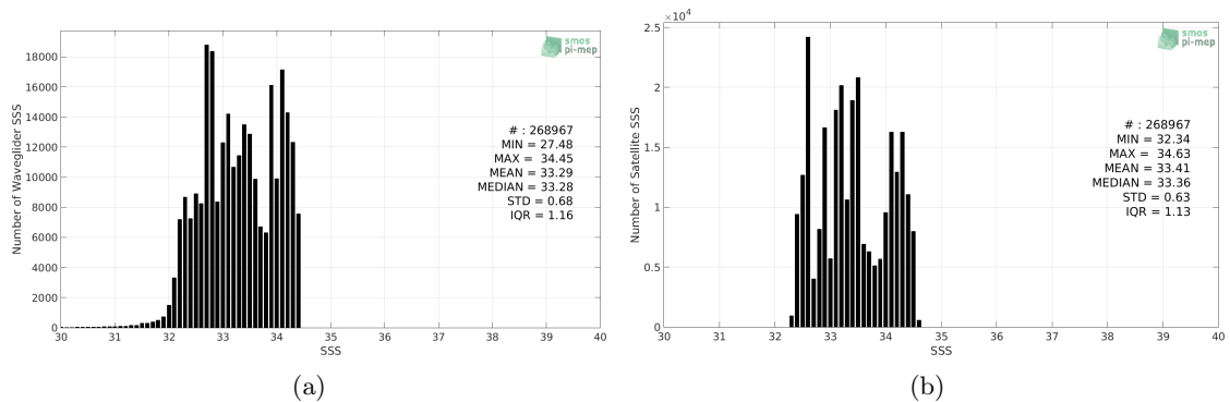
Figure 2: Histograms of SSS from Waveglider (a) and SMAP SSS L4 OI v1 - 7 Days (IPRC) (b) considering all match-up pairs per bins of 0.1 over the SPURS 2 Pi-MEP region and for the full satellite product period.
