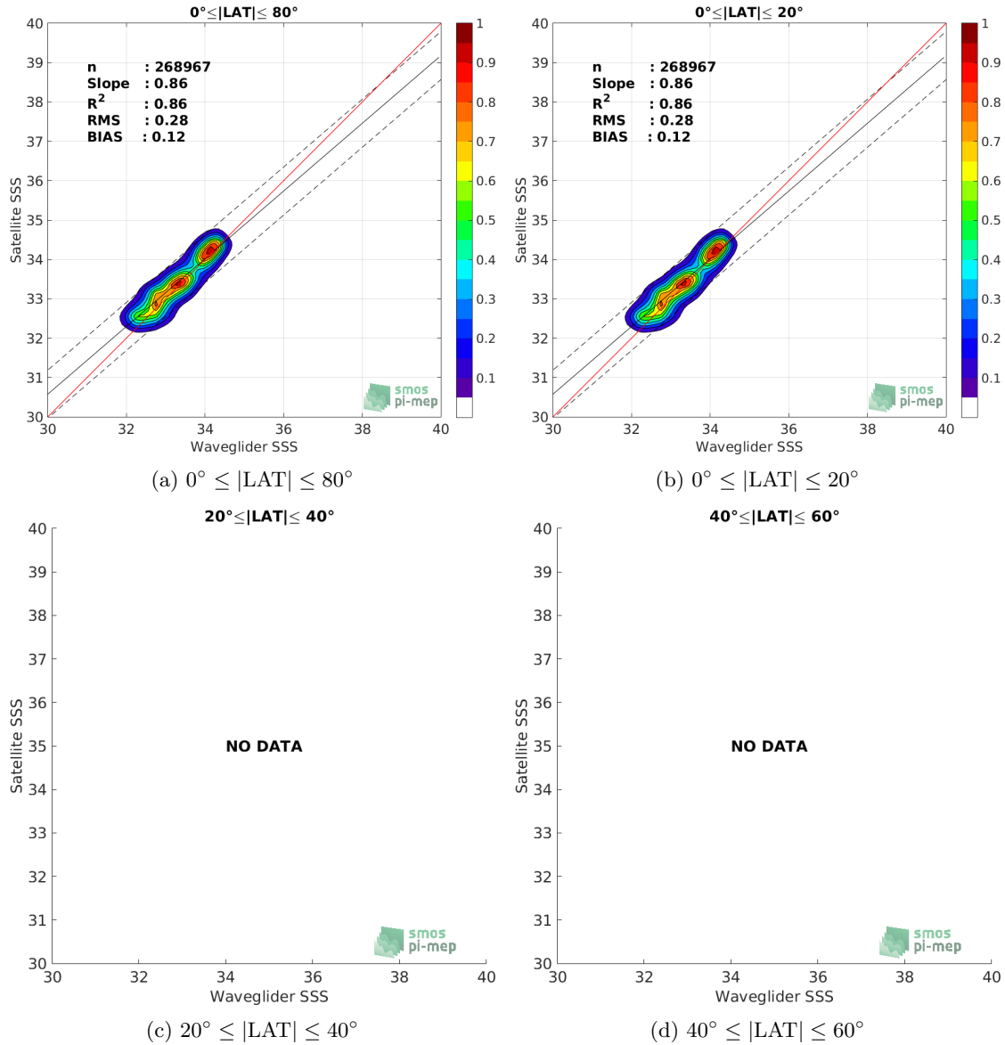
Figure 8: Contour maps of the concentration of SMAP SSS L4 OI v1 - 7 Days (IPRC) SSS (y-axis) versus Waveglider SSS (x-axis) at match-up pairs for different latitude bands. For each plot, the red line shows x=y . The black thin and dashed lines indicate a linear fit through the data cloud and the \pm 95\% confidence levels, respectively. The number match-up pairs n , the slope and R^2 coefficient of the linear fit, the root mean square (RMS) and the mean bias between satellite and in situ data are indicated for each latitude band in each plots.
