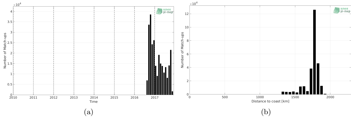
Figure 1: Number of match-ups between Waveglider and SMAP SSS L4 OI v1 - 7 Days (IPRC) SSS as a function of time (a) and as function of the distance to coast (b) over the SPURS 2 Pi-MEP region and for the full satellite product period.
