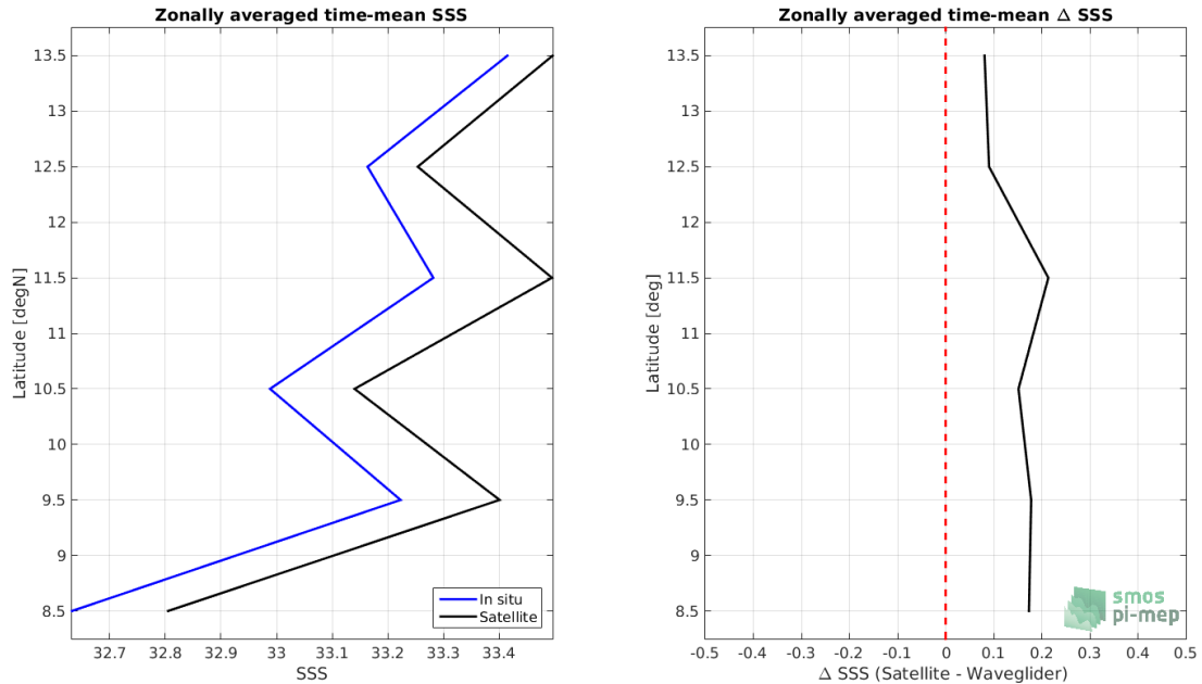
Figure 7: Left panel: Zonal mean SSS from SMAP SSS L4 OI v1 - 7 Days (IPRC) satellite product (black) and from Waveglider (blue). Right panel: Zonal mean of \Delta SSS (Satellite - Waveglider) for all the collected Pi-MEP match-up pairs estimated over the full satellite product period.
