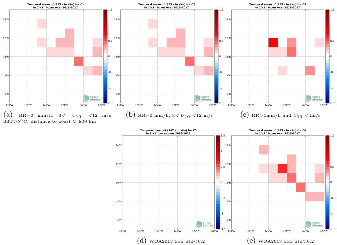
Figure 11: Temporal mean gridded over spatial boxes of size 1^\circ \times 1^\circ of \Delta SSS (SMAP SSS L4 OI v1 - 7 Days (IPRC) - Waveglider) for 5 different subdatasets corresponding to:RR=0 mm/h, 3 < U_{10} < 12 m/s, SST >5^\circ\text{C} , distance to coast > 800 km (a), RR=0 mm/h, 3 < U_{10} < 12 m/s (b), RR >1 mm/h and U_{10} < 4 m/s (c), WOA2013 SSS Std <0.2 (d), WOA2013 SSS Std >0.2 (e).
