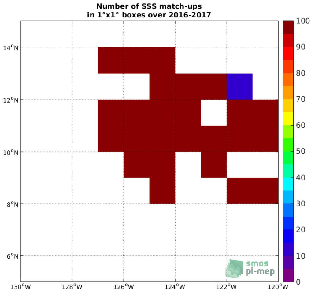
Figure 3: Number of SSS match-ups between Waveglider SSS and the SMAP SSS L4 OI v1 - 7 Days (IPRC) SSS product for the SPURS 2 Pi-MEP region over 1°x1° boxes and for the full satellite product period.
