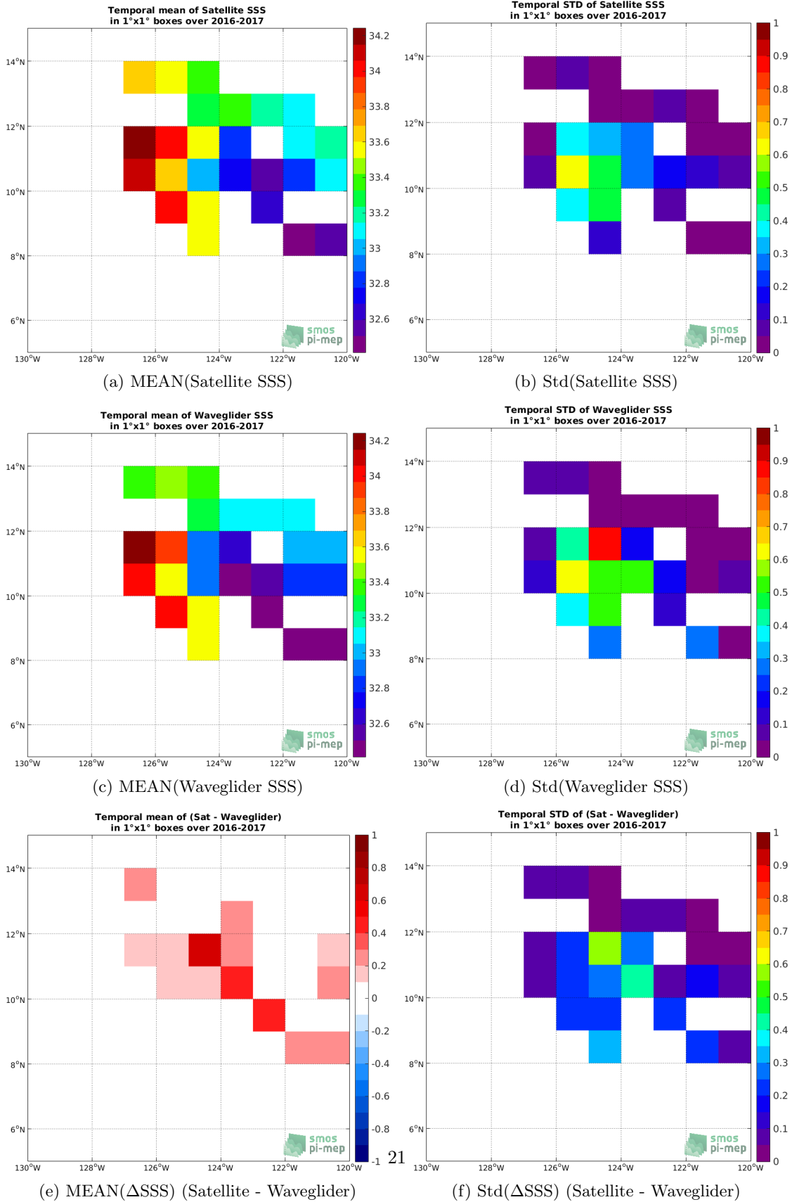
Figure 5: Temporal mean (left) and Std (right) of SSS from SMAP SSS L4 OI v1 - 7 Days (IPRC) (top), Waveglider (middle), and of \Delta SSS (Satellite - Waveglider). Only match-up pairs are used to generate these maps.
