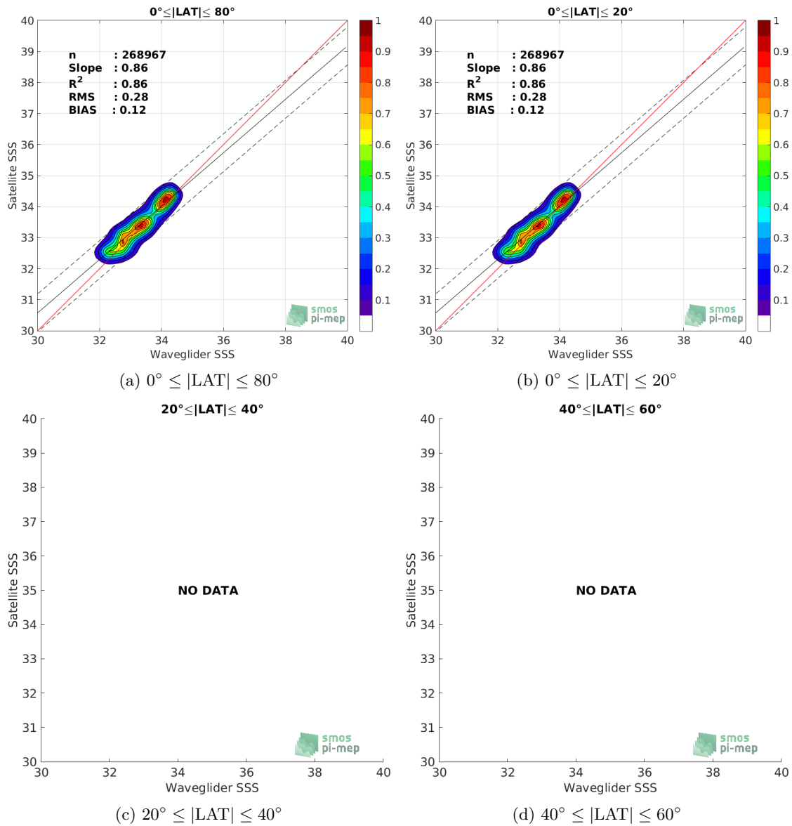
Figure 8: Contour maps of the concentration of SMAP SSS L4 OI v1 - 7day (IPRC) SSS (y-axis) versus Waveglider SSS (x-axis) at match-up pairs for different latitude bands. For each plot, the red line shows x=y . The black thin and dashed lines indicate a linear fit through the data cloud and the \pm 95\% confidence levels, respectively. The number match-up pairs n , the slope and R^2 coefficient of the linear fit, the root mean square (RMS) and the mean bias between satellite and in situ data are indicated for each latitude band in each plots.
