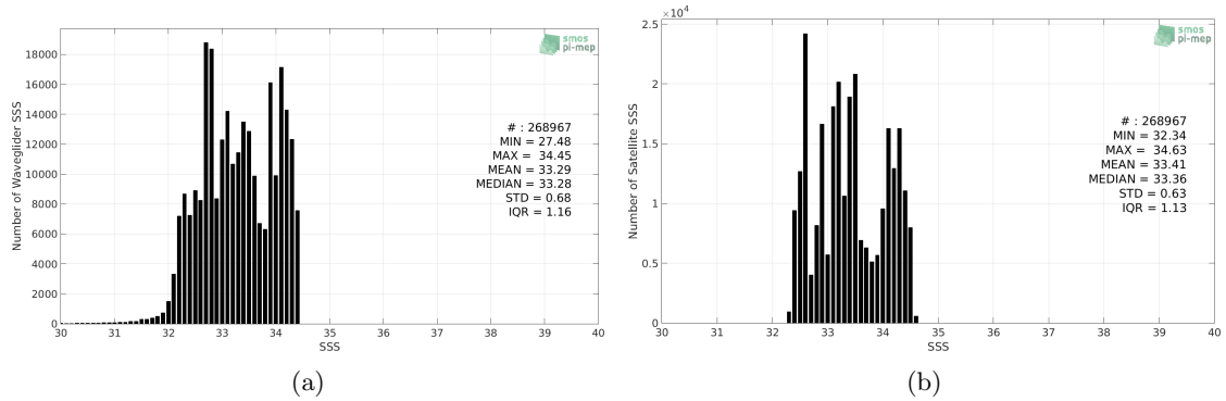
Figure 2: Histograms of SSS from Waveglider (a) and SMAP SSS L4 OI v1 - 7day (IPRC) (b) considering all match-up pairs per bins of 0.1 over the SPURS 2 Pi-MEP region and for the full satellite product period.
