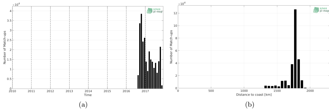
Figure 1: Number of match-ups between Waveglider and SMAP SSS L4 OI v1 - 7day (IPRC) SSS as a function of time (a) and as function of the distance to coast (b) over the SPURS 2 Pi-MEP region and for the full satellite product period.
