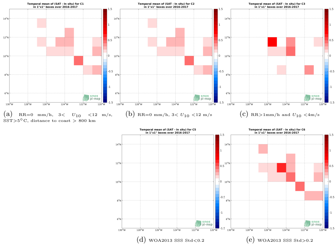
Figure 11: Temporal mean gridded over spatial boxes of size 1^\circ \times 1^\circ of \Delta SSS (SMAP SSS L4 OI v1 - 7day (IPRC) - Waveglider) for 5 different subdatasets corresponding to:RR=0 mm/h, 3 < U_{10} < 12 m/s, SST >5^\circ\text{C} , distance to coast > 800 km (a), RR=0 mm/h, 3 < U_{10} < 12 m/s (b), RR >1 mm/h and U_{10} < 4 m/s (c), WOA2013 SSS Std <0.2 (d), WOA2013 SSS Std >0.2 (e).
