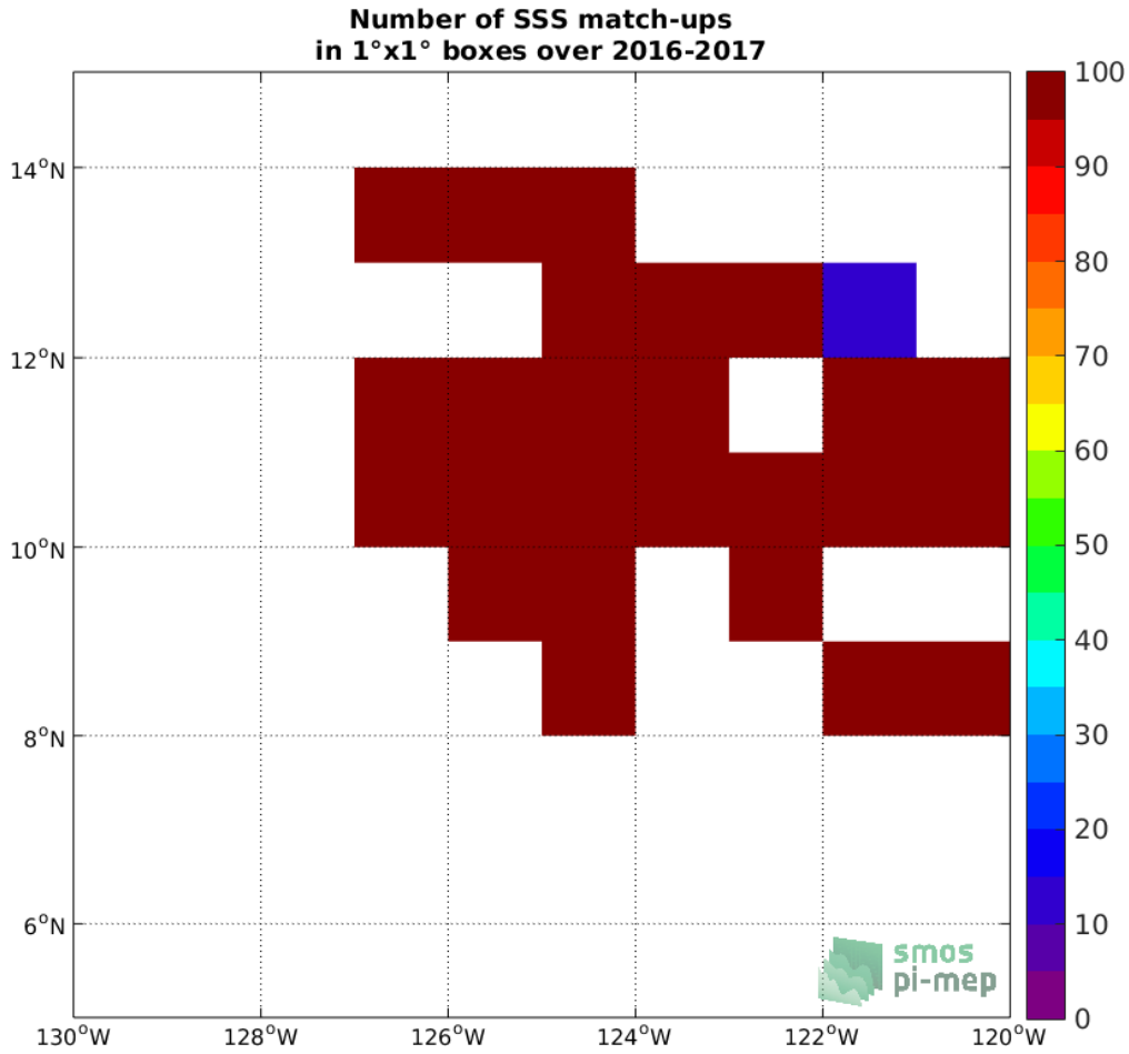
Figure 3: Number of SSS match-ups between Waveglider SSS and the SMAP SSS L4 OI v1 - 7day (IPRC) SSS product for the SPURS 2 Pi-MEP region over 1^\circ \times 1^\circ boxes and for the full satellite product period.
