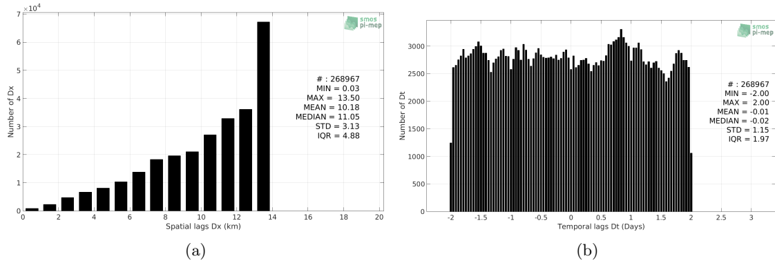
Figure 4: Histograms of the spatial (a) and temporal (b) lags between the location/time of the Waveglider measurement and the date of the corresponding SMAP SSS L4 OI v1 - 7day (IPRC) SSS pixel.
