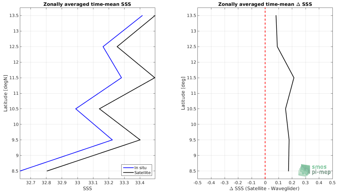
Figure 7: Left panel: Zonal mean SSS from SMAP SSS L4 OI v1 - 7day (IPRC) satellite product (black) and from Waveglider (blue). Right panel: Zonal mean of \Delta SSS (Satellite - Waveglider) for all the collected Pi-MEP match-up pairs estimated over the full satellite product period.
