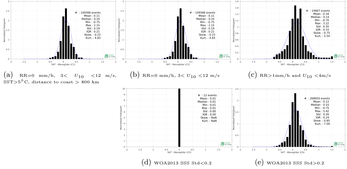
Figure 12: Normalized histogram of \Delta SSS (SMAP SSS L4 OI v1 - 7day (IPRC) - Waveglider) for 5 different subdatasets corresponding to: RR=0 mm/h, 3 < U_{10} < 12 m/s, SST>5°C, distance to coast > 800 km (a), RR=0 mm/h, 3 < U_{10} < 12 m/s (b), RR>1mm/h and U_{10} < 4 m/s (c), WOA2013 SSS Std<0.2 (d), WOA2013 SSS Std>0.2 (e).
